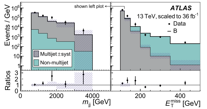
Fig. 3. Distribution of event yields in the multijet validation region for m_{jj} (left) and E_T^{\text{miss}} (right). The m_{jj} plot shows the 100 < E_T^{\text{miss}} < 120 GeV subset of the right plot as indicated by the arrow. The N observed data (dots) are superimposed on the sum of the B backgrounds (stacked histogram). The systematic uncertainty band applies only to the multijet component. The statistical uncertainties are relatively large because of the weighting of the trigger samples with large prescale values. See the caption of Fig. 2 for other plotting details.
