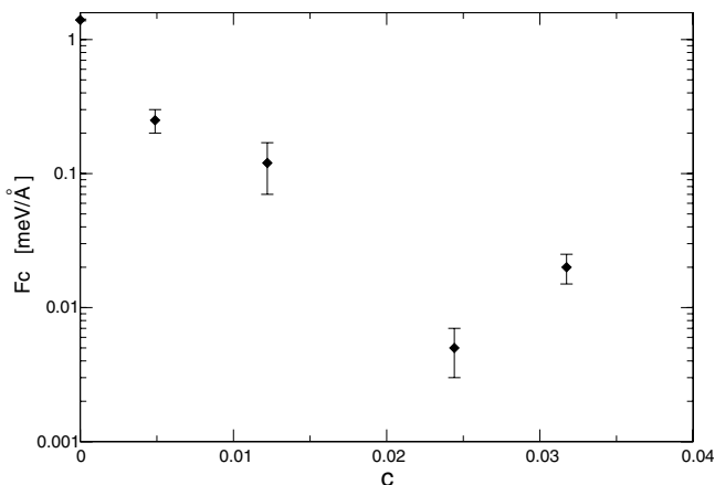
Fig. 5. The effective depinning force F_c as a function of the concentration of vacancies. The depinning force has been obtained as the value of the force for which half of N_r = 10 different configurations depin after a time t_e = 10^{-7} s. The error bar is estimated considering the forces for which the fraction of depinned configurations lies between p = 0.2 and p = 0.8 .
