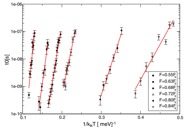
Fig. 1. The activation time as a function of the inverse temperature for different applied lateral forces. The linear behavior in a semilogarithmic plot implies Arrhenius behavior. The slope of the lines yields an estimate of the energy barrier as a function of the applied force.
