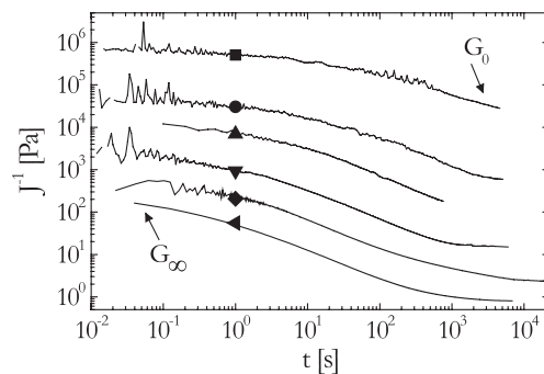
FIG. 2. Representative examples of the time evolution of the inverse compliance J(t)^{-1} obtained in creep experiments using stresses that are well within the linear regime. The responses are measured after a quench to T = 10^\circ\text{C} for \phi = 0.171 (filled square), 0.149 (filled circle), 0.13 (filled upward triangle), 0.11 (filled downward triangle), 0.093 (filled diamond), and 0.075 (filled left side triangle).
