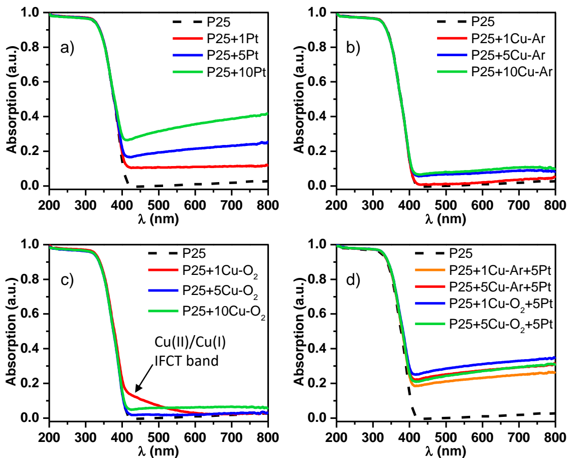
Figure 2. Absorption spectra of the a) P25+xPt, b) P25+xCu-Ar, c) P25+xCu-O 2 , (x = 1, 5 and 10 min); d) Cu and Pt co-modified photocatalyst series, all compared the absorption spectrum of bare P25 TiO 2 (dashed black line).
