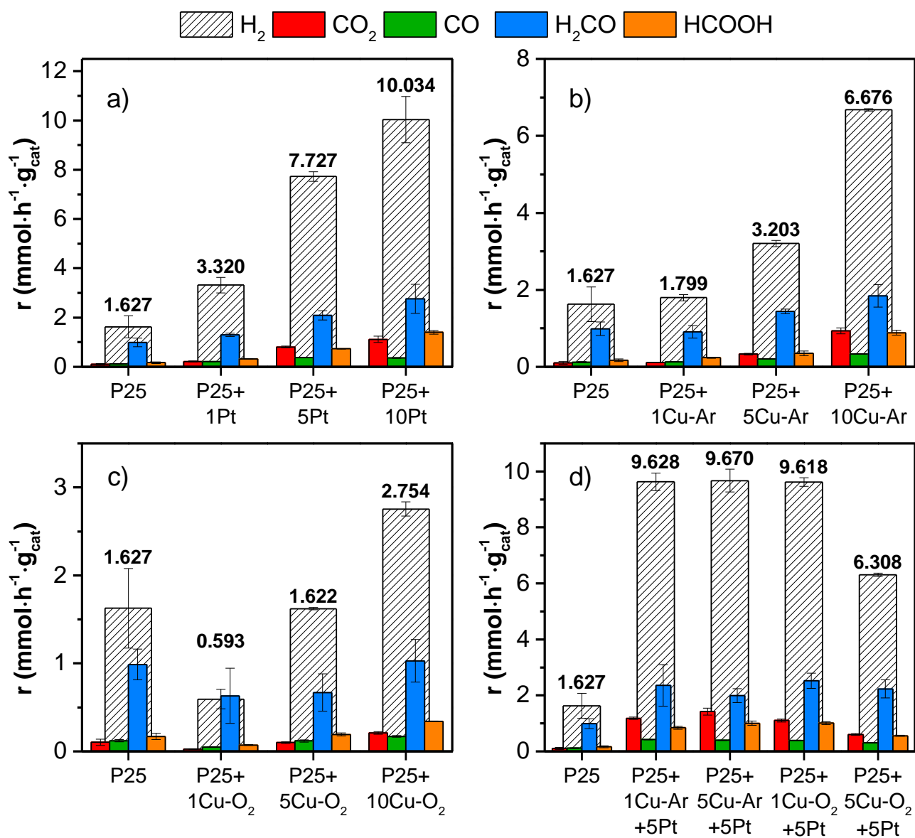
Figure 6. Hydrogen and by-products production rates obtained with (a) Pt-modified \text{TiO}_2 , (b) Ar-sputtered Cu-modified \text{TiO}_2 , (c) Ar/ \text{O}_2 -sputtered Cu-modified \text{TiO}_2 , (d) Pt and Cu co-modified \text{TiO}_2 , compared to bare, unmodified P25 \text{TiO}_2 .
