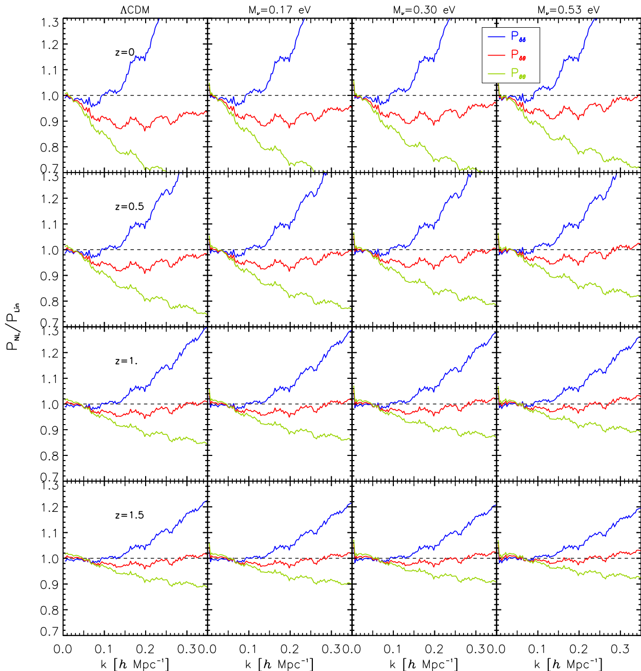
Fig. 3. Ratio between nonlinear (measured) P_{NL} and the linear (predicted) P_{Lin} power spectra in the \Lambda CDM case ( \Sigma m_\nu = 0 ) and for the three neutrino masses ( \Sigma m_\nu = \{0.17, 0.3, 0.53\} eV). The density–density, density–velocity divergence, and velocity divergence–velocity divergence spectra are represented by blue solid, red short dashed, and green long dashed lines, respectively. Each row shows the redshift evolution of these ratios (from top to bottom z = 0, 0.5, 1 , and 1.5 .)
