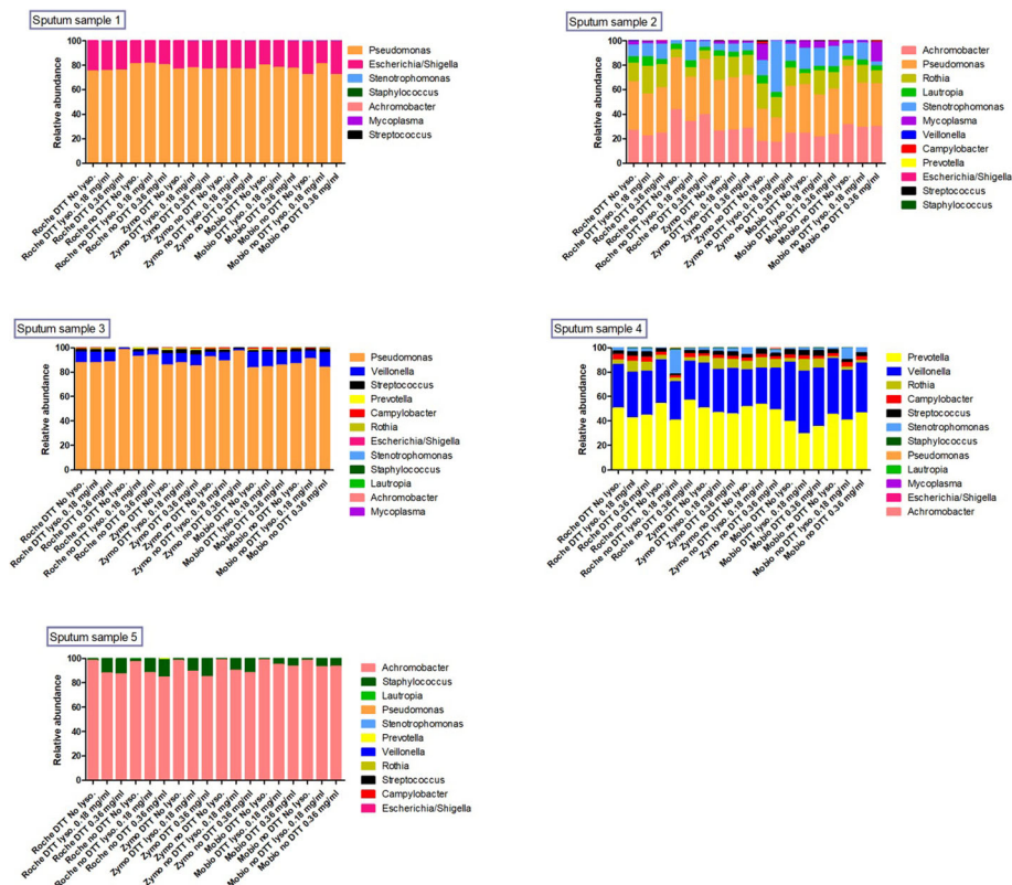
Fig. 5 Relative abundances of bacterial genera in each of the 5 sputum samples across the 18 evaluated conditions
