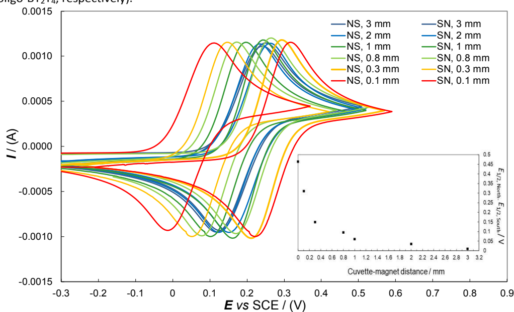
Figure 3. CV patterns recorded at 0.05 V s -1 for the Fe(III)/Fe(II) achiral couple in aqueous solution at hybrid ITO|oligo-(S)-BT 2 T 4 interface, as a function of the applied magnetic field orientation (north-south vs south-north) and of the magnetic field strength.
