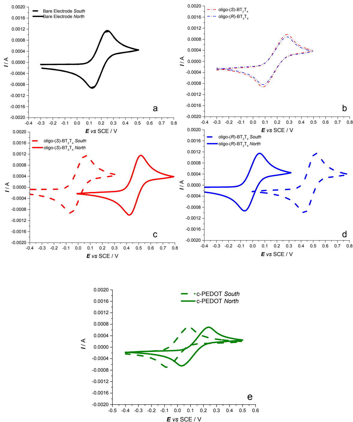
Figure 2. CV patterns recorded at 0.05 \text{ V s}^{-1} for the Fe(III)/Fe(II) achiral couple: (a) on bare ITO electrode, as a function of the magnetic field orientation (solid line for north pole towards electrode, dashed line for south pole); (b) on hybrid ITO|oligo-BT 2 T 4 electrodes (blue line for (R)-configuration, red for (S)-) without the external magnet; (c) e (d) at hybrid ITO|oligo-BT 2 T 4 interface, as a function of the applied magnetic field orientation (solid vs dashed lines, same color legend as before for the film configuration); (e) at hybrid ITO|c-PEDOT interface (same legend for magnetic field orientation).
