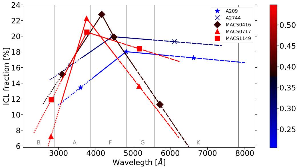
Figure 2. ICL fractions yielded by CICLE for our subsample of merging clusters at rest-frame wavelength. Lines are color-coded by redshift, and different styles are used to represent the wavelength range covered by each one of the three filters: dotted for the F435W filter, solid for the F606W filter, and dashed for the F814W filter. Vertical gray lines separate the wavelength intervals where the emission peaks of the different stellar spectral types are included, as indicated at the bottom of each region.
