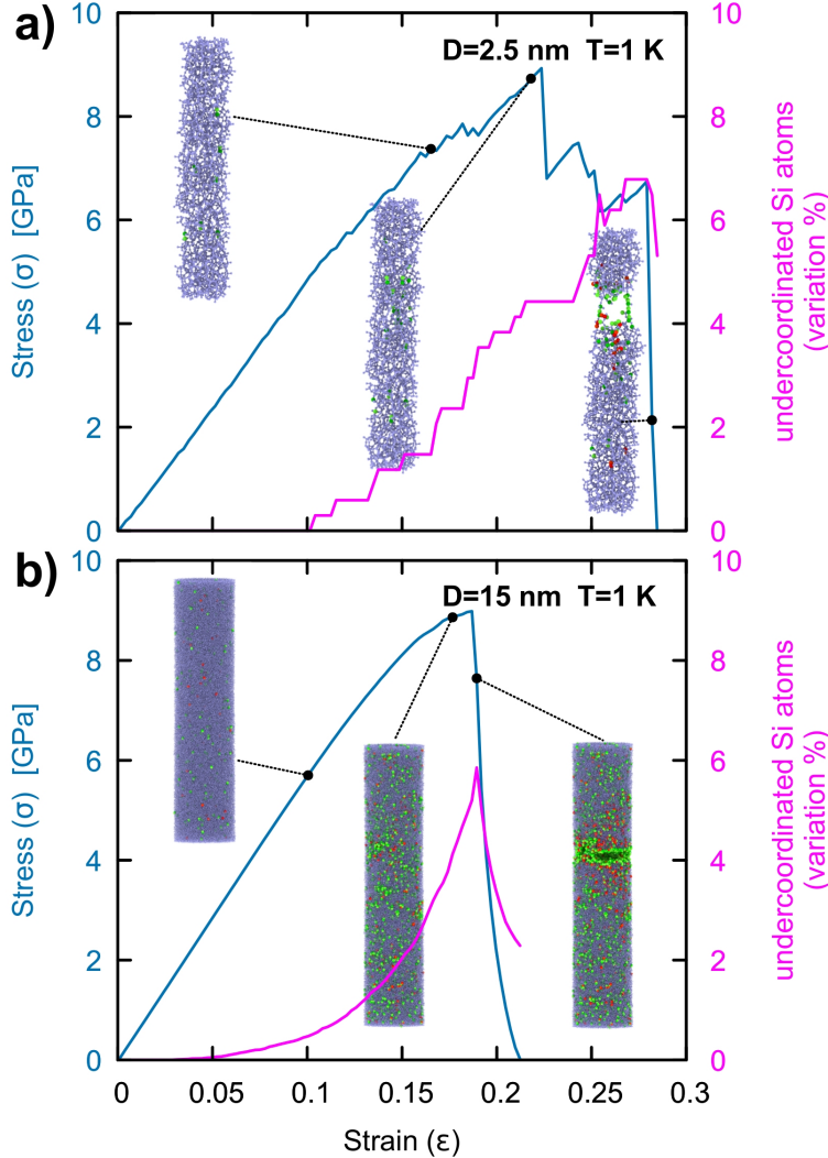
Figure 3: Coordination and damage accumulation in obc samples at 1 K – Stress (blue) and percent variation of the number of undercoordinated Si atoms (magenta) as a function of the applied strain for cylindrical nanofibers with (a) D=2.5 nm and (b) D=15 nm. Snapshots report in green and red the dynamically broken and newly formed (or reformed) bonds, respectively (see SI Movie 3 and 4 for full animations).
