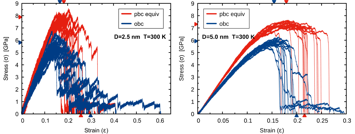
Figure 5: Stress-strain curves comparison at 300 K – Stress strain curves of obc and pbc samples with D = 2.5 nm (left panel) and D = 5 nm (right panel) at T = 300 K. Triangles at left, top, and bottom axes report \sigma^* , \epsilon^* , and \epsilon_{\text{tot}} , respectively, averaged over 32 runs (16 shown).
