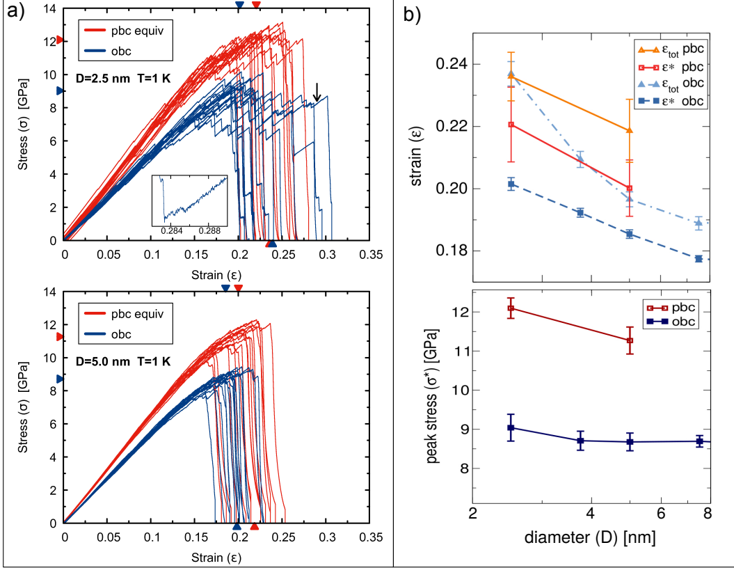
Figure 2: Obc and pbc comparison for small sample sizes at 1 K – (a) Stress strain curves of obc and pbc samples with D=2.5 nm (top panel) and D=5 nm (bottom panel) at T=1 K. Triangles at left, top, and bottom axes report \sigma^* , \epsilon^* , and \epsilon_{\text{tot}} , respectively, averaged over 100 runs (16 shown). The inset in top panel is a magnification of the region pointed by the arrow. (b) Average values comparison as a function of size: (top panel) strain at peak \epsilon^* and rupture strain \epsilon_{\text{tot}} , and (bottom panel) peak stress \sigma^* .
