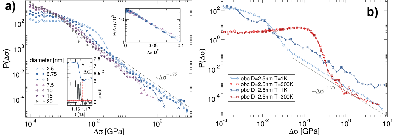
Figure 4: Stress-drops distributions – (a) P(\Delta\sigma) for different sample sizes with obc. The main plot shows a power law distribution P(\Delta\sigma) \sim \Delta\sigma^{-\tau} for the larger \Delta\sigma with exponent \tau \sim 1.75 ; (upper inset) Lin-log plot of the \Delta\sigma \rightarrow \Delta\sigma D^2 scaling, showing a collapse of the distributions for small stress drops; (lower inset) example of stress drop and its derivative, alternative thresholds are also showed. (b) Stress-drops distribution for different temperatures and boundary conditions for the smallest system size.
