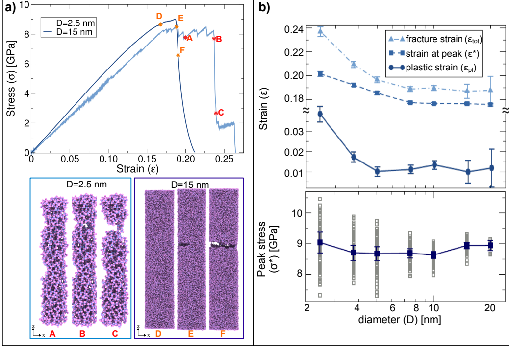
Figure 1: Brittle-to-ductile crossover as the sample size is reduced – (a) (top) Stress-strain curves of two typical samples of diameter D=2.5 nm and D=15 nm, and (bottom) snapshots of the same nanofibers during the deformation at configurations marked by labels on the corresponding stress curves. (Violet spheres: Si atoms, pink spheres: O atoms. Arbitrary scale). See SI Movie 3 and 4 for full animations. (b) (top) Deformation up to peak stress \epsilon^* \equiv \epsilon(\sigma_{max}) , total deformation \epsilon_{tot} before fracture, plastic deformation \epsilon_{pl} \equiv (\epsilon_{tot} - \epsilon^*) , and (bottom) the average maximum stress \sigma^* as a function of the sample diameter. In the latter, scattered symbols show the \sigma^* value of each individual sample, while blue squares correspond to the average.
