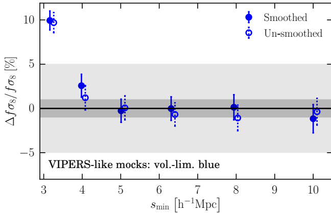
Fig. B.1. Impact of the smoothing of the data covariance matrix on the systematic errors on f_{s8} (filled circles, same as the filled blue circles in Fig. 13) when fitting the auto-correlation function of luminous blue galaxies in VIPERS-like mock samples. Measurements obtained using the raw estimates of the data covariance matrix are also shown as empty circles. In both cases error bars give the errors on the mean of the 153 mock samples. Fits are performed using the Scoccimarro model.
