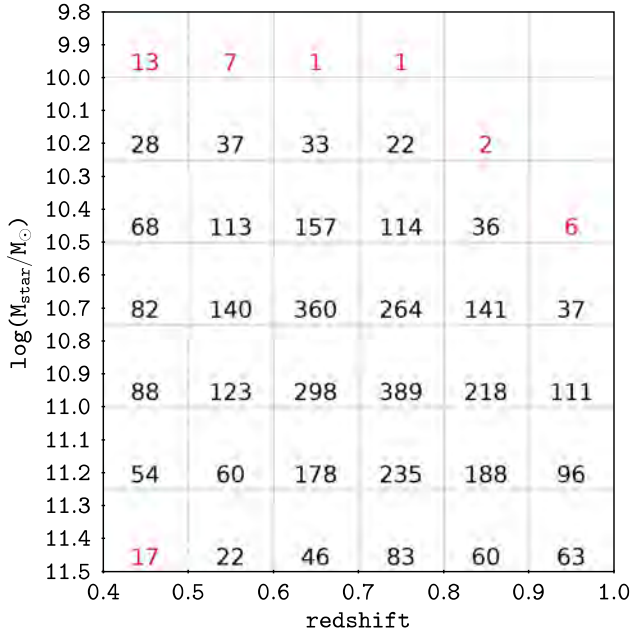
Fig. 3. Final numbers of VIPERS spectra of passive red galaxies for different redshift and stellar mass bins. Bins with insufficient number of galaxies ( <20 ), shown in red, are not used in the following analysis.
