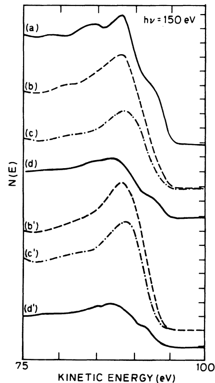
FIG. 4. Si L_{2,3} line shapes for Si(111) and Si+Cu. (a) Si+15 Å Cu, fully mixed. (b) Line shape for Si+4 Å Cu. (b') Line shape for Si+2 Å Cu. (c) (c') Line shape for pure Si attenuated. (d), (d') Difference curve-s: line-shape contribution from Si mixed reacted with Cu at \theta = 4 Å and \theta = 2 Å.
