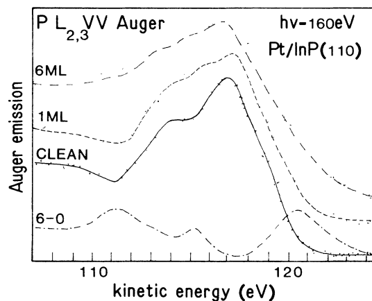
FIG. 4. Auger P L_{2,3} VV line shapes as measured with h\nu=160 eV excitation, for clean InP(110) (solid curve), and for 1 ML Pt/InP(110) and for 6 ML Pt/InP(110). The dot-dashed curve at the bottom is the difference curve between the 6 ML and the clean spectra. A three-peaked structure is obtained with the three peaks being separated by \sim 4.5 eV similarly to the peaks of 3s , 3p bonding and 3p antibonding states in the hybridized valence-band DOS.
