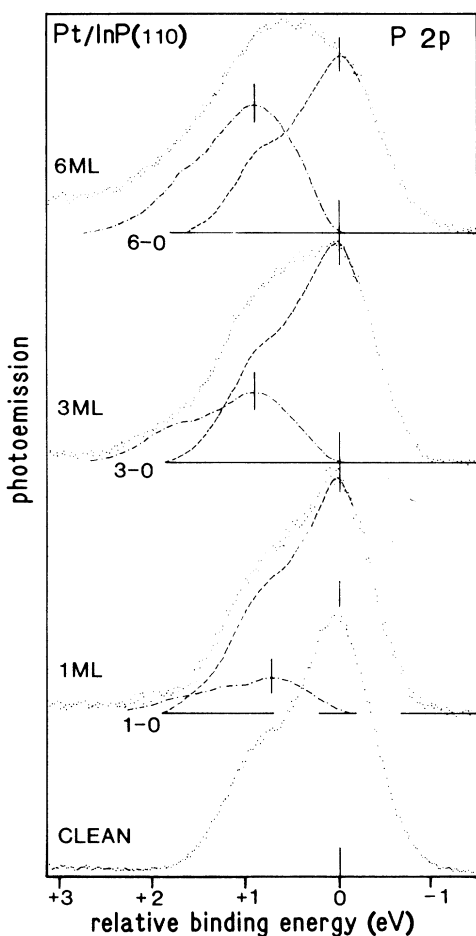
FIG. 5. P 2p core-level photoemission spectra for the clean-InP(110) surface, and for 1, 3, and 6 Pt monolayers on InP(110). The spectra have been aligned on the lowest-binding-energy edge and subtraction between the interface spectra and the clean substrate spectrum are shown as dot-dashed curves. The subtraction results show a single extra P 2p doublet, shifted by 0.85 \pm 0.1 eV towards higher binding energies in the case of 3 and 6 ML. The chemical shift at 1 ML is 0.55 \pm 0.1 eV.
