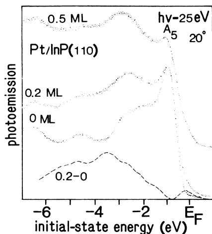
FIG. 1. Angular resolved electron-energy-distribution curves (EDC's) measured at 20^\circ off normal in the [110] direction to enhance the sensitivity to the P A_5 surface state. The bottom curve corresponds to the clean-InP(110) surface, but has been shifted by the Schottky barrier value (see text) in order to align the surface-state peak with the curves for 0.2 and 0.5 monolayers of Pt on InP(110). The dashed curve is the difference between the 0.2 and the clean (shifted) InP. It is representative of the distribution of the interface states.
