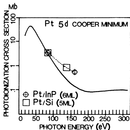
FIG. 8. Cooper-minimum curve of the photoionization cross section of the Pt 5d subshell. The solid curve represents the Hartree-Fock-Slater calculation of Ref. 15. The experimental data for reacted Pt/Si (Ref. 19) and Pt/InP interfaces are arbitrarily normalized at the h\nu=80 eV value to the theoretical atomic value. This allows to observe the reduction of the magnitude of the CM effect for the hybridized Pt 5d states of the interface compounds with respect to the localized Pt 5d atomic states.
