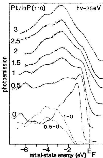
FIG. 2. Photoelectron EDC's excited with h\nu=25 eV and measured at normal emission for clean-InP(110) and Pt coverages as indicated. The dashed and dot-dashed curves represent the difference spectra between the 0.5 and 1 ML curves and the clean (energy shifted of the Schottky barrier value) curve. The Pt derived states are spread over a wide energy range.
