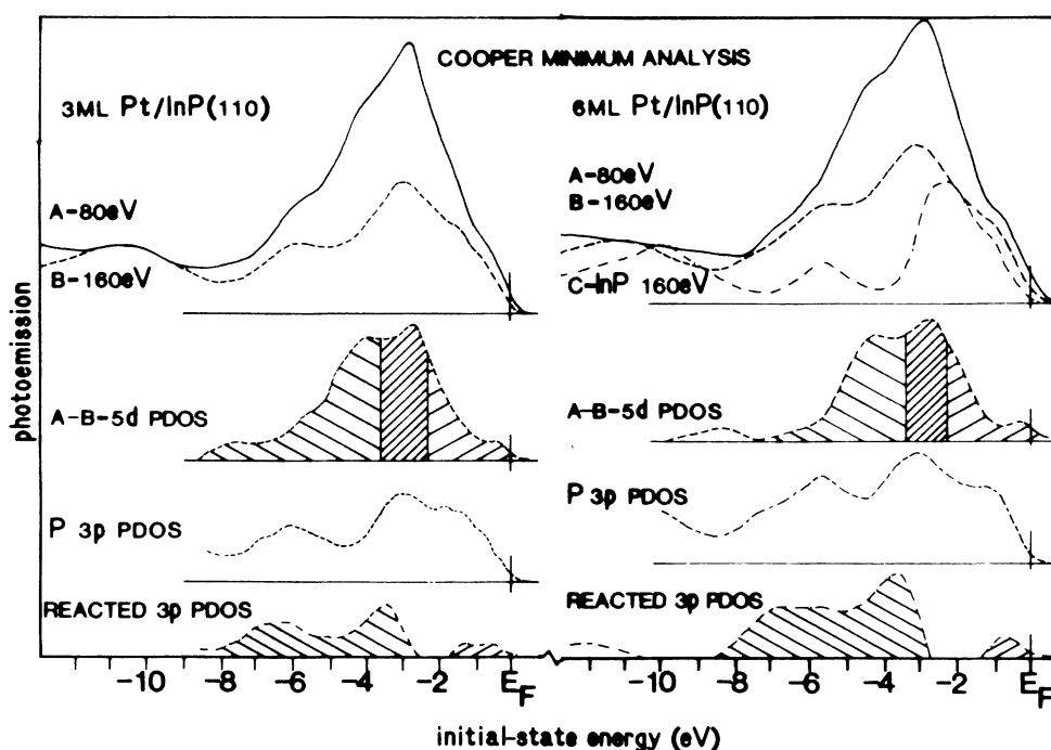
FIG. 9. Cooper-minimum analysis for the 3 ML (left panel) and 6 ML (right panel) Pt/InP(110) interface. The top (solid) curve in both panels is the EDC obtained with h\nu=80 eV, the dashed curve normalized to it at -11 eV is the Cooper-minimum curve obtained with h\nu=160 eV; the dot-dashed curve normalized at -11 eV, in the right panel, is the EDC for clean InP(110) as obtained with h\nu=160 eV. The second-level curves from the top down are the difference curves between the h\nu=80 eV and the Cooper-minimum spectra; they represent the d partial density of states. The central fine-dashed region is the region of the spectrum which undergoes the strongest Cooper-minimum effect (see Fig. 8). The third-level curves from the top down represent the Cooper-minimum curve reduced by the residual d contribution still present at the Cooper minimum, estimated according to Table I. The d contribution has been eliminated by subtracting the proper amount of the d PDOS line shape. This curve is an indicator of the averaged P 3sp PDOS at the interface, i.e., both from the ioniclike or unreacted InP and from the P-Pt phase. The bottom difference curves are indicators of the interface P-Pt PDOS of P 3p character: They are obtained by subtracting from the total P 3p DOS an amount of clean-InP(110) line shape which is calibrated by the relative weight of reacted-unreacted P 2p core-level photoemission peaks. By comparing the DOS peaks in the Pt 5d PDOS and P 3sp PDOS it is plausible to attribute the DOS features between -3 and -8 eV to bonding d - p hybrid states, and the DOS peaks between -2 and E_F to the partially occupied antibonding states. It is noteworthy that in correspondence with the more localized Pt 5d states, between -3.5 and -2.5 eV there is a gap (or a minimum) of P 3sp DOS.
