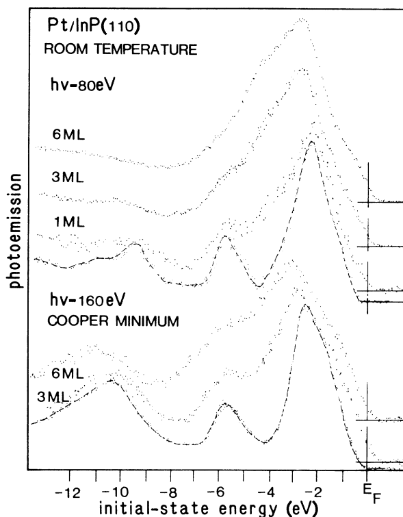
FIG. 3. Normal emission EDC's obtained with h\nu=80 eV and at the Cooper minimum ( h\nu=160 eV) for cleaved InP(110) (dashed curves) and for Pt coverages onto InP(110). These spectra allow the experimental derivation of the d -like PDOS and p -like PDOS at the interface, as detailed in Figs. 5 and 6.
