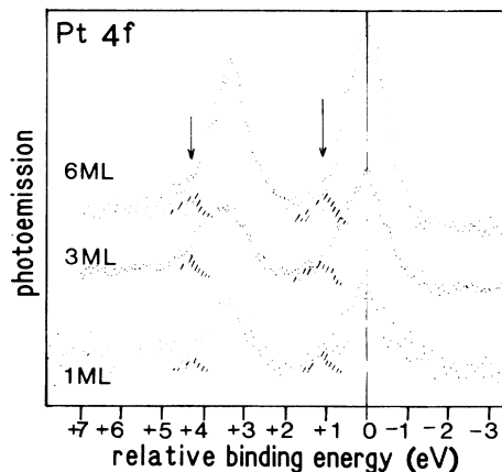
FIG. 7. Pt 4f core-level photoemission as a function of the Pt coverage. The spectra are aligned at the 4f_{7/2} peak; the minor doublet at 1 eV higher energy is shown by the dashed areas.
