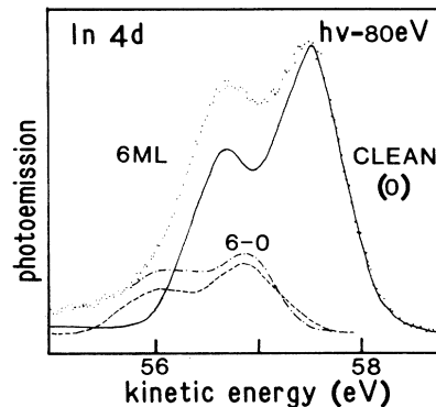
FIG. 6. In 4d core levels spectrum for 6 ML Pt/InP(110) (dots). The line shape of In 4d from cleaved InP(110) (solid line) is shifted to match the lower energy edge of the interface In 4d signal. The difference between the two spectra show a single extra doublet (dot-dashed). A second In 4d line shape from clean InP (dashed) is compared to the difference curve. The higher intensity in the high-energy tail of the interface spectrum can be attributed to a Sunjic-Doniach effect due to the metallic character of at least one of the In environments at the 6 ML interface (on this point the peak decomposition procedure is intrinsically ambiguous). The main component of the In 4d emission is shifted by 0.7 \pm 0.1 eV towards lower-binding energies, i.e., towards a bulk-In binding energy, this is likely to be the metallic-In phase. The same result is obtained for 3 ML Pt/InP(110).
