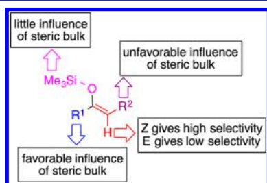
Figure 8. Composite influence of substrate shape on selectivity.
