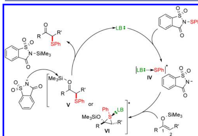
Figure 4. Proposed catalytic cycle.
