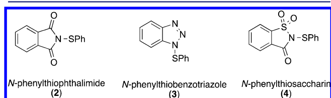
Figure 1. Sulfenylating agents.
