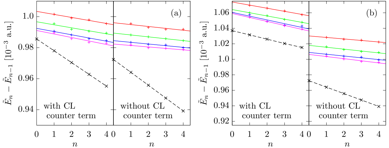
FIG. 7. Shift of the eigenenergies of a MO coupled to a resonant CL bath with parameters \omega_{\max} = \omega_s , \omega_c = 0.5 \omega_s , and coupling strengths \eta_{\text{eff}} = 0.1 in panel (a) and \eta_{\text{eff}} = 0.5 in (b). All plot specifications as in Fig. 5, with the addition of results for 60 bath DOFs (magenta crosses).
