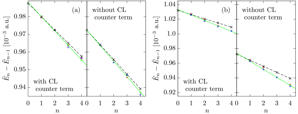
FIG. 6. Birge-Sponer fit to the difference of consecutive eigenenergies \tilde{E}_n of a Morse oscillator coupled to the off-resonant CL bath from Fig. 5. The “+” crosses denote results with 10 (red), 20 (green), and 40 (blue) bath HOs. The solid green line is a linear fit to the 20 DOFs result, and the dashed black line with “x” crosses is the corresponding 1D MO reference, i.e., E_n - E_{n-1} (Eq. (21)) or E_{\text{mod},n} - E_{\text{mod},n-1} (Eq. (32)), respectively.
