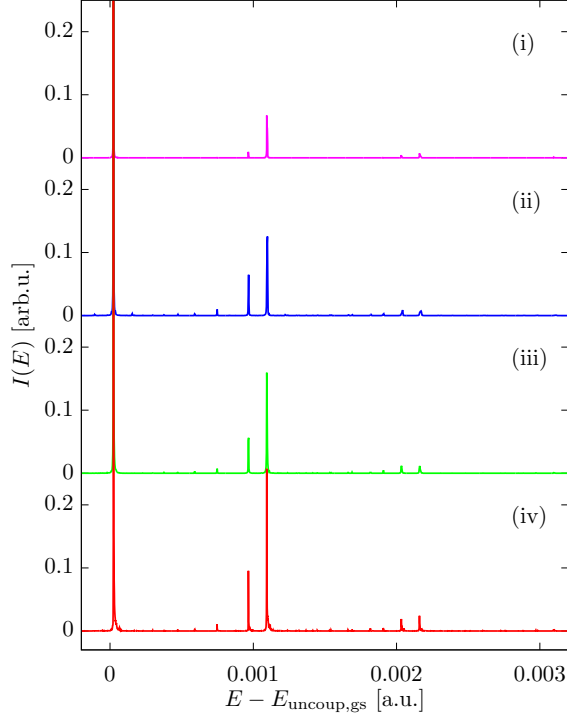
FIG. 1. Spectrum of an iodine-like Morse oscillator coupled to a CL bath comprising 10 DOFs with \omega_{\max} = \omega_s , \omega_c = 0.5 \omega_s and coupling \eta_{\text{eff}} = 0.5 . From top to bottom: separable TA mixed with 1 HK DOF (magenta, (i)) (Eq. (19)), full TA mixed with 1 HK DOF (blue, (ii)) and full TA mixed with 2 HK DOFs (green, (iii)) (Eq. (13)), and the separable TA HK (red, (iv)) using Eq. (6). All spectra are renormalized such that the elastic peak has height one, and all spectra are magnified and overlapped in order to make excited peaks visible.
