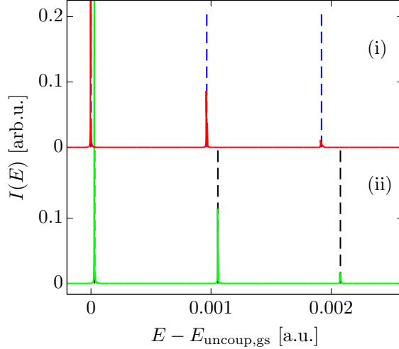
FIG. 3. Spectra for a Morse oscillator in an off-resonant CL bath with 20 HOs. Bath parameters are \omega_c = 0.1 \omega_s , \omega_{\max} = 0.5 \omega_s , and \eta_{\text{eff}} = 0.5 . The top result (i) is from a calculation without the CL counter term, the bottom spectrum (ii) from a calculation including the CL counter term. The dashed lines represent eigenvalues of a regular 1D Morse potential (blue, top) and of a 1D Morse potential modified by the CL counter term according to Eq. (32) (black, bottom).
