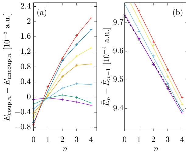
FIG. 9. Cutoff frequency dependence of the shift of the eigenenergies of a Morse oscillator coupled to a CL bath. Bath parameters: 20 HOs, maximum frequency fixed at \omega_{\text{max}} = 0.7 \omega_s , and cutoff frequencies \omega_c are 0.1 \omega_s (violet “+” crosses), 0.2 \omega_s (green), 0.3 \omega_s (light blue), 0.4 \omega_s (orange), 0.5 \omega_s (yellow), 0.6 \omega_s (dark blue), and 0.7 \omega_s (red). The CL counter term is not included in the Hamiltonian (Eq. (31)). The “×” crosses and black dashed line show the eigenenergy differences of the gas-phase Morse oscillator. The lines in subfigure (a) are just a guide to the eye. In subfigure (b), the lines are the linear fit to the crosses of the same color.
