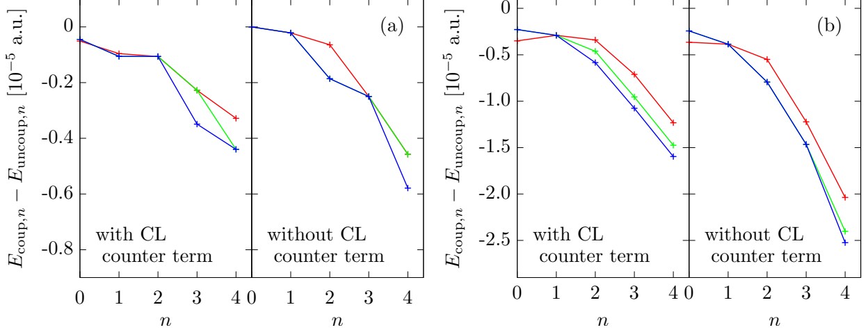
FIG. 5. Shift of the eigenenergies (Eq. (33)) of a Morse oscillator coupled to an off-resonant CL bath with parameters \omega_{\max} = 0.5 \omega_s , \omega_c = 0.1 \omega_s . The coupling strength is \eta_{\text{eff}} = 0.5 in panel (a) and \eta_{\text{eff}} = 2.0 in panel (b). The bath comprises either 10 (red crosses), 20 (green), or 40 (blue) HOs, and the solid lines are just a guide to the eye. The CL counter term is included in the calculations on the left side of each panel, and not included on the right side (Eq. (31)).
