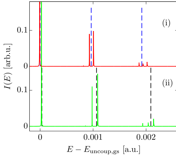
FIG. 4. Spectra for a Morse oscillator in a resonant CL bath with 20 HOs. Bath parameters are \omega_c = 0.5 \omega_s , \omega_{\max} = \omega_s , and \eta_{\text{eff}} = 0.5 . All remaining plot specifications as in Fig. 3.
