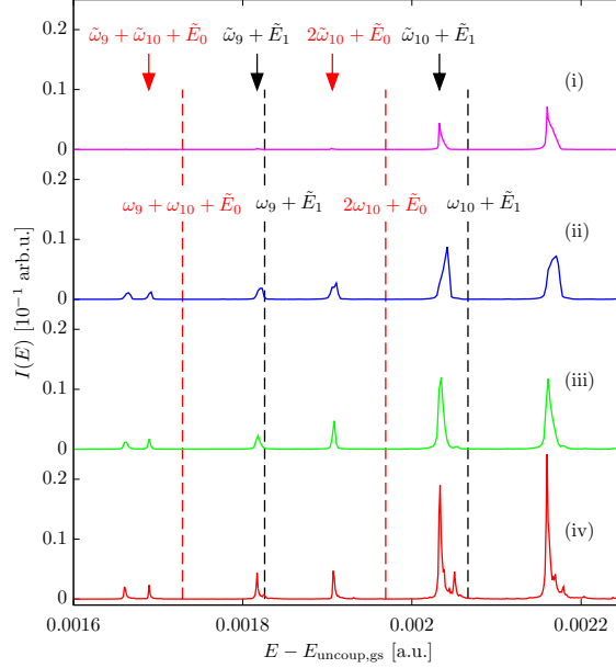
FIG. 2. Bath excitations in the spectrum of a Morse oscillator coupled to a CL bath. The rightmost peak is the second excitation of the system, the remaining peaks originate from bath modes. All bath parameters and plot specifications are identical to Fig. 1. The arrows highlight bath peaks of first order (fundamental) in black color and higher order (overtones) in red color, dashed vertical lines show the respective uncoupled counterpart.
