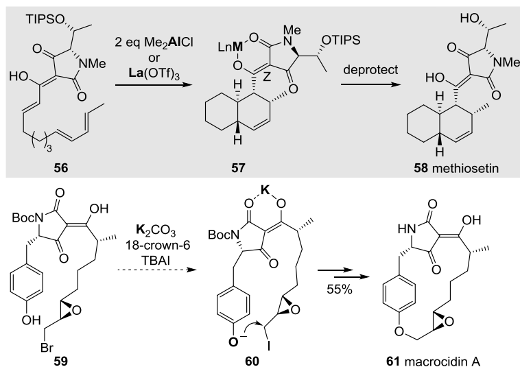
Figure 17. Metal chelate assisted syntheses of methiosetin 58 and macrocidin A 61 . TIPS = tris(isopropyl)silyl; OTf = \text{CF}_3\text{SO}_3 ; TBAI = tetrabutylammonium iodide; M = Al or La; L_n = number of auxiliary ligands.
