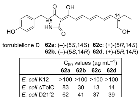
Figure 18. Antibacterial activity of stereoisomers of torribiellone D 62 against E. coli strains. E. coli K12: wildtype; E. coli \Delta\text{TolC} : mutant lacking the ArcAB–TolC efflux system; E. coli D21f2: supersusceptible mutant with truncated lipopolysaccharide core.
