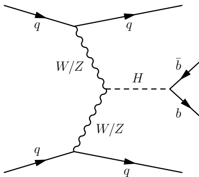
Figure 1: An example Feynman diagram illustrating vector-boson-fusion production of the Higgs boson and its decay to a b\bar{b} pair.
