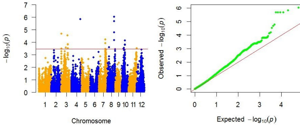
Figure 4. Manhattan (a) and Q-Q (b) plots of GWAS results for the SSI related to flowering delay.
