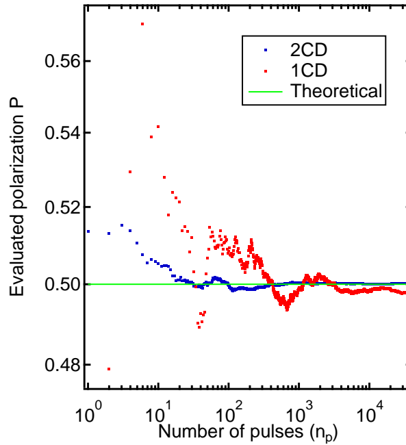
Fig. 3. The result of measurement of a 50% polarization ( P^{true} = 0.5 ) with a 1CD (red) and 2CD (blue) as a function of the number of averaged pulses.
