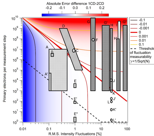
Fig. 2. Expected range of application with different sources. The dotted mesh (A,A',C,E,E',E'') defines quasi-continuous sources, the continuous line mesh defines continuous sources (B,D), light gray mesh defines pulsed solid state lasers (F,J,J',K,K',L,L'), the rombohedral mesh “hot” FELs (G,G',G''),H,H') and the white fill indicates superconducting FELs (I). A,A' - Synchrotron Beamline. B - Helium Lamp . C - quasi-CW VUV Laser. D - Electron gun. E',E'' - Femtoslicing synchrotron beamline. F - Table-top laser 4HG. G - LCLS Hard-X FEL. G' - Sacla Hard-X FEL. G'' - LCLS Self-seeding. H - Fermi FEL-1 (Seeded). H' - Fermi FEL-2 (Seeded,cascaded). I - FLASH FEL (SASE). J,K,J',K' - High power HHG Laser (Fluct. inferred from L). L,L' - Mid-power HHG Laser (for which shot-to-shot fluctuations were accurately measured).
