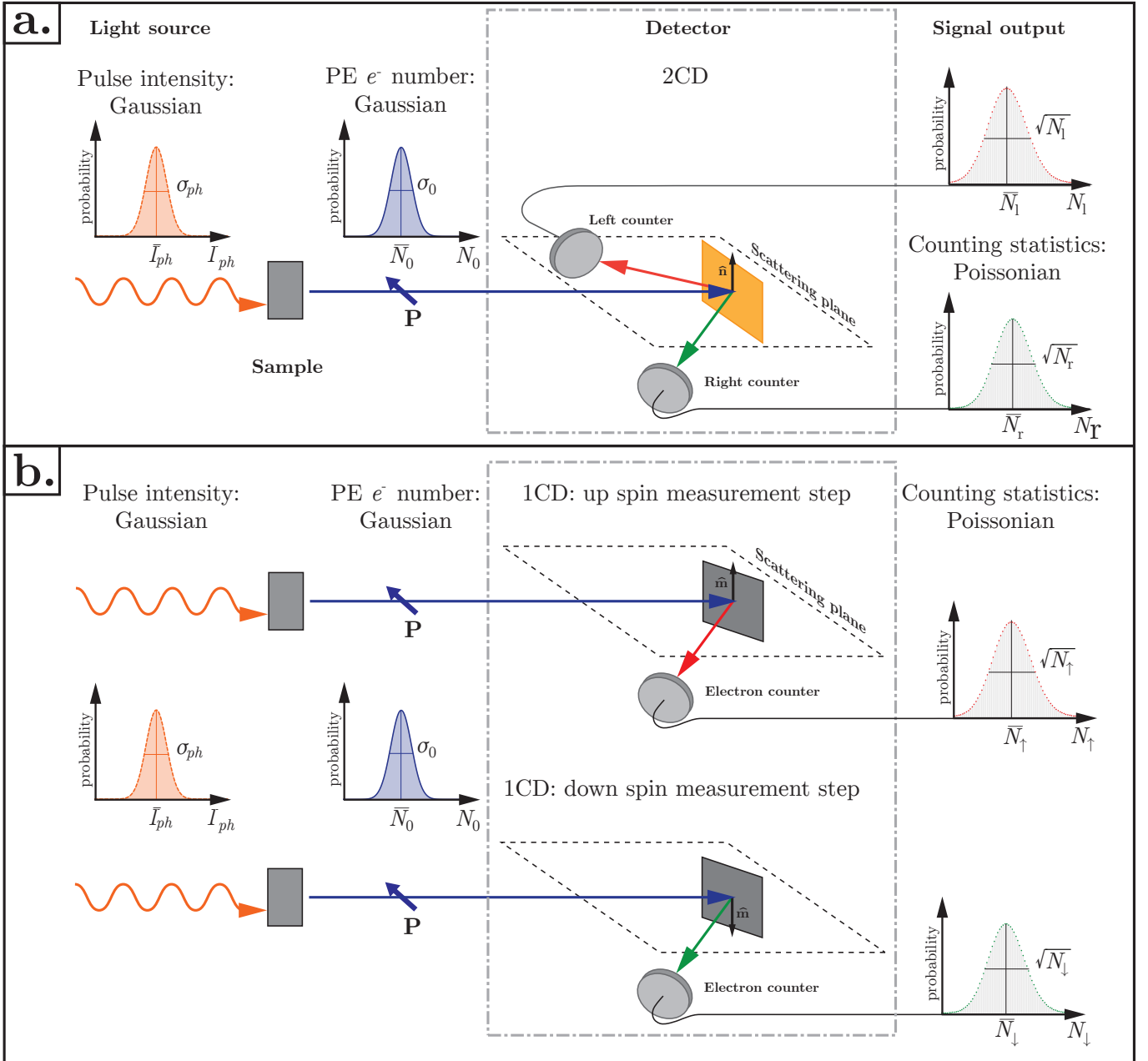
Fig. 1. a. Simplified scheme of the operation and of the accounted probability distributions in a 2CD detector. b. Simplified scheme of the operation and of the accounted probability distributions in a 1CD detector. It is divided in two subfigures in which the two successive steps needed for a single polarization measurement are shown.
