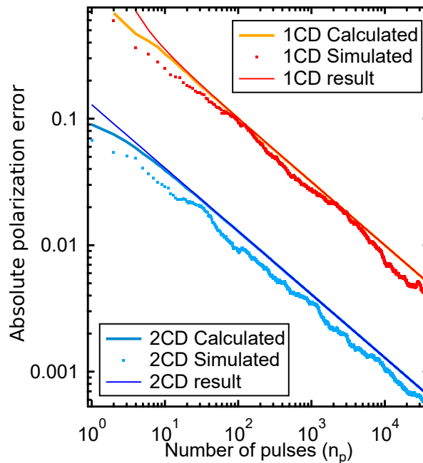
Fig. 4. The results of a simulated run on 1CD and 2CD detector. In this case, we used n_p = 36000 , corresponding to 1h acquisition at 10Hz, \bar{N}_0 = 100000 , \sigma_0 = 0.1 , S_{\text{eff}} = 0.36 for 1CD, \varepsilon_M = 6 \times 10^{-4} , \varepsilon_V = 1 \times 10^{-2} , N_{\text{sim}} = 100 . The solid red and dark blue line show the direct calculation from Eq. 19, 31, the light blue and orange the results of our approximation for large n_p , and the dots the simulated measurements.
