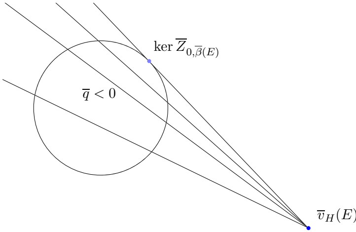
Fig. 1 A section of the negative cone \bar{q} \leq 0 and the tangent plane passing through \bar{v}_H(E) and \ker \bar{Z}_{0, \bar{\beta}(E)} . The other planes through \bar{v}_H(E) intersecting \bar{q} < 0 correspond to walls of stability for \bar{v}_H(E)
