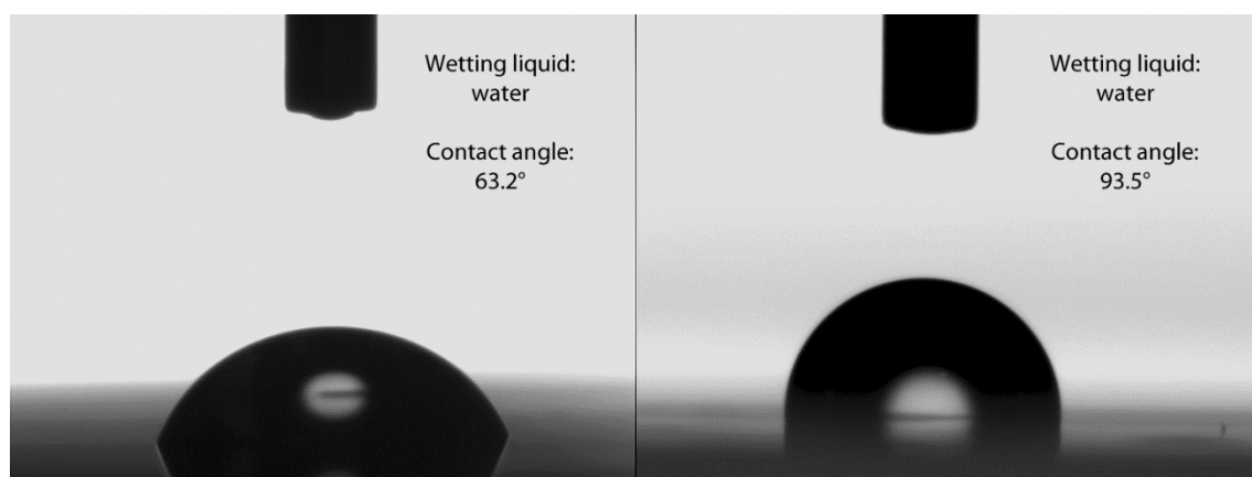
Figure S3. Sessile drop of water on (left) bare PET and (right) PET with H-coating.
