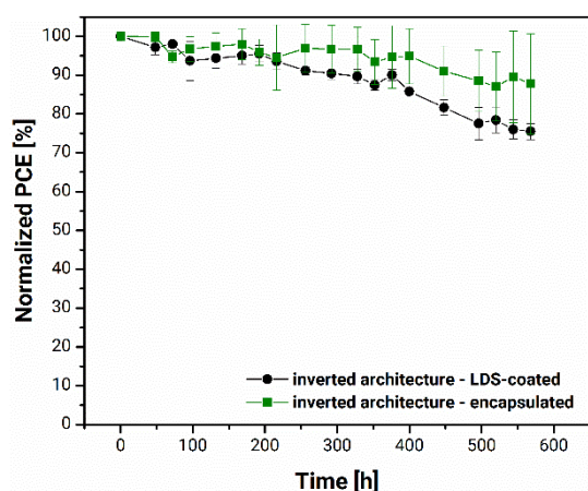
Figure S5. Normalized power conversion efficiency plot over light exposure time for LDS-coated devices and encapsulated devices in inverted configuration.
