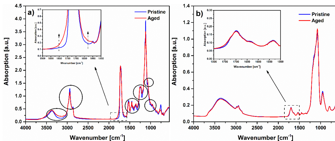
Figure S7. FTIR spectra prior to and after weathering of (a) the fully polymeric coating proposed in a previous work on dye-sensitized solar cells [S1] and (b) the organic/inorganic sol-gel hybrid material presented in this work. Insets show a zoomed image of the carbonyl stretching region, where signals associated to photo-oxidized species (arrows) are found to appear over weathering time in the fully polymeric coating. Conversely, the hybrid organic/inorganic sol-gel coating presented in this work shows remarkable stability.
