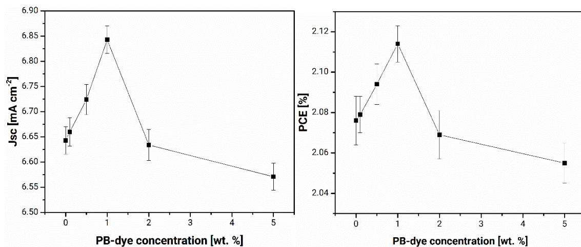
Figure S4. J_{sc} variation (left) and PCE variation (right) as a function of the PB-dye concentration for LDS-coated flexible OPV devices.
