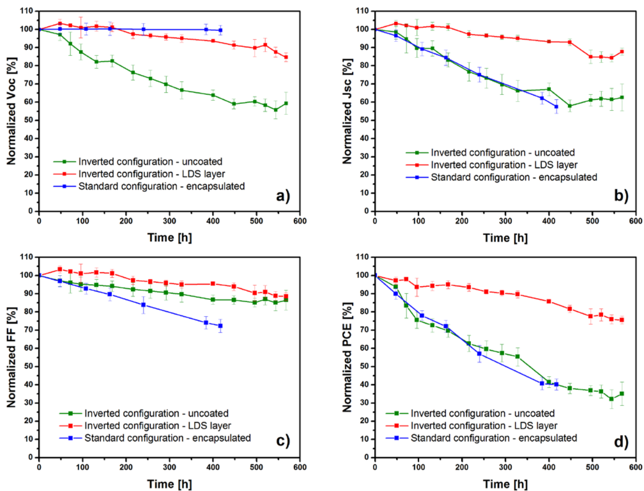
Figure S6. Normalized (a) Voc, (b) Jsc, (c) FF and (d) power conversion efficiency plots over light exposure time for uncoated reference devices, LDS-coated devices, and encapsulated devices in standard configuration.
