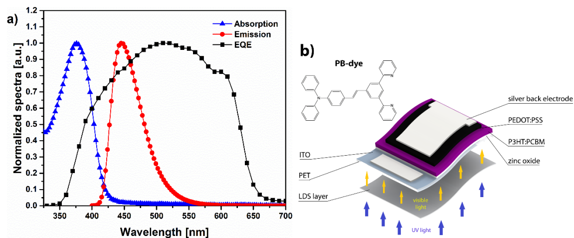
Figure 2. (a) Absorption and emission spectra of the organic dye, superimposed to the IPCE curve of the OPV device. (b) schematic illustration of the LDS process and the molecular structure of the PB-dye incorporated in the LDS layer.
