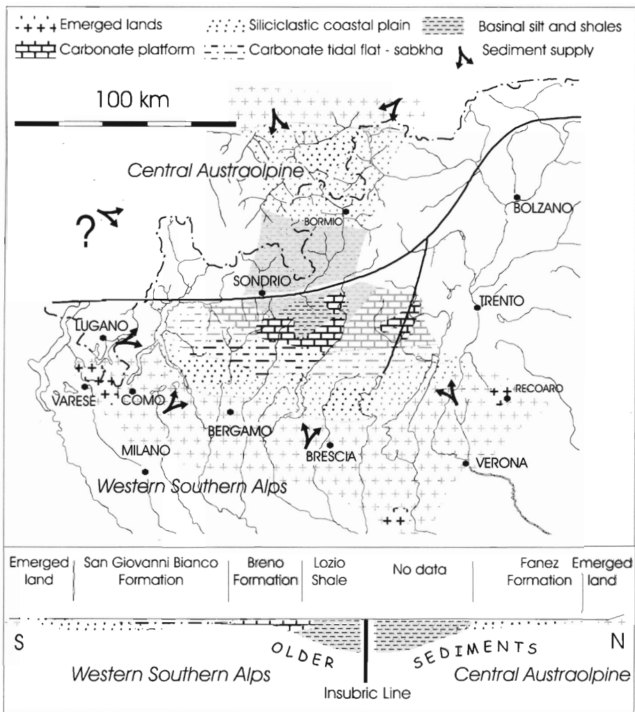
Fig. 8 - Schematic paleogeographic reconstruction (map and section) at the beginning of the deposition of "Black Pelites" in the western Southern Alps and in the Central Austroalpine (Cluozza Sandstone). The black hatches correspond to outcropping areas, the grey-ones to interpretation. Subsurface data in the Po Plain are placed according to Brusca et al. 1982.
