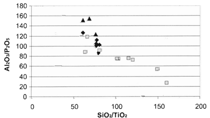
Fig. 4 - a) Microfacies (normal and polarized light) of a fine-grained sandstone of the Lozio Shale: note the presence of garnets (arrows) denoting the erosion of a metamorphic basement. Sample J207, X10. b) Diagrams of different ratios from chemical analysis of fine-grained siliciclastics from the Lozio Shale, Gorno and San Giovanni Bianco Fms. Note the similar distribution of the Gorno and San Giovanni Bianco samples and the different pattern of the Lozio Shale
