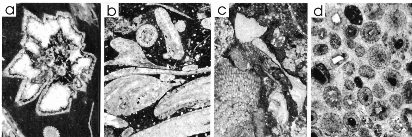
Fig. 6 - Microfacies of the "Bioclastic Horizon" in the Ave Section. a) Calcified star-shaped secondary anhydrite in a bioclastic wackestone. Sample AF13, X 10; b) Bioclastic packstone with coated and rounded grains (brachiopods, pelecypods) and superficial ooids, sample AE26, X10; c) Bioclastic packstone with red algae, crinoids, brachiopods, sample AE27, X20; d) oolitic grainstone with quartz grains at the nucleus of ooids, sample AE28, X 10.
