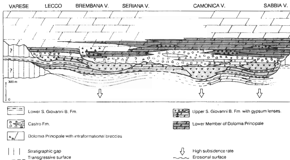
Fig. 2 - Stratigraphic scheme of the Late Carnian succession of Lombardy.
