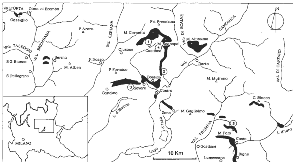
Fig. 1 - Map showing the location of the studied area and of the most important outcrops of the Castro Fm. as well as of Upper Carnian dolomitic breccias. Location of stratigraphic sections is labelled with numbers.
