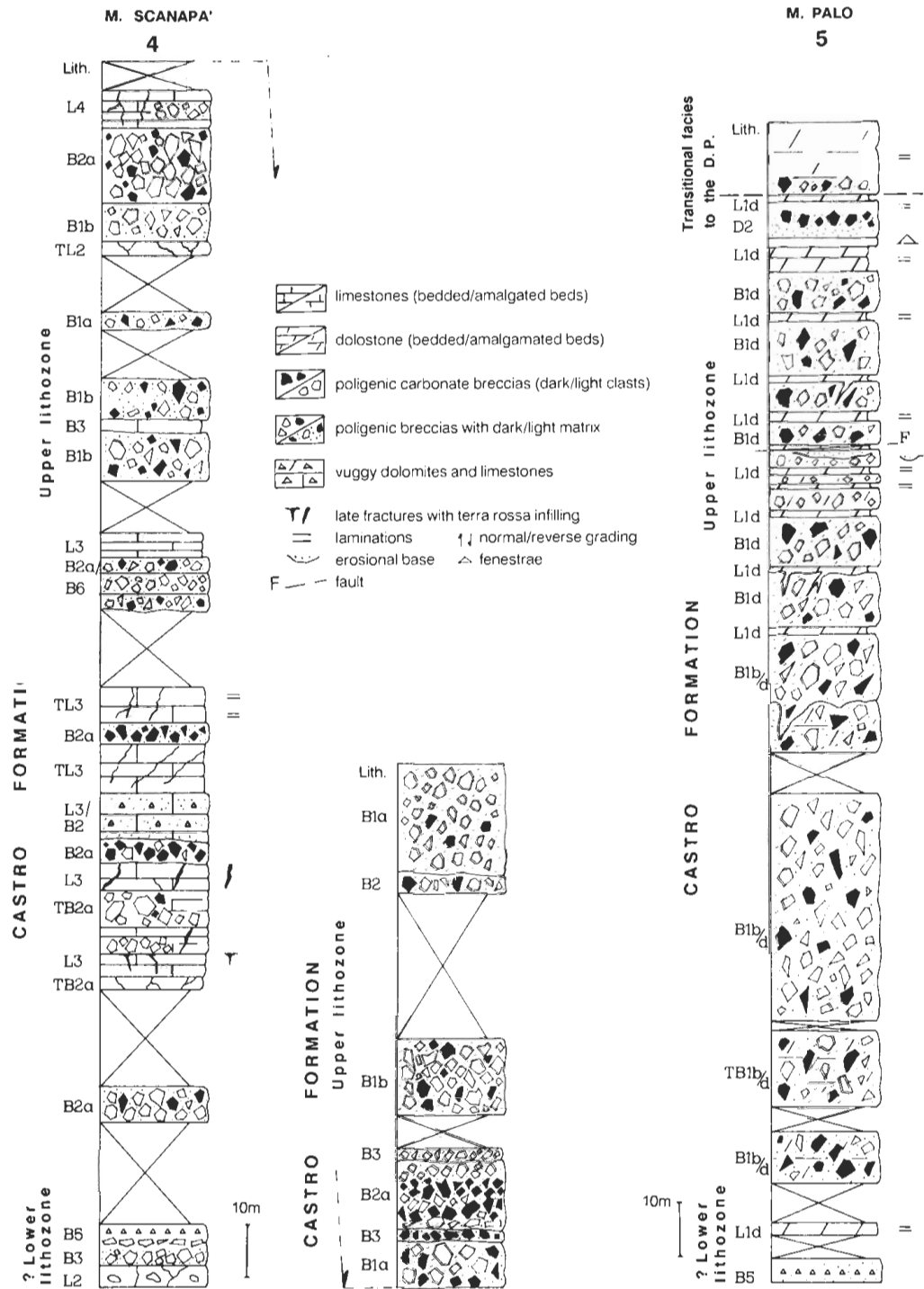
Fig. 5 - Stratigraphic sections of Castro Fm. at Monte Scanapà and Monte Palo.
