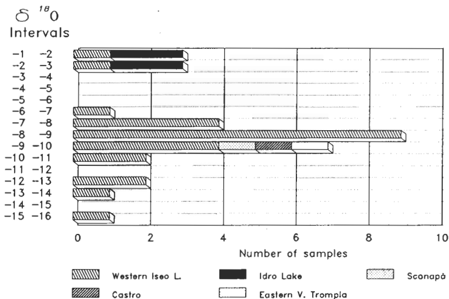
Fig. 11b - Geographical distribution of \delta^{18}\text{O} in the Castro Formation lithofacies.
