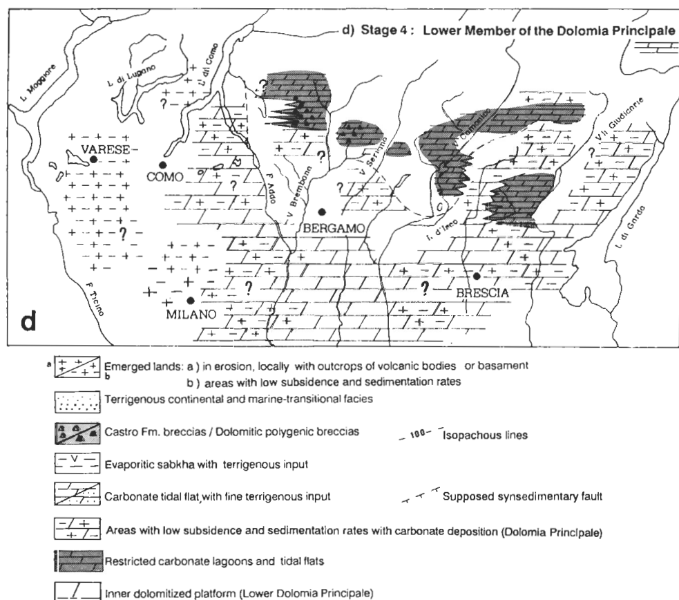
Fig. 9 - Late Carnian paleogeographic interpretative schemes (a,b,c,d), not palinspastic, from the deposition of the S. Giovanni Bianco Fm. to the sedimentation of the Lower Member of the Dolomia Principale. Palaeogeographic evolution of the southern areas (Po plain) is an extrapolation of our data of the Prealps outcrops and Agip data (Errico et al., 1979; Bongiorno, 1987).
