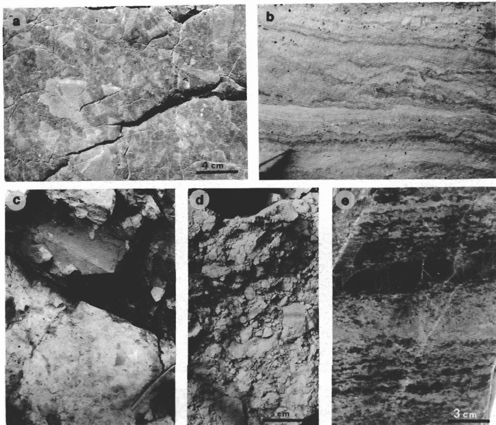
Fig. 6 - Castro Formation breccias and limestones lithofacies. a) Intraformational calcareous monogenic breccia, note clasts showing tension fractures filled by sparry calcite (Castro, upper lithozone). b) Laminated dolomitic limestones showing the development of incipient brecciation (Val Piana, lower lithozone). c) At the bottom polygenic breccias and intercalated dark azoic marly limestones. At the top of the latter irregular pockets of polygenic breccia (Val Piana, lower lithozone). d) Poorly sorted calcareous breccia with good compaction and affected by tectonics (Castro, base of upper lithozone). e) Pseudolaminated dark micrite with alternating light pseudosparitic "layers" with small dark intraclasts probably due to recrystallization phenomena (Val Piana, upper lithozone).
