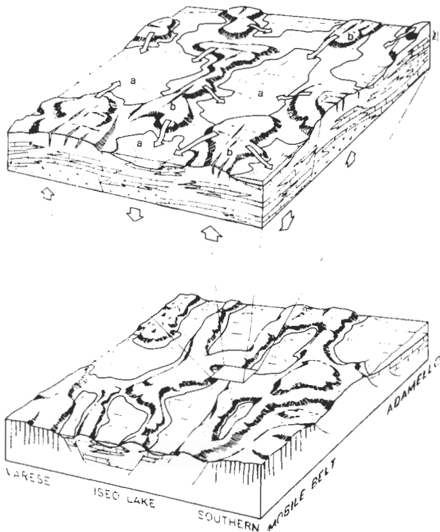
Fig. 12 - Depositional system proposed for the Castro Fm. a) Ephemeral, subsident lakes with fine limestones, intraformational breccias and dissolution-collapse breccias related to underlying evaporitic bodies. b) Mounds and ridges temporarily emerged related to dissolution-collapse and uplift-deformation phenomena into the underlying evaporites, desiccation of limestone muds. Tectonics may be an important element controlling subsidence in the central Lombardy depression and locally its paleogeographic setting.
