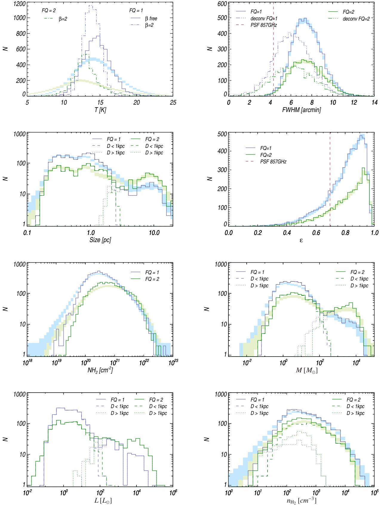
Fig. 12. Distribution of the physical properties of the PGCC objects with FQ=1 (blue) and FQ=2 (green). The coloured shaded regions provide an estimate of the impact of the individual uncertainties on the statistical distribution at a 1\sigma dispersion level around the mean value obtained from 10 000 MC realizations (see Sect. 6 for more details). The temperature distribution is shown for two temperature estimates, i.e., using a free emissivity spectral index \beta (solid line) or a fixed \beta=2 (dot-dashed line). The distribution of the intrinsic size, after deconvolution, is shown on the top right panel in dot-dot-dot-dashed line. The distributions of the physical size, mass, mean density and luminosity of the clumps are provided for sources with reliable distance estimates (DIST_QUALITY=1 or 2). These distributions are also shown separately for sources at solar distances smaller or larger than 1 kpc from the Sun, in dashed and dotted lines, respectively.
