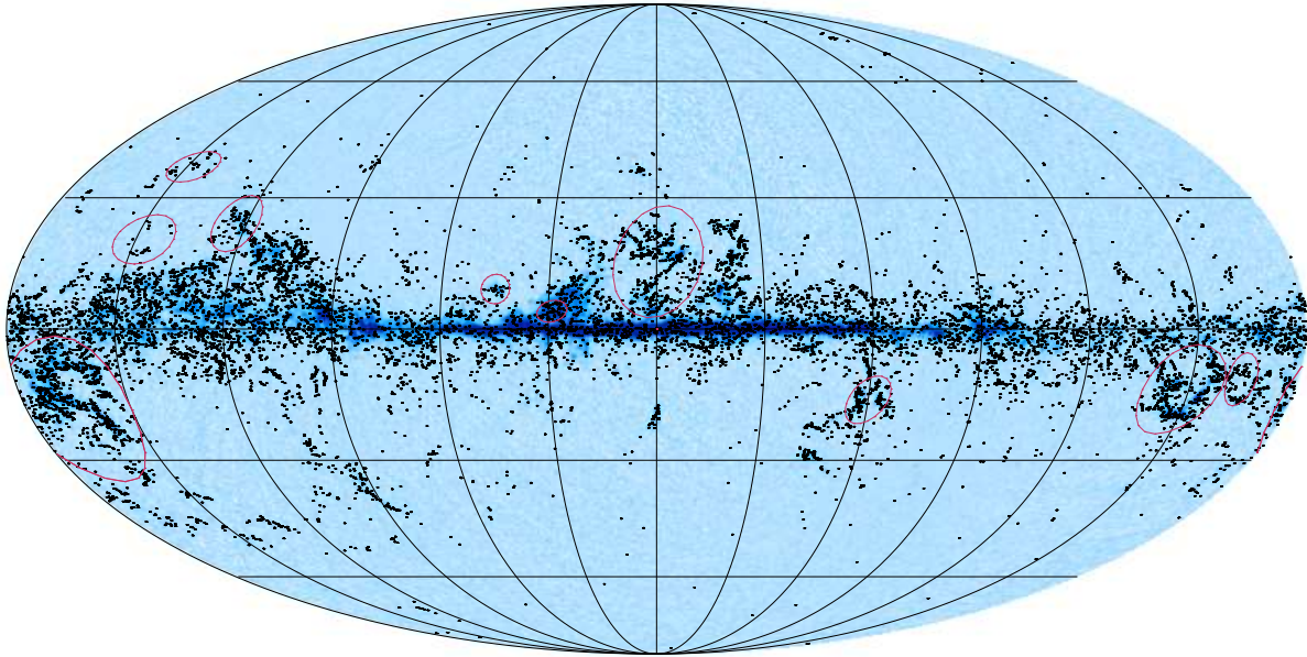
Fig. B.1. All-sky distribution of the PGCC sources with FQ=1 or 2, displayed over the Planck ^{12}\text{CO } J=1\rightarrow 0 map ranging from -5 to 30 \text{K.km.s}^{-1} . The locations of the molecular complexes used in the distance estimate procedure are shown as red circles.
