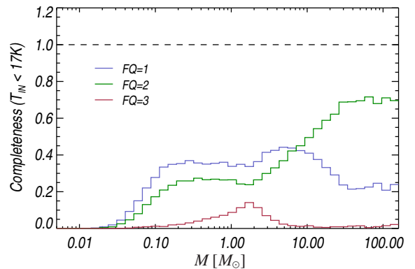
Fig. 4. Completeness as a function of the input temperature ( top panel ), latitude ( middle panel ), and mass ( bottom panel ) of the injected sources. For the latitude and mass cases, the input temperature was lower than 17 K. In addition, when considering the dependence of completeness on mass, all the sources are assumed to be at 100 pc from the Sun. Each panel shows the distributions obtained from selecting only the sources in a given FLUX_QUALITY category. In particular, FQ=1, 2 and 3 correspond to the blue, green and pink curves, respectively. Finally, the dotted line in each panel denotes the completeness for the sample of sources with input flux density S_{857}^{IN} > 15 Jy.
