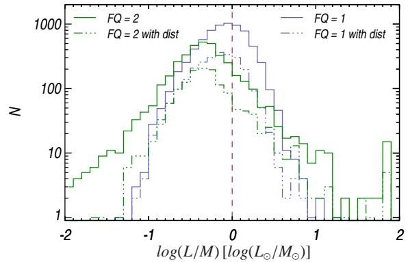
Fig. 13. Distribution of the luminosity to mass ratio of the PGCC clumps for sources with FQ=1 (blue line) and FQ=2 (green line). The dot-dot-dot-dashed line denotes the distribution for the subsample of sources with a reliable distance estimate.
