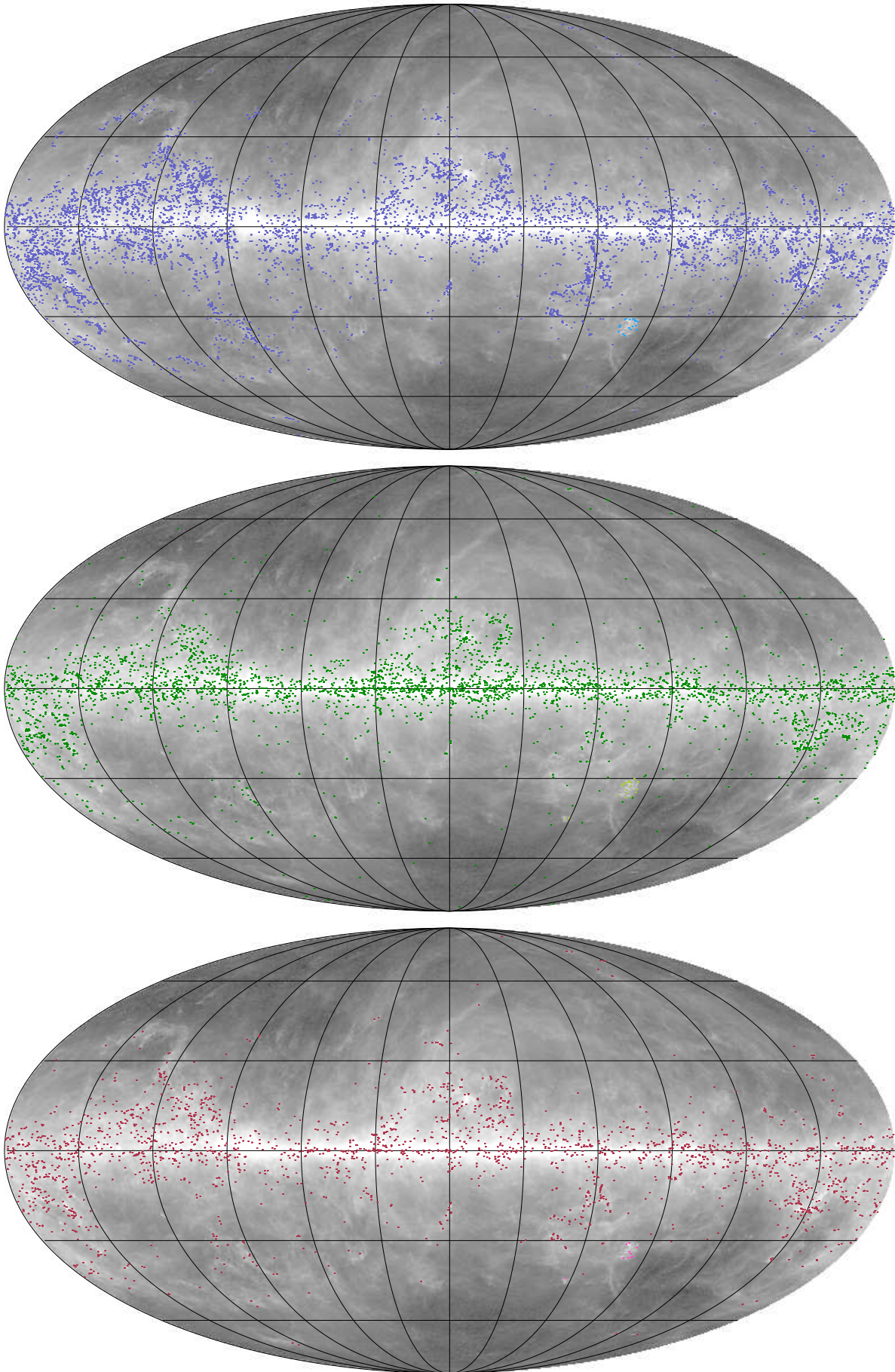
Fig. 2. All-sky distribution of the PGCC sources according to their FLUX_QUALITY category: "Reliable flux densities" (FQ=1, top panel), "Missing 3 THz flux density" (FQ=2, middle panel) and "Detection only" (FQ=3, bottom panel). Sources located in the LMC and SMC are also shown in light colours.
