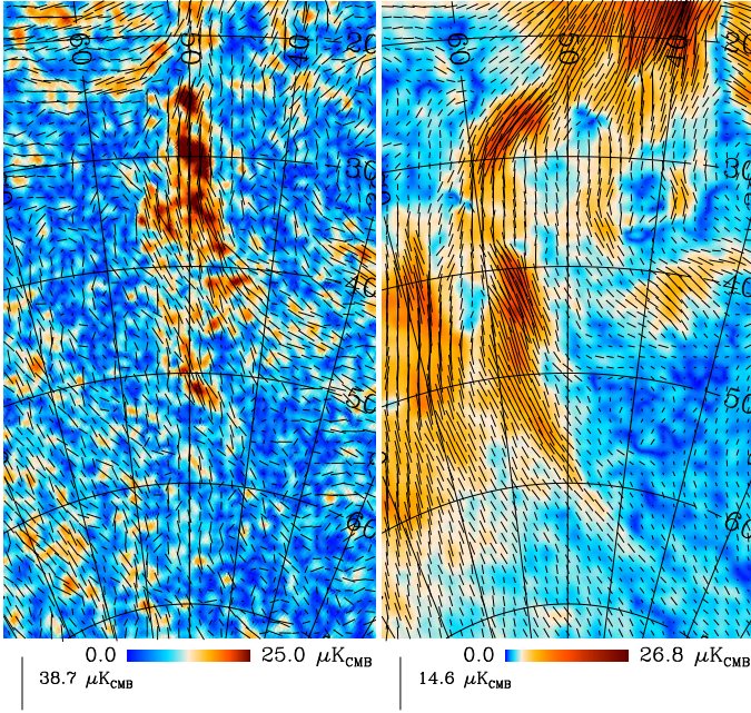
Fig. 28. The South Polar Spur. Left: Planck - WMAP polarization map; right: Planck 353-GHz dust polarization. The maps are centred at (l, b) = (50^\circ, -45^\circ) and the graticule has a 10^\circ spacing.
