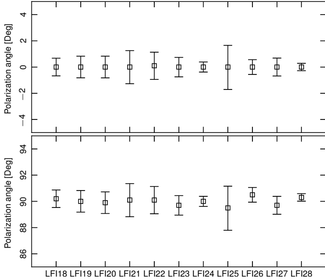
Fig. 4. Simulated polarization angles and error bars from the Crab measurements used in the analysis. Top: radiometer main arm. Bottom: radiometer side arm. The scatter of the plotted angles is much less than the error bars because the uncertainty in our simulations is much smaller than the error bars derived from Crab measurements.
