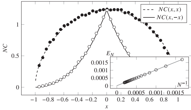
FIG. 1. sEBMP on the real line with points generated using a semicircle distribution, Eqs. (23). We plot the correlation functions C(x, x) and C(x, -x) for N = 3000 , obtained averaging over 5000 instances of the problem. We plot also the AOC E_N obtained averaging over 5000 instances. We compare with the theoretical predictions obtained from Eqs. (21).
