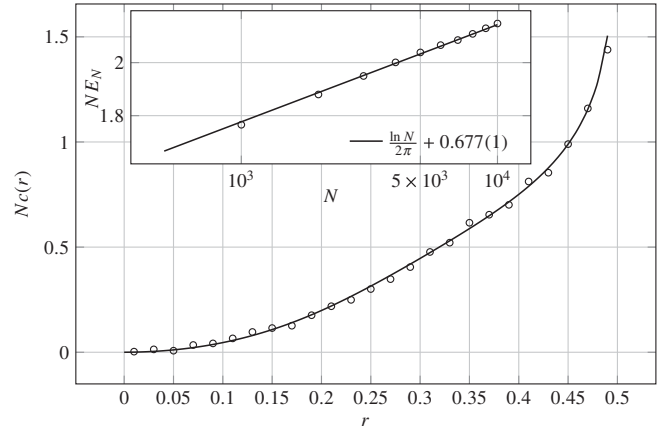
FIG. 2. Matching problem on the square. In the main plot, correlation function between points on the diagonals of the square, see Eq. (27), obtained for N = 3000 and averaging over 2 \times 10^4 instances. We compare with our analytical prediction. In the smaller plot, we compare our theoretical prediction for the AOC, Eq. (26) with numerical results obtained averaging over 2 \times 10^4 instances. In particular, the value of \gamma = 0.677(1) is obtained by a fit procedure.
