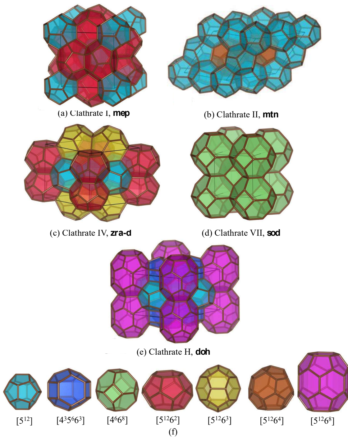
Figure 1. Structures of the five clathrates investigated in this work: (a)-(e). The building blocks of the structures are shown in (f).
