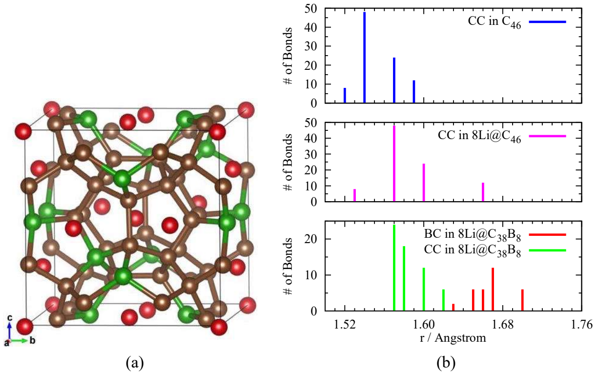
Figure 9. (a) The optimized R3c 8Li@C 38 B 8 unit cell with six 6 c and two 16 i carbon atoms substituted by B, and (b) histograms of B-C and C-C bond lengths in the unit cells of Clathrate I, 8Li@C 46 , and structure (a). Li, C, and B are represented by red, brown, and green spheres, respectively. The binning resolution in (b) is 0.01 Å.
