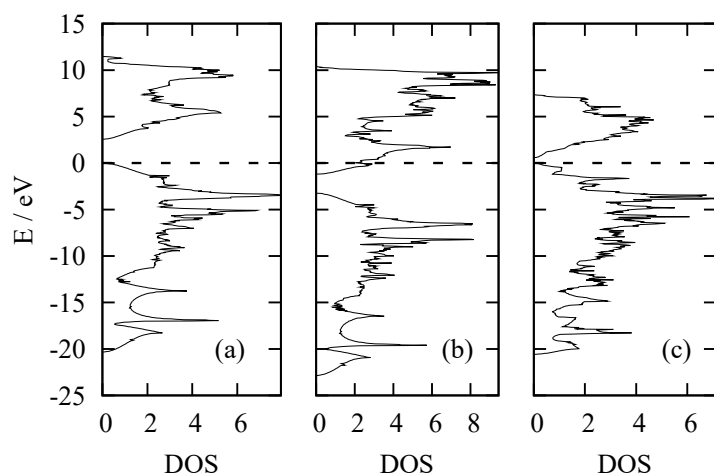
Figure 3. Densities of states of (a) Clathrate VII, (b) 2Li@C 12 , and (c) the representative P4 2 /mmc 2Li@C 10 B 2 . The DOS unit is states/eV/unit cell.
