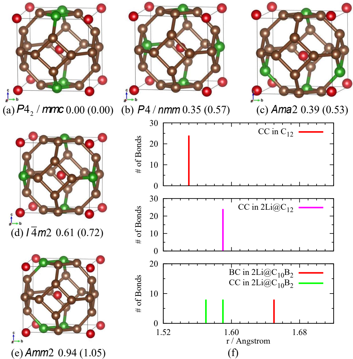
Figure 5. (a)-(e) The five 2\text{Li}@C_{10}B_2 unit cell structures with their relative enthalpies with respect to (a) (eV per unit cell, values in parentheses are under P = 40 GPa) and space group symbols. Li, C, and B are represented by red, brown, and green spheres, respectively. (f) Histograms of B-C and C-C bond lengths in the unit cells of Clathrate VII, 2\text{Li}@C_{12} , and structure (a).
