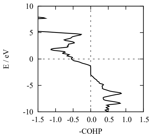
Figure 4. The Crystal Orbital Hamilton Population between two adjacent C atoms in 2\text{Li}@C_{12} around the Fermi level. The position of the highest occupied crystal level is indicated by the horizontal dashed line. Note that we plot the negative of COHP, following the convention of the chemical community.
