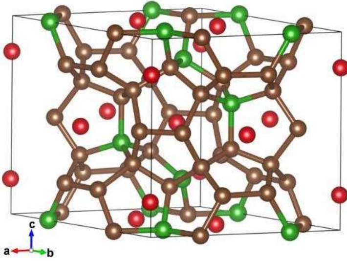
Figure 11. The optimized unit cell structure of the representative C2 7\text{Li}@C_{33}\text{B}_7 . Li, C, and B are represented by red, brown, and green spheres, respectively.
