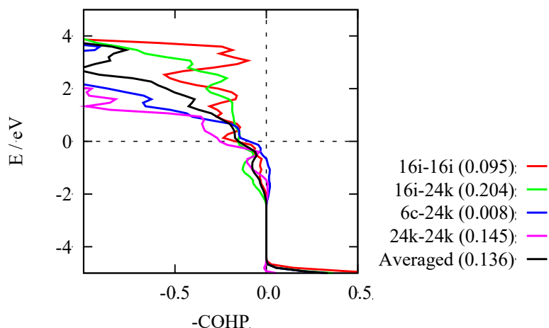
Figure 8. Crystal Orbital Hamilton Populations of the four types of C-C bonds and their weighted average in 8\text{Li}@C_{46} around the Fermi level. The position of the highest occupied crystal level is indicated by the horizontal dashed line. The numbers in parentheses are the integrated COHP (in eV) from E = -4 to 0 eV. Note that we plot the negative of COHP, following the convention of the chemical community.
