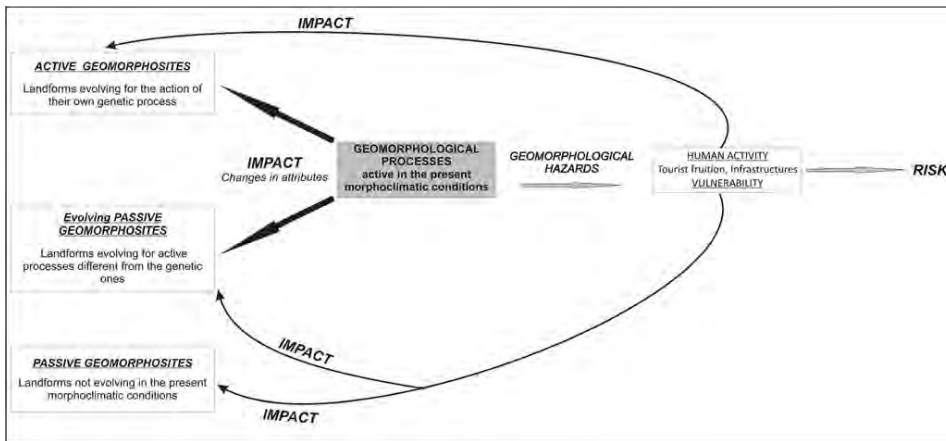
Fig. 1 Relationships between geomorphological processes, geomorphosites and human activity
