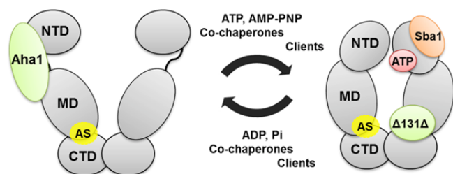
Figure 1. Schematic representation of Hsp90 structure and its conformational equilibrium. NTD, N-terminal Domain; MD, Middle Domain; CTD, C-terminal Domain; AS, predicted allosteric site; Aha1, Hsp90 co-chaperone; Sba1, yeast homologue of co-chaperone p23; \Delta 131\Delta , Hsp90 client protein model.
