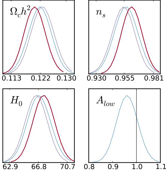
Figure 41. Comparison of the posterior distributions for \Omega_c h^2 , n_s , and H_0 for the default six-parameter \Lambda CDM model constrained by Planck (red); compared to the case when we allow a variable low- \ell power spectrum amplitude at \ell \leq 49 (blue); and when replacing the low- \ell temperature likelihood with a Gaussian prior on \tau , the optical depth of reionization (purple). The lower right panel shows the posterior distribution for the low- \ell amplitude, A_{low} .
