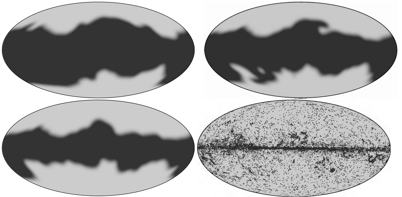
Figure B.2. Apodised Galactic and point source masks, which we derived (see text) from their non-apodised version shown in Fig. B.1. From left to right and top to bottom, the panels show the GA34, GA38, GA54 and PSA82 masks, which are the ones we combine to use in the likelihood analysis.
