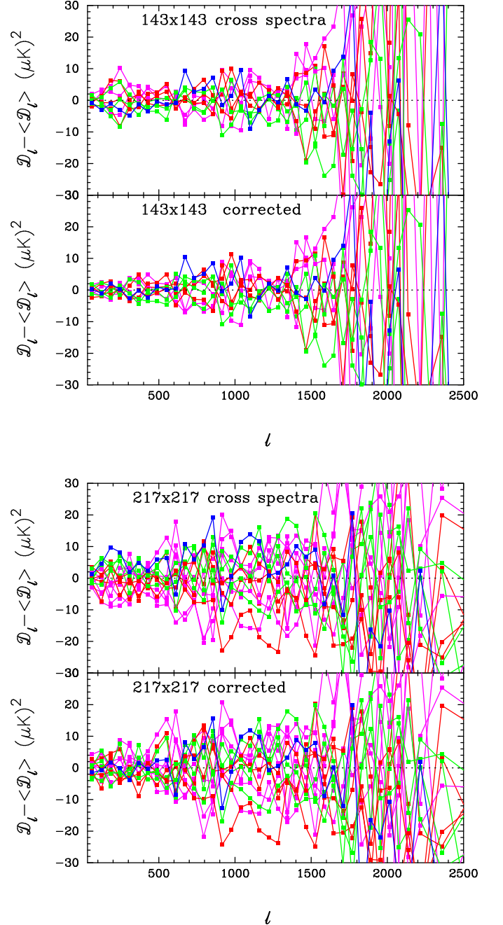
Figure 9. Cross spectra for the 143 GHz ( top ) and 217 GHz ( bottom ) channels, as in Fig. 8, before correction for multiplicative intra-frequency calibration coefficients (above), and after correction (below). The colour coding is the same as in Fig. 8.
