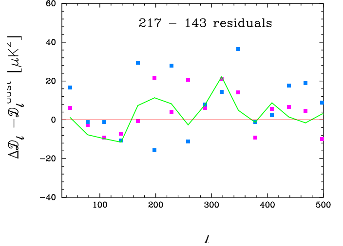
Figure C.2. Fake versus real data difference spectra. The magenta points show the double difference power spectrum of actual data (as in Figure 3). The green line shows the same double difference spectrum computed from the ILC + 857 dust template maps described in the text. This model provides a good match to the magenta points both in amplitude and phasing. The blue points show the difference of the 217 and 143 power spectra for mask1, which adds CMB cosmic variance, illustrating why we use double-differenced spectra for this comparison. In all cases, the smoothed dust power spectrum model of equation (9) (with slightly adjusted amplitude to bring the residuals at these low multipoles close to zero) has been subtracted.
