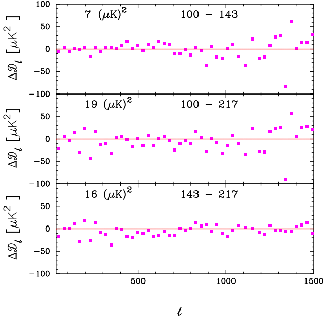
Figure C.3. Power spectrum residuals between the summed cross-spectra at three HFI frequencies. The top panel shows 100 \times 100 - 143 \times 143 , the middle panel shows 100 \times 100 - 217 \times 217 and the bottom panels shows 143 \times 143 - 217 \times 217 . A ‘best fit’ model for unresolved foregrounds has been subtracted from the power spectrum at each frequency. The scatter in the multipole range 50 \leq \ell \leq 500 is listed in each panel.
