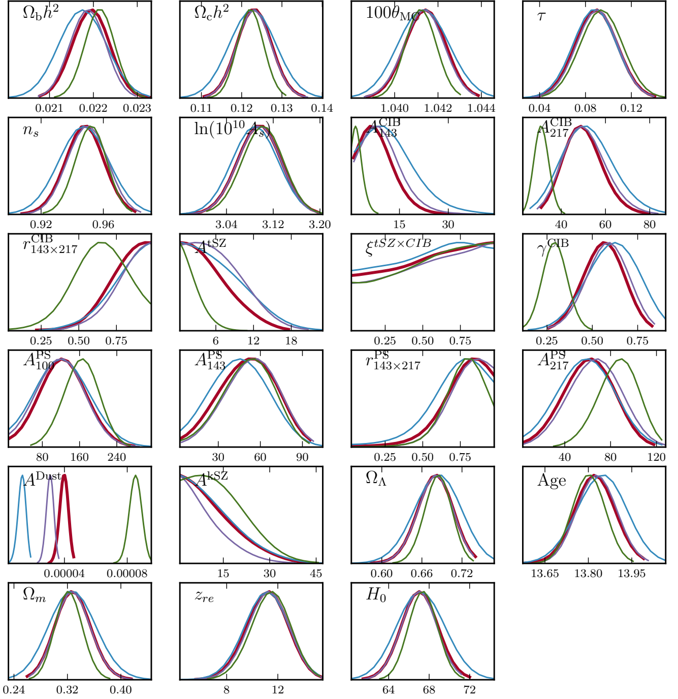
Figure D.5. Impact of changing the Plik Galactic mask, increasing the sky area used from GA21 (blue), GA34 (purple), GA38 (red, reference), to the least conservative GA54 (green). All results use the 100 \leq \ell \leq 2508 range. Note that the CamSpec likelihood uses the G35 mask for the 143 and 217 GHz channels, and G56 at 100 GHz, but with a restricted, composite multipole range.
