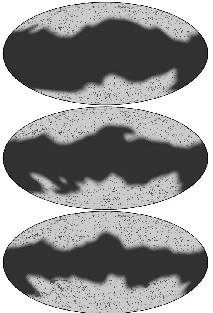
Figure 2. Set of masks (CL31, CL39, CL49) used for the likelihood analyses, in Mollweide projection.
