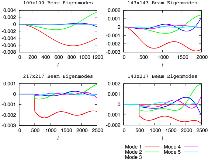
Figure A.2. Eigenmodes of the beam covariance matrix, shown for each cross-spectrum used in the analysis. The largest five modes are shown for each cross-spectrum.
