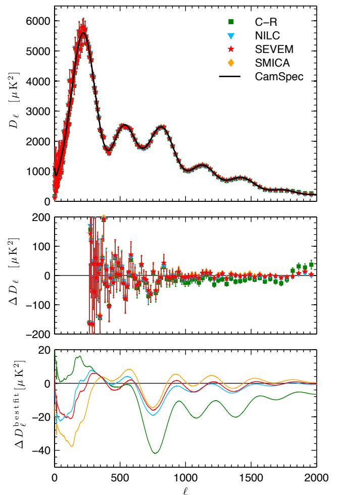
Figure 29. Top: CMB power spectrum, with best-fitting foreground model removed, compared to the CamSpec best fit model. Middle: the residuals with respect to this best-fit model. Bottom: residuals of the best-fit models from the map-based likelihoods, with respect to the CamSpec best fit model.
