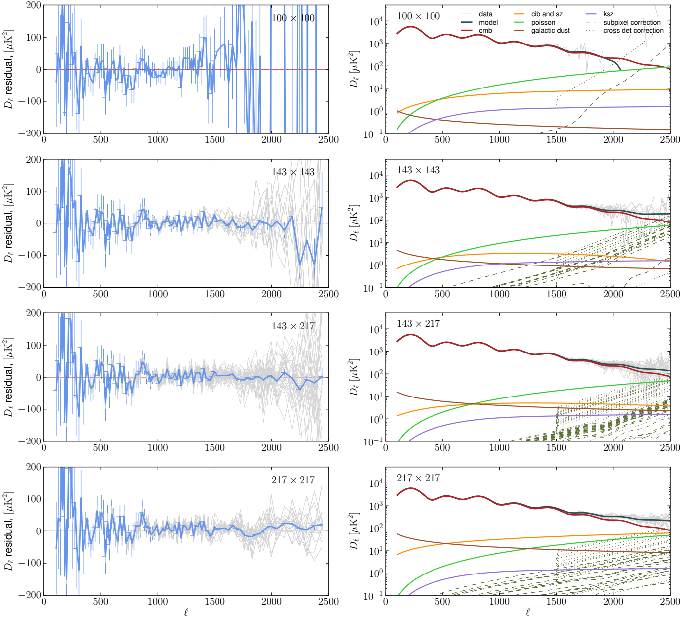
Figure 17. Left: Residuals between the Planck power spectrum derived with Plik using ‘validation’ settings (described in the text) and the Plik best-fit model. The light grey lines show residuals for individual detector pairs within each frequency combination. The blue lines show the inverse covariance weighted averages of the individual residuals, together with their errors computed from the covariance matrix. Right: Decomposition of the total best-fitting model power spectra into CMB, combined thermal SZ and CIB, unresolved point sources, kinetic SZ, and Galactic dust.
