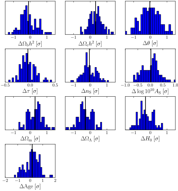
Figure 22. Distribution of the difference between cosmological parameter mean posterior values, as estimated by Plik (assuming foreground spectra are known) from the (CMB + fixed foregrounds + noise) FFP6 simulations, and the corresponding posterior parameter mean values from CMB only simulations (based on the same CMB realisations as in the FFP6 simulations), in units of the FFP6 posterior standard deviations. This demonstrates the absence of methodological bias at the level of the intrinsic dispersion between realisations, while removing from the distributions the dominating scatter coming from the purely CMB induced cosmic variance. In these figures, the dominant source of scatter comes from the CMB-foreground chance correlations in the signal dominated part of the spectrum, and from the noise scatter at large multipoles.
