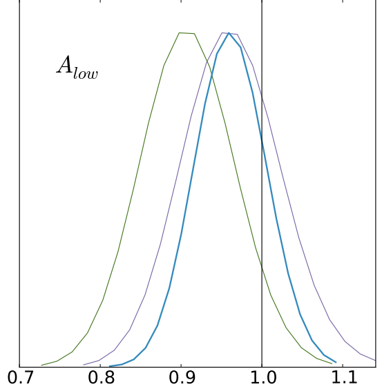
Figure 40. Posterior distributions for the low- \ell spectrum amplitude, A_{\text{low}} , estimated using the Planck likelihood, with \ell_{\text{low}} = 32 (green) and \ell_{\text{low}} = 49 (blue). The purple line shows the distribution derived using the WMAP temperature likelihood with \ell_{\text{low}} = 32 .
