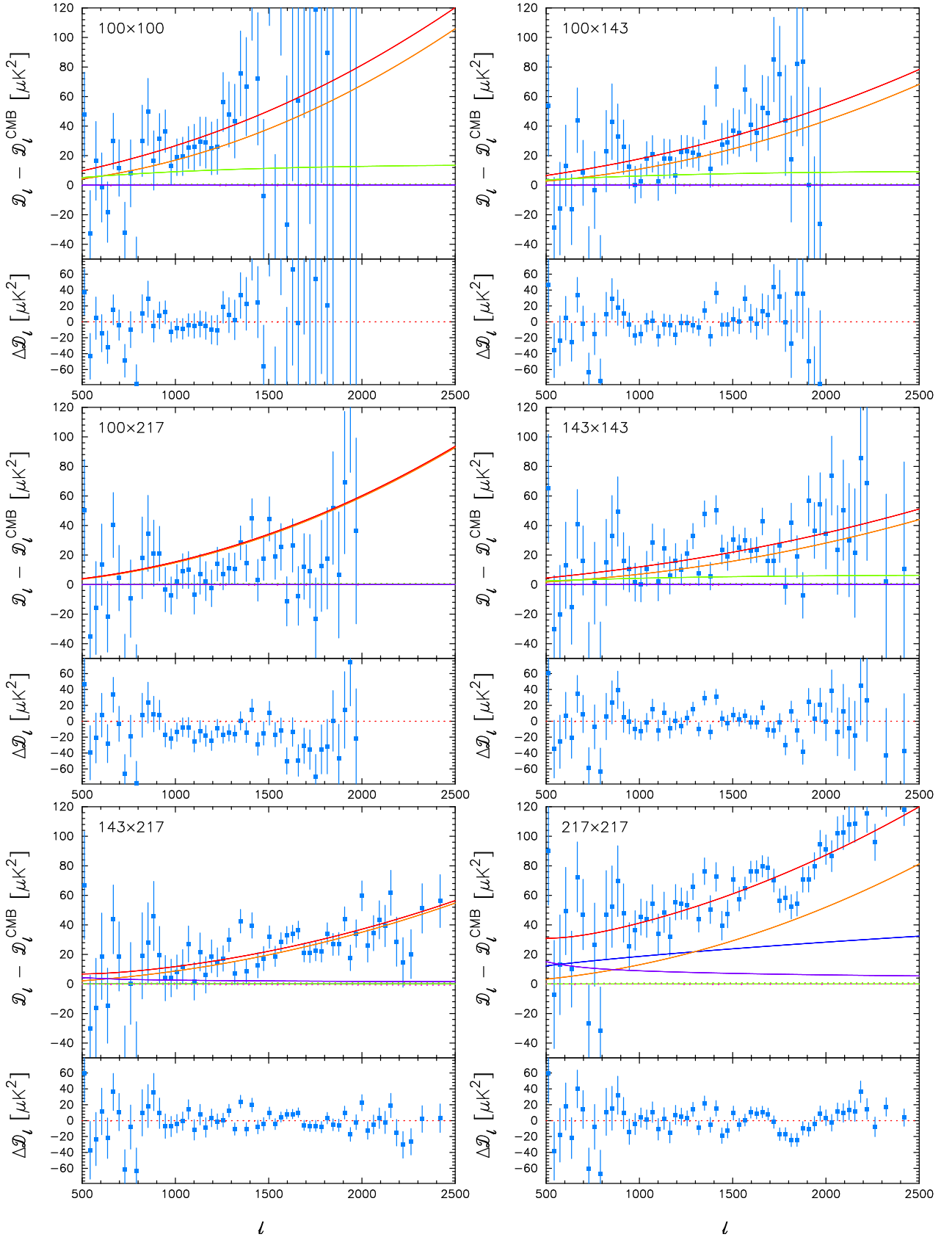
Figure 13. Foreground model over the full range of HFI cosmological frequency combinations. The upper panel in each plot shows the residual between the CamSpec measured power spectrum and the ‘best-fit’ primary CMB power spectrum, i.e., the unresolved foreground residual for each frequency combination. The lower panels show the residuals after removing the best-fit foreground model. The lines in the upper panels show the various foreground components. Major foreground components are shown by the solid lines, colour coded as follows: total foreground spectrum (red); Poisson point sources (orange); CIB (blue); thermal SZ (green), Galactic dust (purple). Minor foreground components are shown by the dotted lines: kinetic SZ (green); tSZ X CIB cross correlation (purple). The 100 \times 143 and 100 \times 217 GHz spectra are not used in the CamSpec likelihood. Here we have assumed r_{100 \times 143}^{PS} = 1 and r_{100 \times 217}^{PS} = 1 .
