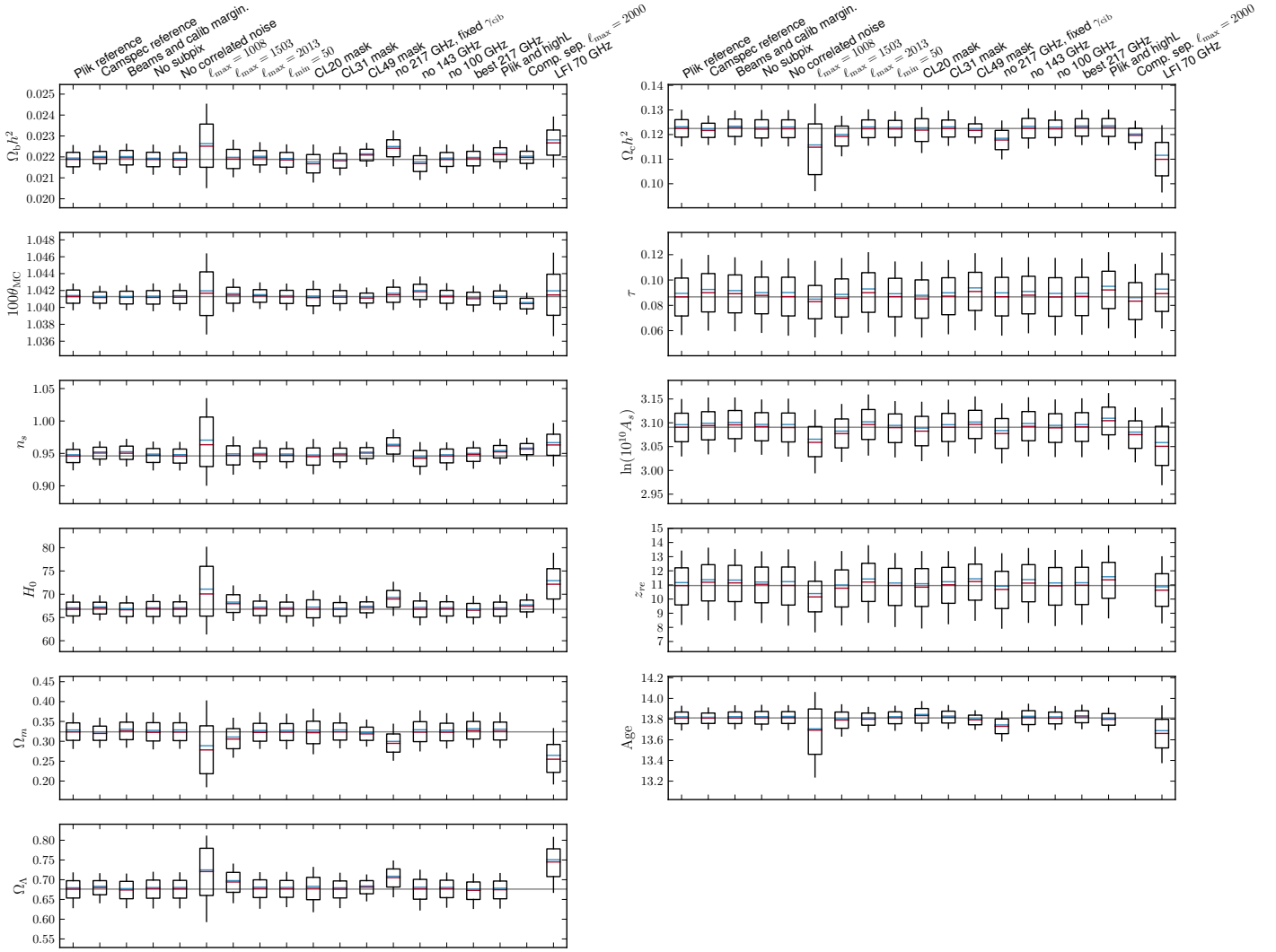
Figure 24. Comparison of the distributions of cosmological parameters obtained with Plik in the reference case (left) with a set of validation test cases. The red line indicates the median and blue the mean, computed from the posterior histograms. The box shows the 68% confidence interval; the outer line the 95% interval.
