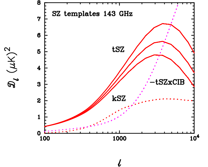
Figure 6. SZ templates at 143 GHz computed for a normalisation of \sigma_8 = 0.8 . The tSZ templates are from the model of Efstathiou & Migliaccio (2012) for three values of the evolution parameter \epsilon , \epsilon = 0 (top), \epsilon = 0.25 (middle) and \epsilon = 0.5 (lower). The kinetic SZ template is from Trac et al. (2011). The tSZ x CIB cross correlation (143 \times 143 GHz) is from the Addison et al. (2012b) template with parameters described in the text, and is negative for 143 \times 143 GHz.
