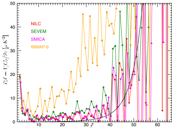
Figure D.12. Power spectrum of the residual CMB maps, relative to Commander, for the NILC, SEVEM, and SMICA methods. The 1\sigma expected noise level is shown in black.
