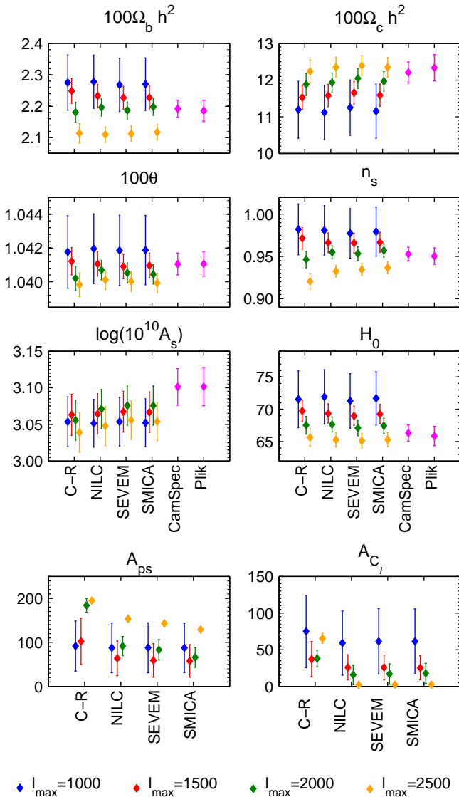
Figure 30. The variation of cosmological and foreground parameters estimated for the four CMB maps as function of \ell_{\max} = 1000, 1500, 2000, 2500 , with \ell_{\min} = 70 , compared to those obtained with the CamSpec and Plik likelihoods. Parameters are consistent to 1\sigma for \ell_{\max} \leq 2000
