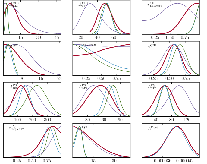
Figure 20. Comparison of foreground parameters estimated with the CamSpec and Plik likelihoods. The purple (red) lines show the CamSpec (Plik) distributions using only Planck data, and the green (blue) lines show the CamSpec (Plik) results when additionally including ACT and SPT.
