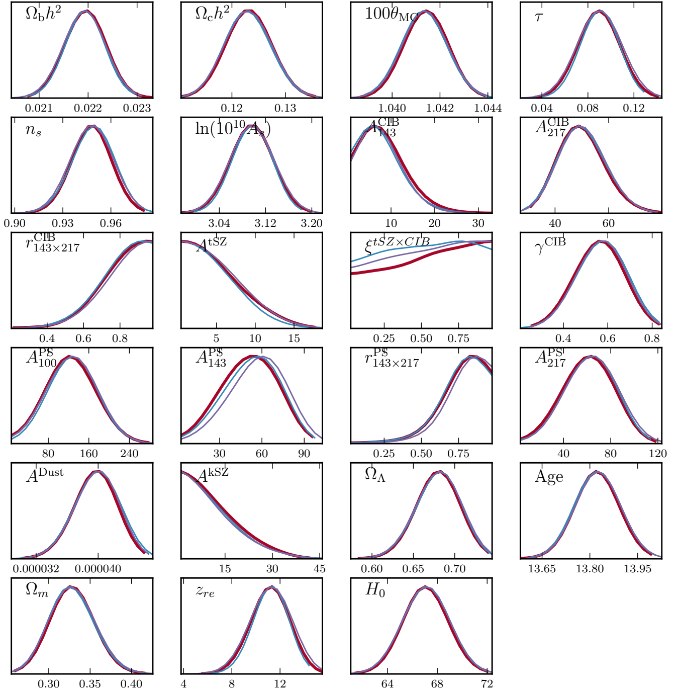
Figure D.2. Impact of removing the sub-pixel effect (blue) or the correlated noise between detector sets (purple), compared to the Plik reference case (red).
