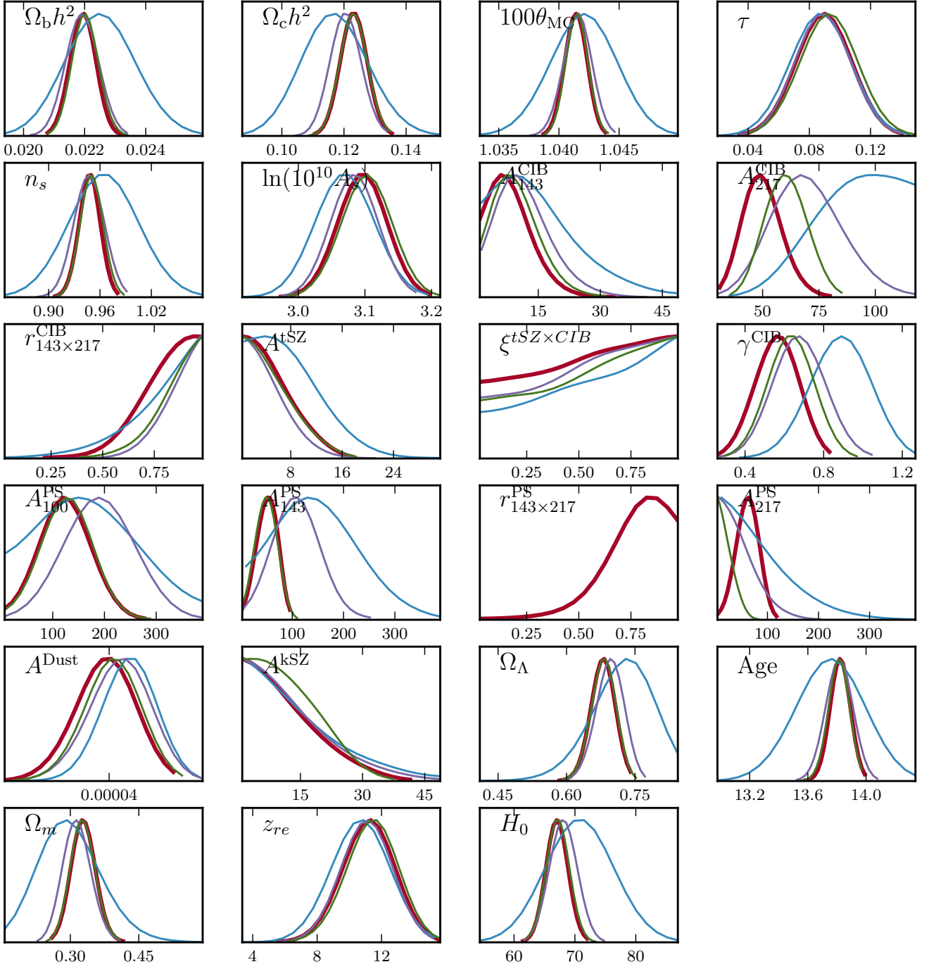
Figure D.3. Impact on the cosmological and foreground parameters of varying the maximum multipole, \ell_{\max} , retained in the Plik likelihood. We consider \ell_{\max} = 1008 (blue), 1503 (purple), and 2013 (green) in addition to the reference \ell_{\max} = 2508 (red).
