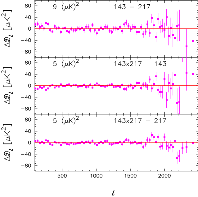
Figure 10. Differences between the 143 \times 143 , 143 \times 217 , and 217 \times 217 cross spectra (plotted in bins of width \delta\ell \approx 31 ). The best-fit model for unresolved foregrounds has been subtracted from each spectrum. The numbers list the dispersions over the multipole range 800 \leq \ell \leq 1500 .
