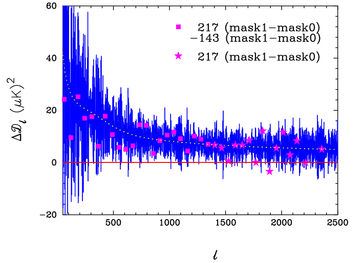
Figure 3. Differences between power spectra evaluated from the union masks \text{G22} \cup \text{PSA82} and \text{G35} \cup \text{PSA82} ( \equiv \text{mask0} and \text{mask1} respectively in the legend), showing the presence of Galactic dust. For \ell \leq 1400 the spectra show the 217–143 “double-differenced” power spectrum, rescaled to correct for dust emission at 143 GHz. For \ell > 1400 the 217 mask differenced power spectrum is plotted. The blue line shows the 857 GHz mask-differenced power spectrum scaled to 217 GHz as described in the text. The green dotted line shows the best-fit of Eq. 9 scaled to 217 GHz. This is the model that we use to subtract dust emission at high multipoles from the 143 \times 143 , 143 \times 217 and 217 \times 217 spectra with suitably adjusted scaling factors.
