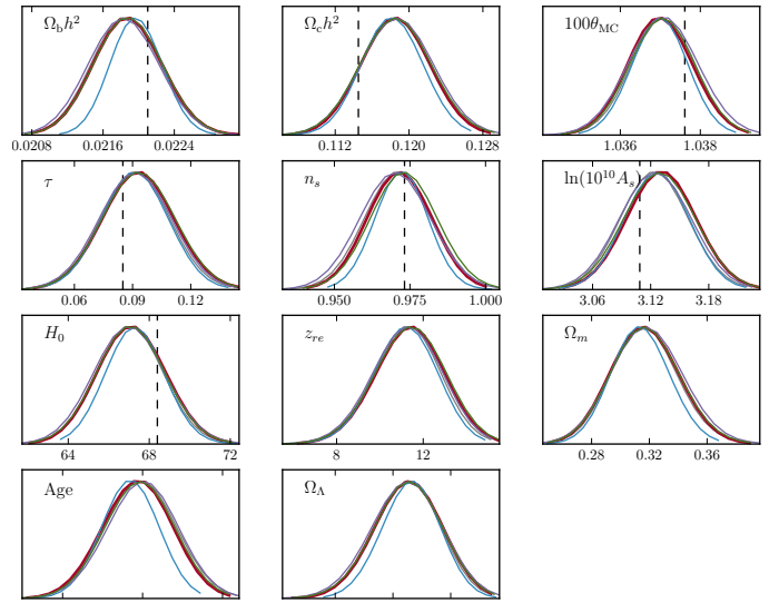
Figure 23. Posterior marginal distributions of cosmological parameters obtained by Plik on a single FFP6 realisation, under different assumptions on the foreground model. Red thick lines correspond to the foreground model parametrisation described in Sect. 3 with fixed \gamma^{\text{CIB}} . Purple lines (resp. green, grey) show the effect of leaving \gamma^{\text{CIB}} free (resp. letting \gamma^{\text{Dust}} free, or fixing \gamma^{\text{CIB}} to 0.4, 2\sigma away from the peak posterior value). Finally, the blue lines correspond to the analysis made on CMB-only simulations. The input values of the parameters of the simulation are shown as dashed vertical lines.
