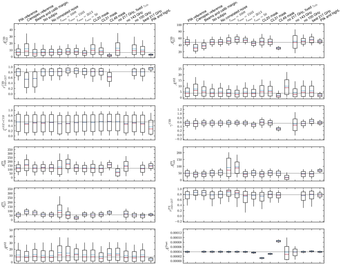
Figure 25. Comparison of the distributions of foreground model parameters obtained with Planck , as in Figure 24.
