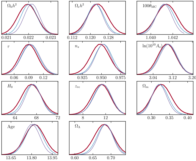
Figure 19. Comparison of cosmological parameters estimated from the CamSpec (blue) and Plik (red for mask CL39; purple for mask CL49) likelihoods. All parameters agree to better than 0.2\sigma when CL49 is used for Plik, matching the sky area used by CamSpec at 100 GHz.
