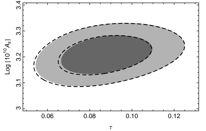
Figure 33. Comparison of constraints on \tau and A_s using the split temperature-polarization WMAP likelihood approach (dashed contours; Eqs. 24 and 25) with those obtained with the exact brute-force pixel likelihood (shaded contours; Eq. 21).
