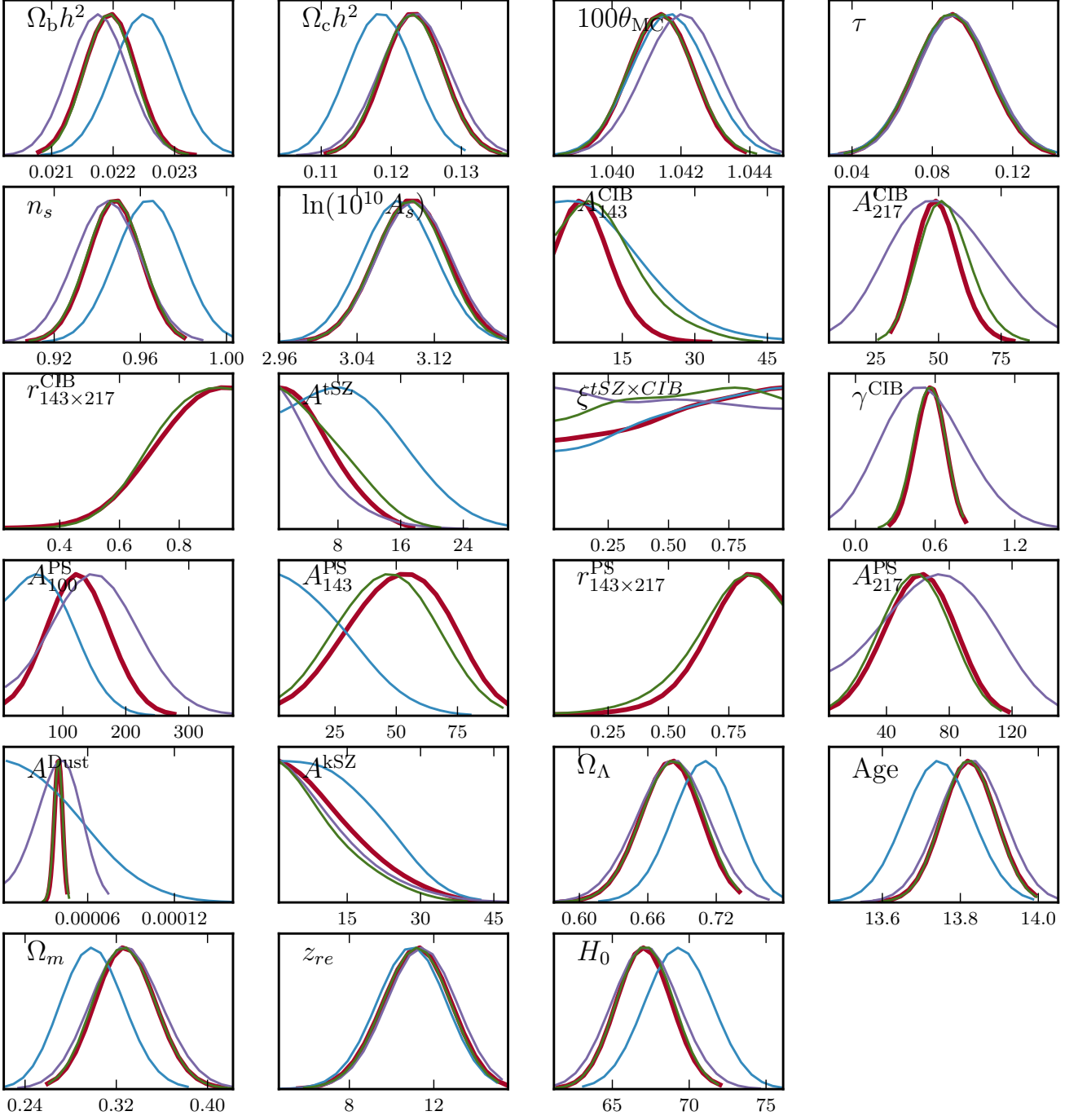
Figure D.6. Impact on parameters of removing one single frequency channel (i.e., all spectra with at least one frequency in the removed channel). Results are shown removing the 100 GHz (green), 143 GHz (purple), or 217 GHz (blue) channels, compared to the reference case (red). Where the 217 GHz channel is removed, the CIB spectral index is held fixed at \gamma^{CIB} = 0.6 .
