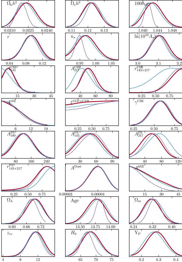
Figure 27. Posterior distributions for cosmological parameters obtained with Planck , varying the Helium abundance Y_P (red). We show the effect of marginalizing over calibration and beam errors (blue), and the results obtained using the reference settings (purple), where Y_P is constrained by BBN.
