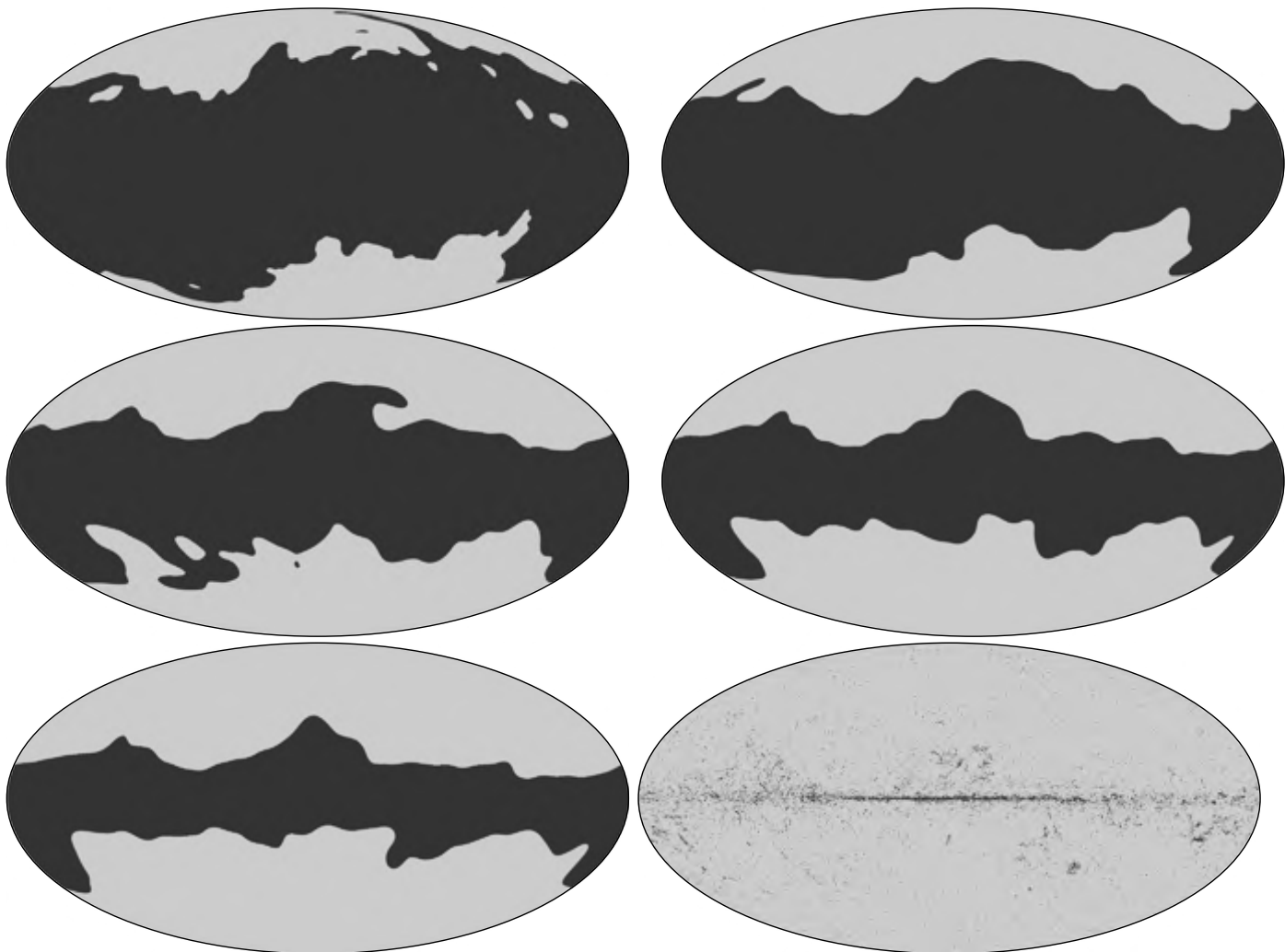
Figure B.1. Set of unapodised foreground masks, G22, G35, G45, G56, G65, PS96, which, once apodised, are used for the likelihood analyses. The Galactic (G22 to G65) masks are defined using a threshold of the 353 GHz Planck temperature map. The (lower-right) PS96 point source mask is based on the union of resolved sources in all channels from 100 GHz to 353 GHz.
