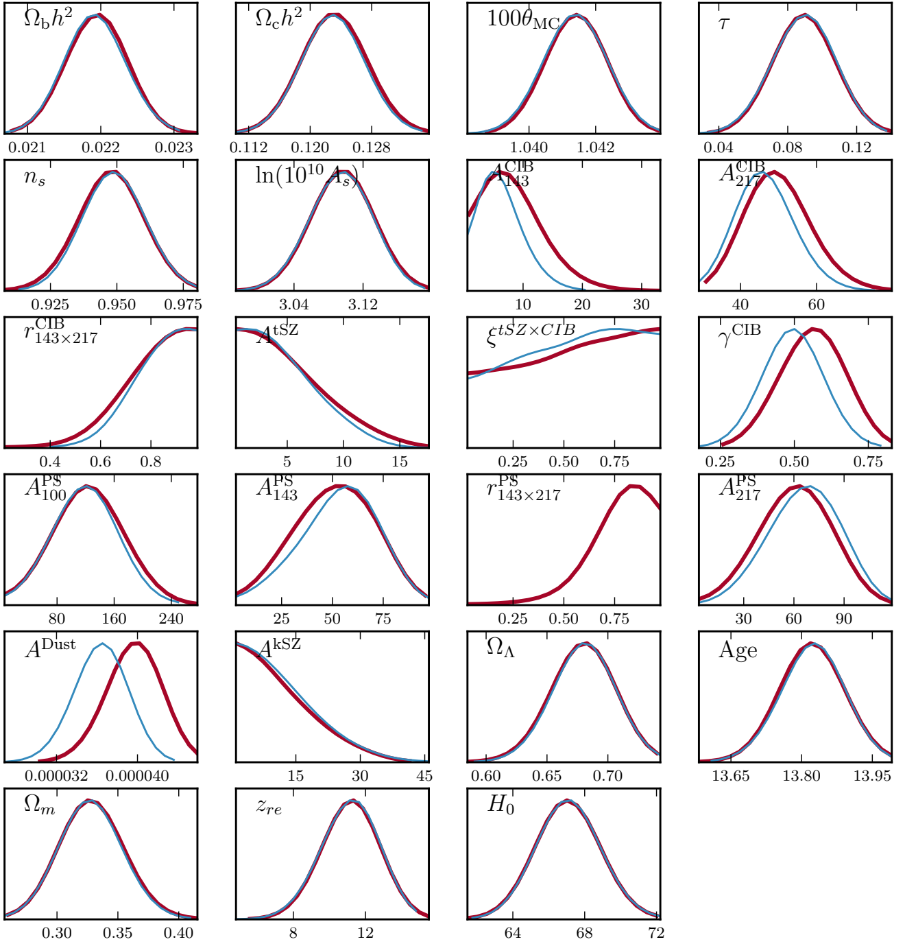
Figure D.4. Impact of changing in the Plik likelihood the minimum multipole from \ell_{\min} = 100 (red, as in reference case) to \ell_{\min} = 50 (blue).
