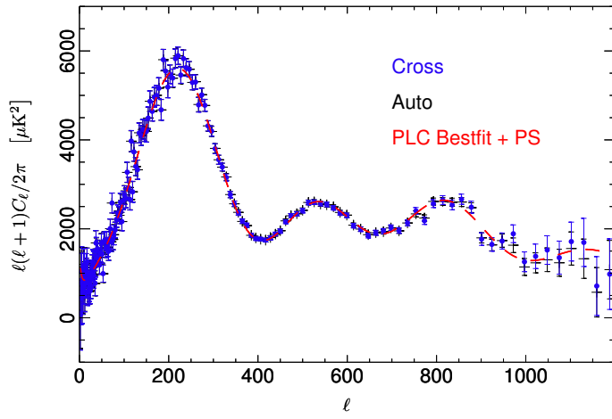
Figure D.9. Power spectrum from the Planck 70 GHz channel, before removal of unresolved sources. Both the auto-spectrum from the 70 GHz maps, and the weighted cross spectra from maps of the three 70 GHz horn pairs are shown. The best-fitting cosmological model from CamSpec, shown for comparison with the best-fitting source power added, gives a good fit to the data.
