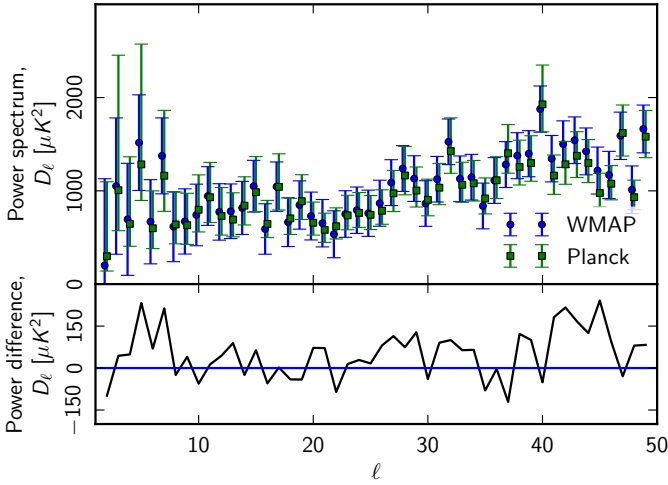
Figure 35. Top: Comparison between the low- \ell Planck temperature power spectrum estimated by Commander and the 9-year WMAP spectrum (Bennett et al. 2013). Error bars indicate 68% confidence regions. Bottom: Difference between the WMAP and Planck low- \ell spectra.
