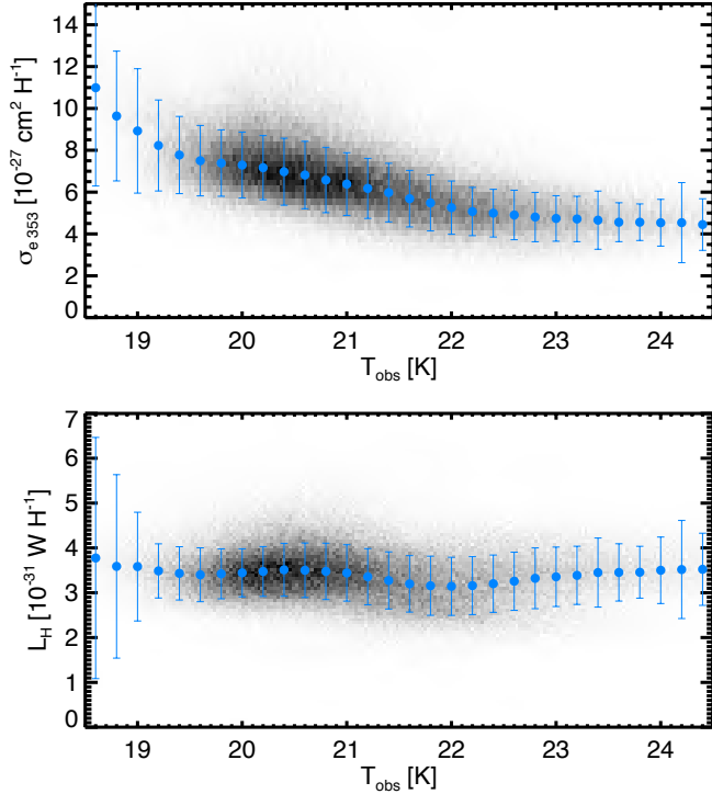
Fig. 19. Variation of \sigma_{e353} ( upper ) and L_H ( lower ) as a function of T_{obs} in the diffuse ISM. Data used were smoothed to 30' , the angular resolution of the HI data. Only pixels where 1 \times 10^{20} < N_{HI} < 2.5 \times 10^{20} \text{ cm}^{-2} were selected. The greyscale shows the point density in the two-dimensional histogram while the blue points indicate the average and standard deviation of L_H and \sigma_{e353} in bins of T_{obs} .
