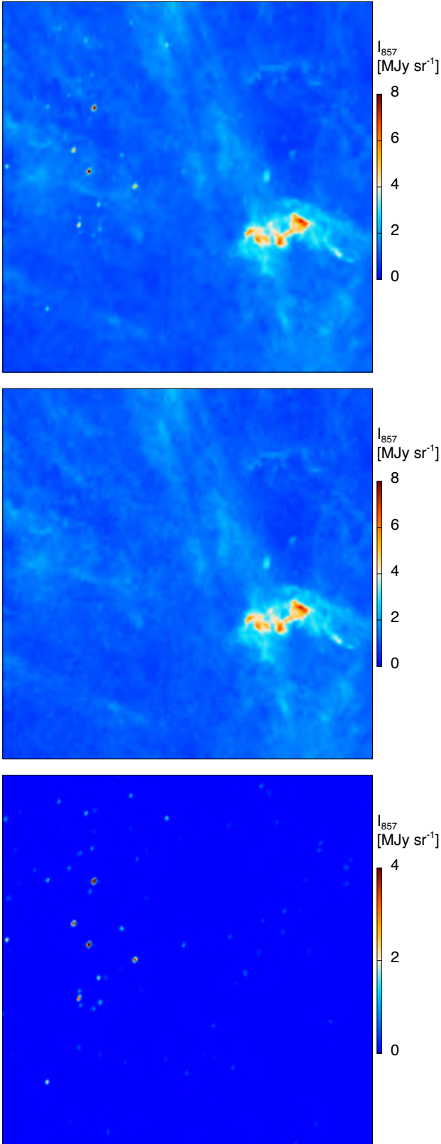
Fig. D.1. Example of the point source removal in a 10^\circ \times 10^\circ region centred on l = 260^\circ , b = 75^\circ ; original map at 857 GHz ( upper ), point source removed map ( middle ), and difference ( lower ).
