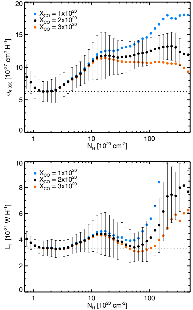
Fig. 20. \sigma_{e353} ( upper ) and L_H ( lower ) vs. N_H computed at 30' resolution from Eq. (13) with three values of X_{CO} : [1, 2, 3] \times 10^{20} \text{ H}_2 \text{ cm}^{-2} \text{ K}^{-1} \text{ km}^{-1} \text{ s} . The mean values of \sigma_{e353} and L_H were computed in bins of N_H equally spaced in log; the error bar is the standard deviation, shown only for X_{CO} = 2 \times 10^{20} \text{ H}_2 \text{ cm}^{-2} \text{ K}^{-1} \text{ km}^{-1} \text{ s} . The horizontal dotted line indicates the average values found in the low N_{HI} mask.
