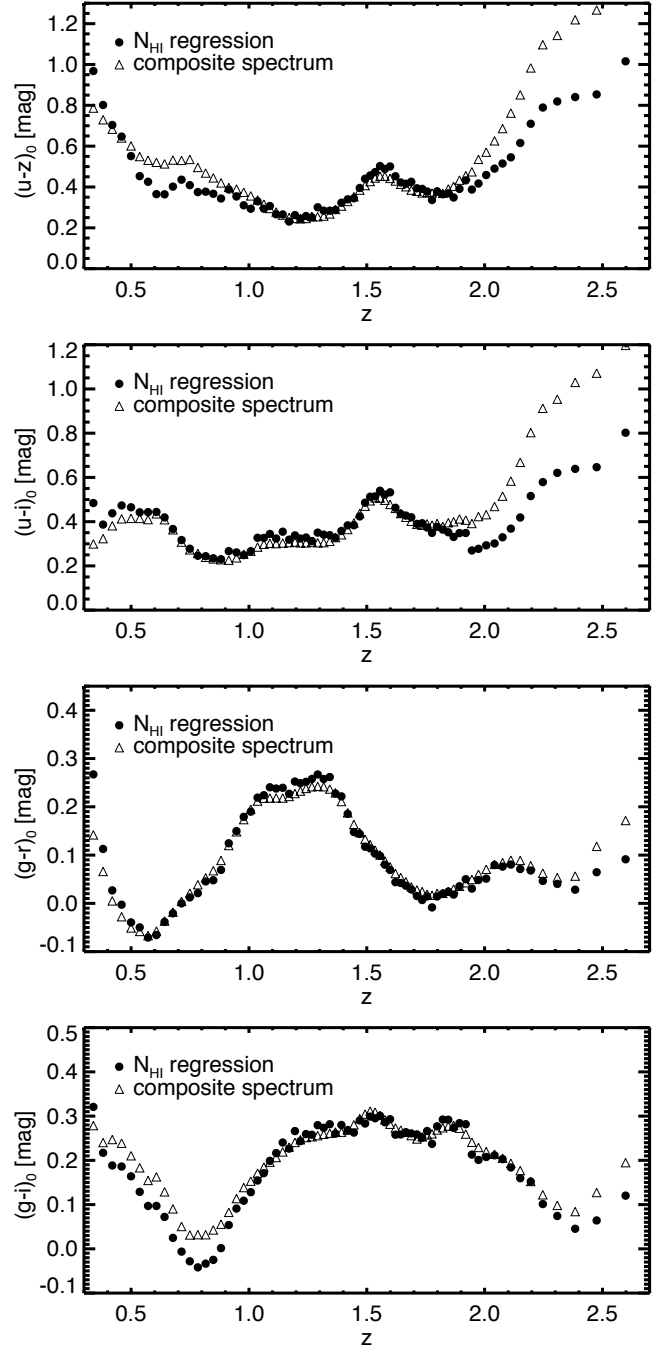
Fig. E.1. Intrinsic colour of quasars as a function of redshift for (u - z) , (u - i) , (g - r) and (g - i) , top to bottom . The black points give the intercept of the (m_X - m_Y) vs. N_{\text{HI}} relation in each bin of redshift (see Eq. (E.7)). The triangles give the intrinsic colour of quasars computed with the composite spectrum (see Eq. (E.8)).
