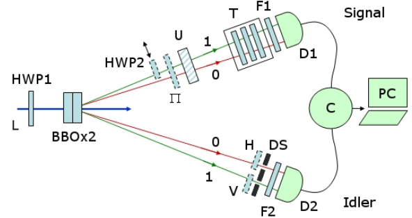
Figure 2. (Color online) Scheme of the apparatus. L is the pump laser, HWP1 and HWP2 are half-wave plates, BBOx2 two BBO crystals, \Pi a polarizer and U is the spatial light modulator. T is the tomographic scheme (a quarter-wave plate, a HWP and a polarizer), H and V denote two polarizers aligned along the horizontal and vertical axes, respectively, DS is the double slit, F1 a high pass filter (780 nm), F2 an interference filter (bandwidth of 10 nm and central wavelength of 810 nm); D1, D2 are detectors and C the coincidences counter. The components drawn with a dashed line have to be modified or moved according to the different stages of the procedure.
