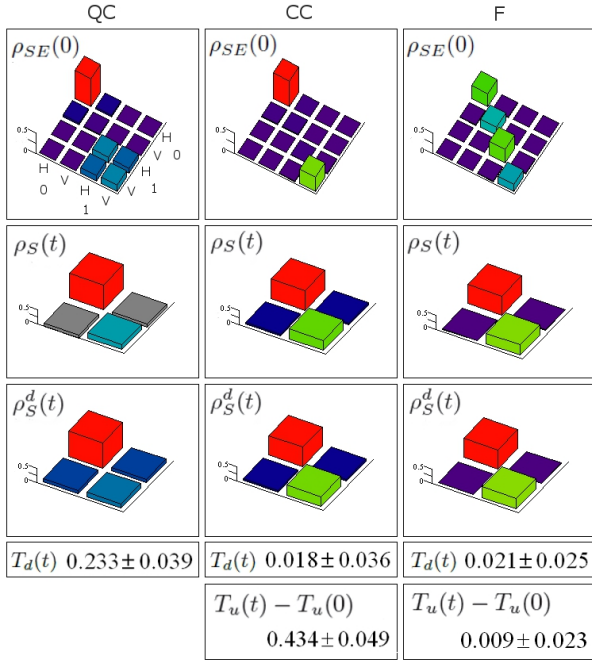
Figure 4. (Color online) Tomographic measurements of the states involved in the experiment. In the left column the case of a state of the form Eq. (6) with \lambda = 0.7 and \theta = \pi/4 has been considered. From top to bottom we have plotted the observed values for \rho_{SE}(0) , \rho_S(t) and \rho_S^d(t) respectively. In the central column we provide the corresponding measurements for the state Eq. (5) with \lambda = 0.64 . The value T_d(t) of the trace distance Eq. (3) is here compatible with zero according to the experimental error, testifying the absence of quantum discord, while the positivity of T_u(t) - T_u(0) given by Eq. (4) shows the detection of classical correlations. In the right column the considered state corresponds to Eq. (7) with \lambda = 0.65 , and the factorized structure of the state is unveiled by the value of T_u(t) - T_u(0) , which is zero within the experimental value. The time specification 0 and t denote the states right after the preparation and the interaction stages respectively.
