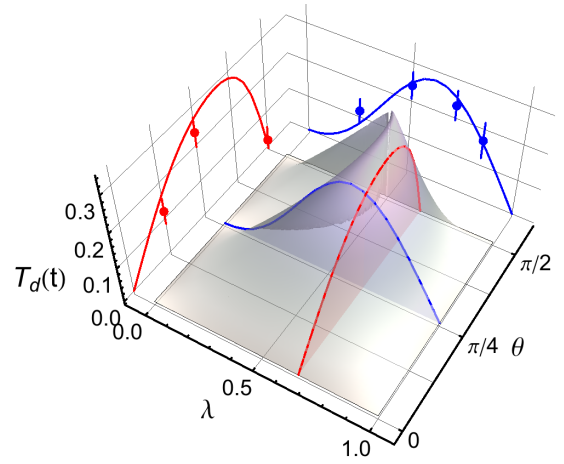
Figure 5. (Color online) Experimental results for the trace distance Eq. (3) corresponding to different values of the parameters \lambda and \theta , as compared to the theoretical prediction given by the smooth surface. The red curve corresponds to \lambda = 0.65 , while the blue curve is fixed by \theta = \pi/4 . The experimental points are plotted on the projected curves to improve their visibility.
