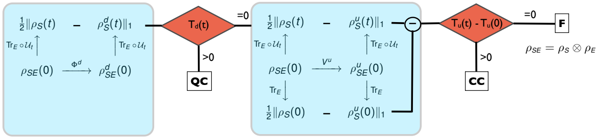
Figure 1. (Color online) Logical scheme of the cascading, two-step procedure exploited to discriminate among quantum correlated (QC), classically correlated (CC) or simply factorized (F) SE states. In the first stage (left box) a dephasing operation \Phi^d which leaves invariant the marginals is applied, allowing to detect quantum correlations using as witness the trace distance T_d(t) between the reduced states evolved from original and dephased state. If no quantum correlations are detected, the second stage (right box) is entered, in which the growth in time of the trace distance of initial states differing by a local unitary operation on the system V^u , i.e. T_u(t) - T_u(0) , allows to detect classical correlations or to conclude that the initial state is factorized. See the text for details.
