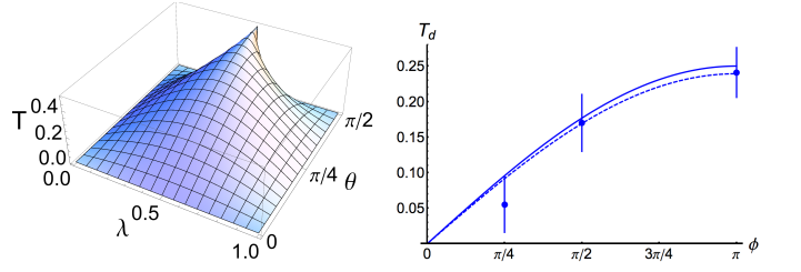
Figure 3. (Color online) (Left) The amount of quantum discord T_d defined in Eq. (2) for a state given in Eq. (6), as a function of \lambda and \theta . (Right) Measured values of T_d for different values of the parameter \phi , which describes the interaction between system and environment. The two points for \phi = \pi/2 and \phi = \pi/4 have been obtained for \lambda = 0.5 , whereas for \phi = \pi we have set \lambda = 0.48 . The solid and dashed lines correspond to \lambda = 0.5 and \lambda = 0.48 , respectively.
