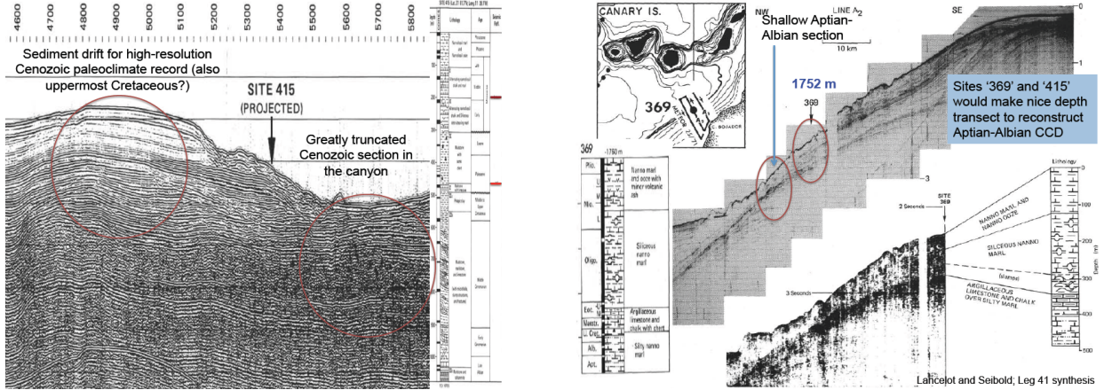
Figure 1. Proposed deep water and slope sites off Morocco. Left: Two deep-water sites adjacent to DSDP Site 415 drilled during DSDP Leg 50. Right: Slope site near DSDP Site 369 drilling during DSDP Leg 41.
