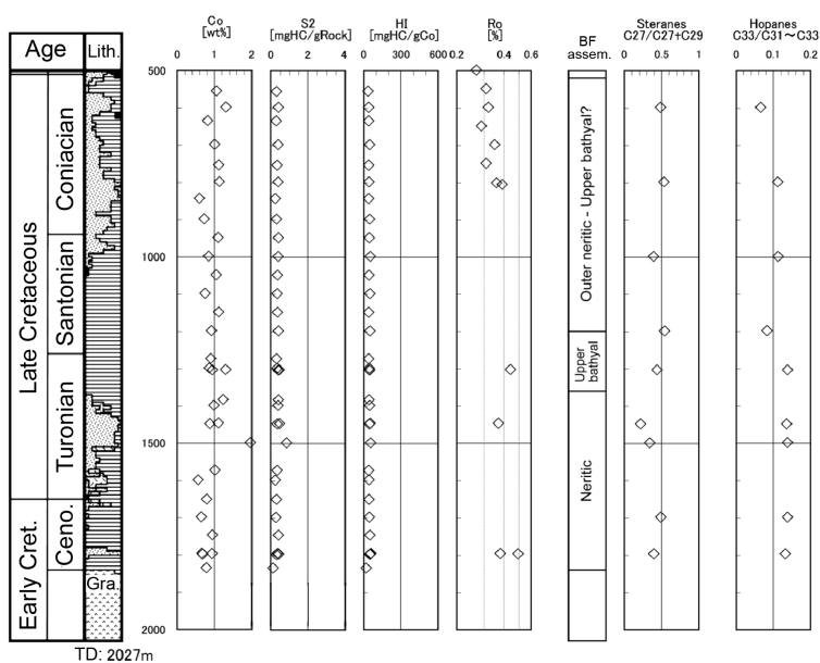
Fig. 1. Organic geochemical stratigraphy of the borehole drilled by Japan Oil, Gas and Metals National Corporation (MITI Off-Kesennuma, in Inaba et al., 2009; Jour. Jap. Ass. Per. Tech, 74, 560-572). Depth is denoted by meter below sea level. Water depth is 230m. Shadings with horizontal lines and dots in lithology represent mudstone and sandstone, respectively. BF assem.; Benthic foraminiferal assemblages. Cret.; Cretaceous. Gra.; Granite. Lith; Lithology. TD; Touchdown depth.
