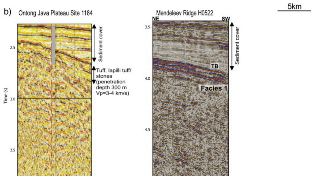
Figure A2. Comparison of seismic character of Mendeleev Ridge and Ontong Java Plateau from Bruvoll et al. (2012).
