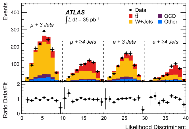
Fig. 5. Untagged analysis: (Top) The distribution of the likelihood discriminant for data superimposed on expectations for signal and backgrounds, scaled to the results of the fit. The left bins correspond to the muon channel and the right bins to the electron channel. (Bottom) The ratio of data to fit result.
