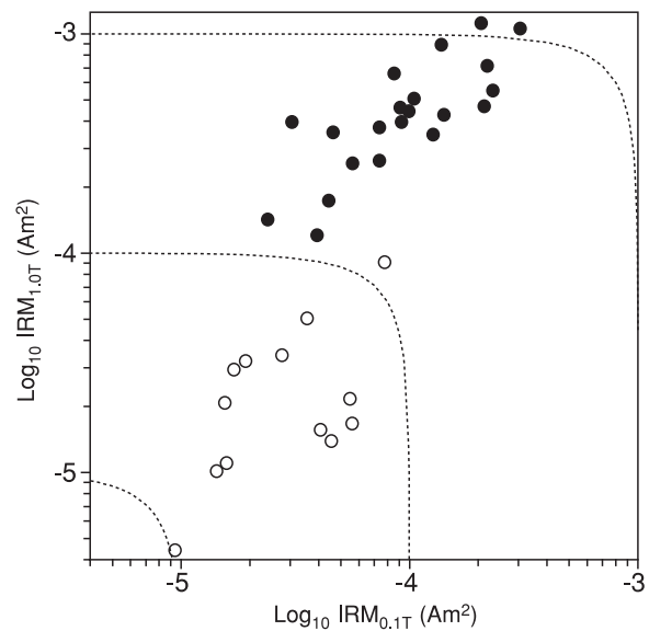
Figure 7. Logarithmic plot of the IRM at 0.1 and 1.0 T for representative red and grey-greenish samples; dotted lines represent equal IRM intensities. Grey-greenish samples (open circles) show generally low IRM values compared to red samples (closed circles); see text for details. [Correction made after online publication 2012 September 20: this figure has been corrected and the caption has been reworded accordingly.]
