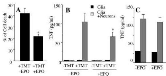
Figure 5. rhEPO prevents neuronal death-induced TNF production in mixed neuron-glia cocultures. (A) Percentage of neural cell death induced by 1 \mu\text{M} TMT without or with treatment with 10 U/ml rhEPO. (B) Release of TNF from glial cells exposed to 1 \mu\text{M} TMT in the presence (gray bars) or absence (black bars) of neurons, with or without 10 U/ml rhEPO. (C) Cytokine production by glial cells exposed to the products of neuronal homogenates with or without rhEPO. Neuronal death, P < 0.05 (Student's t test) versus TMT alone; TNF production, *, P < 0.05 versus neurons plus glia (ANOVA plus Tukey's multiple comparison test). The same experimental conditions were used for the three panels of this experiment.
