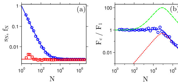
Figure 2. (color online) Analytical expressions and numerical evaluation for \sigma = 10 with a configuration average on 10 realizations as a function of atom number. (a) Results for s_N (blue circles), f_N (red squares) and analytical expressions 1/N + s_\infty (blue line), f_\infty (red line). (b) Forces acting on a cloud of atoms with \Delta_0 = -100\Gamma : numerical evaluation (blue circles) of the average cooperative force. The full lines indicate (i) the force in presence of isotropic scattering, i.e. assuming f_N = 0 (green dashed line), (ii) the force for continuous density distributions without disorder (red dotted line) and (iii) the total force taking into account cooperative scattering and disorder (blue line).
