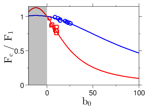
Figure 6. (color online) Experimental data and fits using the cooperative radiation force F_c (normalized to the single atom radiation force F_1 ) in presence of disorder for \Delta_0 = -1.9\Gamma (red squares) and \Delta_0 = -4.2\Gamma (blue circles). The shadowed area corresponds to the non-physical region b_0 < 0 .
