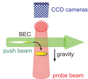
Figure 7. (color online) Scheme of the experiment.
