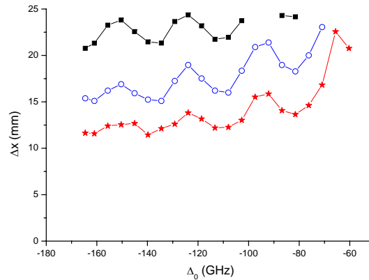
Figure 5. (color online) Displacement of the center of mass of the atomic cloud as a function of detuning for different interaction times: 50ms (red stars), 60ms (open blue circles), 70ms (black squares) obtained for a laser power of P = 100mW .
