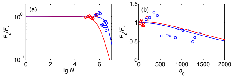
Figure 8. (color online) Blue lines and symbols correspond to T = 1 \mu\text{K} cold thermal clouds (size and shape independent on N ), red ones to condensates in the Thomas-Fermi limit (size and shape depend on N ). (a) Calculated (lines) and measured (symbols) N -dependence of the radiation pressure ratio. (b) Same as (a), but in linear scales and as a function of resonant optical density. The experimental parameters were \Delta_0 = 500 \text{ MHz} , \sigma_{+-\text{pol}} , \tau_0 = 20 \mu\text{s} , \tau_{\text{tof}} = 20 \text{ ms} . No parameter were adjusted. Every data point is an average over several measurements.
