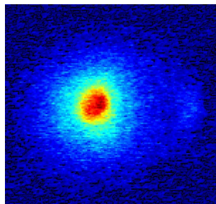
Figure 9. (color online) Absorption images of atomic clouds released from the magnetic trap.
