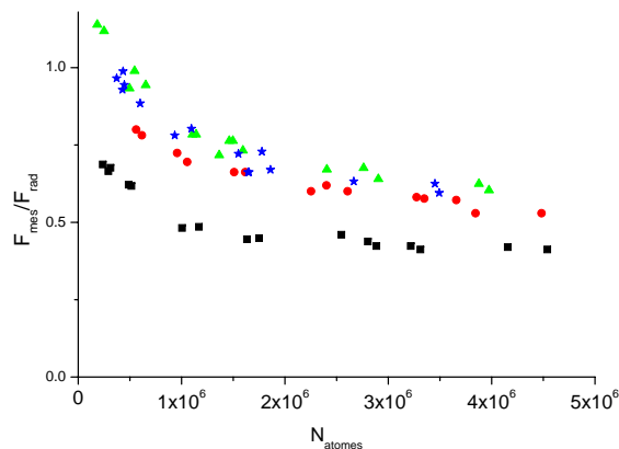
Figure 4. (color online) Average radiation force on the cloud of the atoms. For increasing atom number, the cloud is less displaced by the dipole laser. The interaction time for this experiment is 50\text{ms} , the laser beam power is 100\text{mW} for \Delta_0 = -76\text{GHz} (black square), \Delta_0 = -87\text{GHz} (red circles), \Delta_0 = -90\text{GHz} (green triangles) and \Delta_0 = -108\text{GHz} (blue stars).
