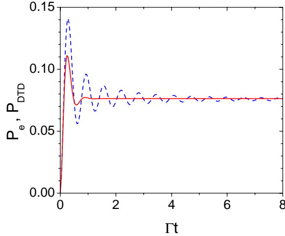
Figure 1. (color online) P_{DTD}(t) = |\beta(t)|^2 (red solid line) and P_e = \sum_j |\tilde{\beta}_j(t)|^2 (blue dashed line) as a function of \Gamma t obtained using the evolution equations (11) and (8), respectively. The simulation parameters are N = 4000 , \sigma = 10 for a gaussian spherical cloud, \Delta_0 = 10\Gamma and \Omega_0 = 0.1\Gamma .
