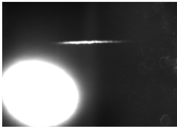
Figure 3. Fluorescence image of the cold atoms. The large cloud corresponds to the free falling atoms and the narrow cigar shaped cloud to atoms trapped in the dipole laser.
