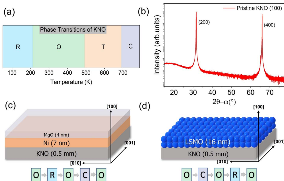
Fig. 1 (a) Temperature-dependent structural phase diagram of KNO crystals, (b) wide 2\theta - \omega scan of pristine KNO (100) in its orthorhombic phase, (c and d) schematic representation of KNO/Ni (c) and (d) KNO/LSMO heterostructures; below them, the thermal treatments of the two systems are shown.
