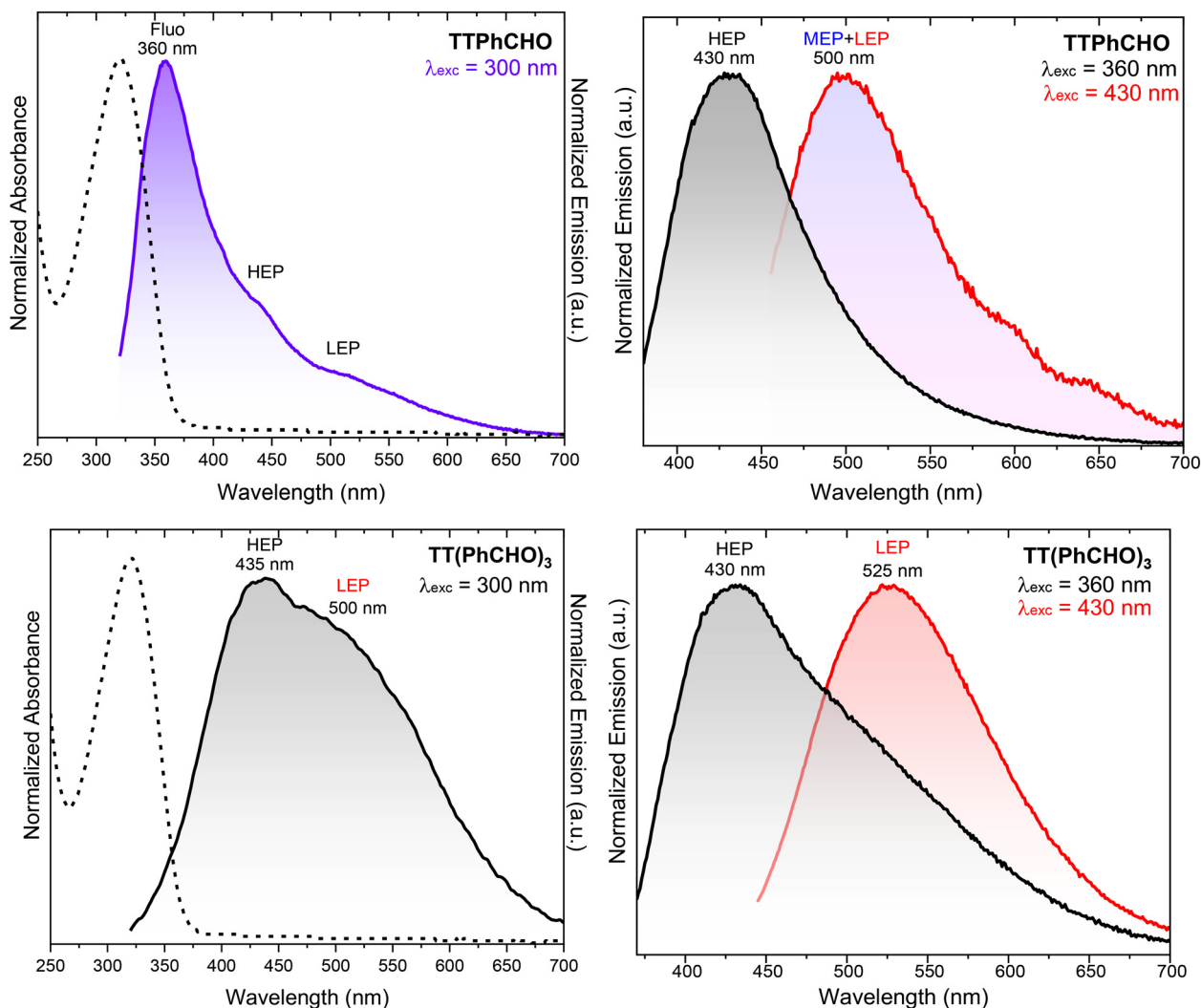
Fig. 2 Normalized Spectra of PMMA film (0.5 w/w%) of TTPhCHO (upper panel) and TT(PhCHO) 3 (bottom panel) at 298 K. Left: absorption (dash lines) and PL emission (full lines, \lambda_{exc} = 300 nm). Right: PL emission at \lambda_{exc} = 360 nm (black lines) and 430 nm (red lines).
