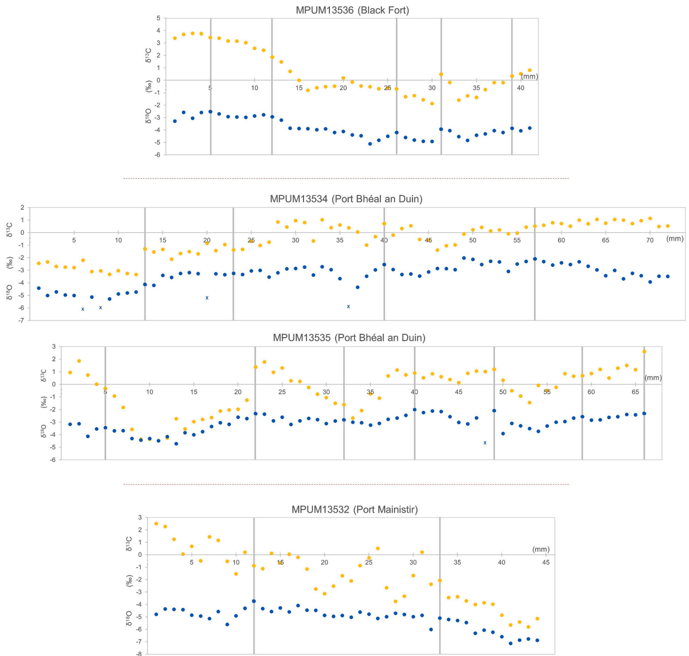
Fig. 12. \delta^{18}\text{O} (blue circles) and \delta^{13}\text{C} (yellow circles) isotope profiles for specimens of Gigantopproductus semiglobosus from Black Fort (AR11–5), Port Bhéal an Duin (AR10–16, AR10–28) and Port Mainistir (AR2–5), Inishmore. Grey vertical lines represent the position of the growth lines. Blue crosses are outlier values not considered in the seasonal reconstruction. (For interpretation of the references to colour in this figure legend, the reader is referred to the web version of this article.)
