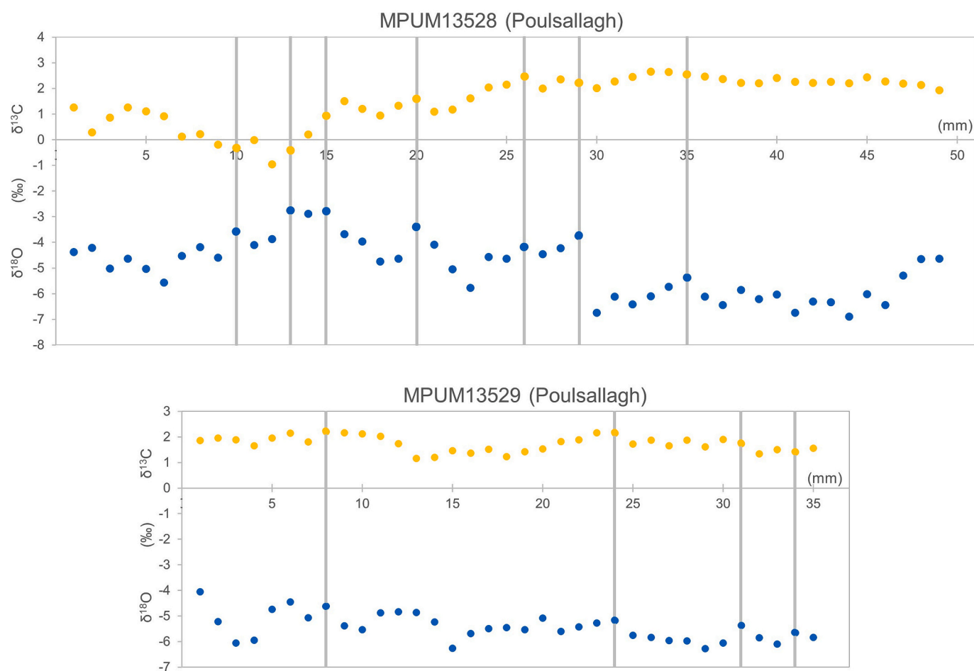
Fig. 11. \delta^{18}\text{O} (blue circles) and \delta^{13}\text{C} (yellow circles) isotope profiles for specimens of Gigantoproductus semiglobosus from Poulsallagh, Burren Region. Grey vertical lines represent the position of the growth lines. (For interpretation of the references to colour in this figure legend, the reader is referred to the web version of this article.)
