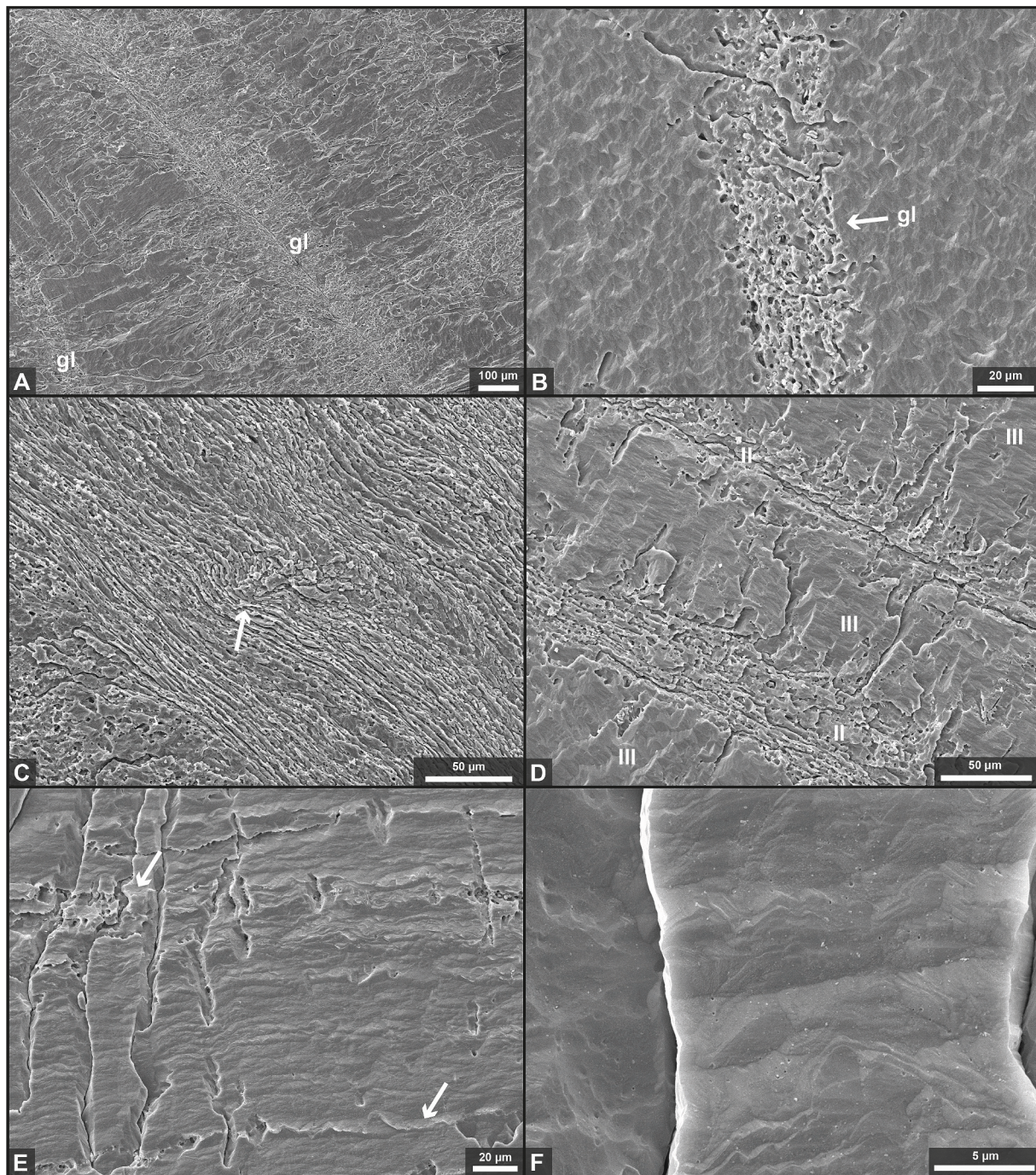
Fig. 9. SEM images showing the shell microstructure of Gigantoproductus semiglobosus (Part 2). A) MPUM13534, growth lines (gl) in the columnar tertiary layer; B) MPUM13535, details of a growth line (gl) in the columnar tertiary layer; C) MPUM13535, laminar secondary layer with pseudopuncta (white arrow); D) MPUM13536, intercalations of laminar secondary layer (II) and columnar tertiary layer (III); E) MPUM13536, growth steps inside the columns of the tertiary layer, some major growth lines are also visible (white arrows); F) MPUM13536, growth stages inside each column of the tertiary layer with thin accretionary lines which may represent diurnal growth banding.
