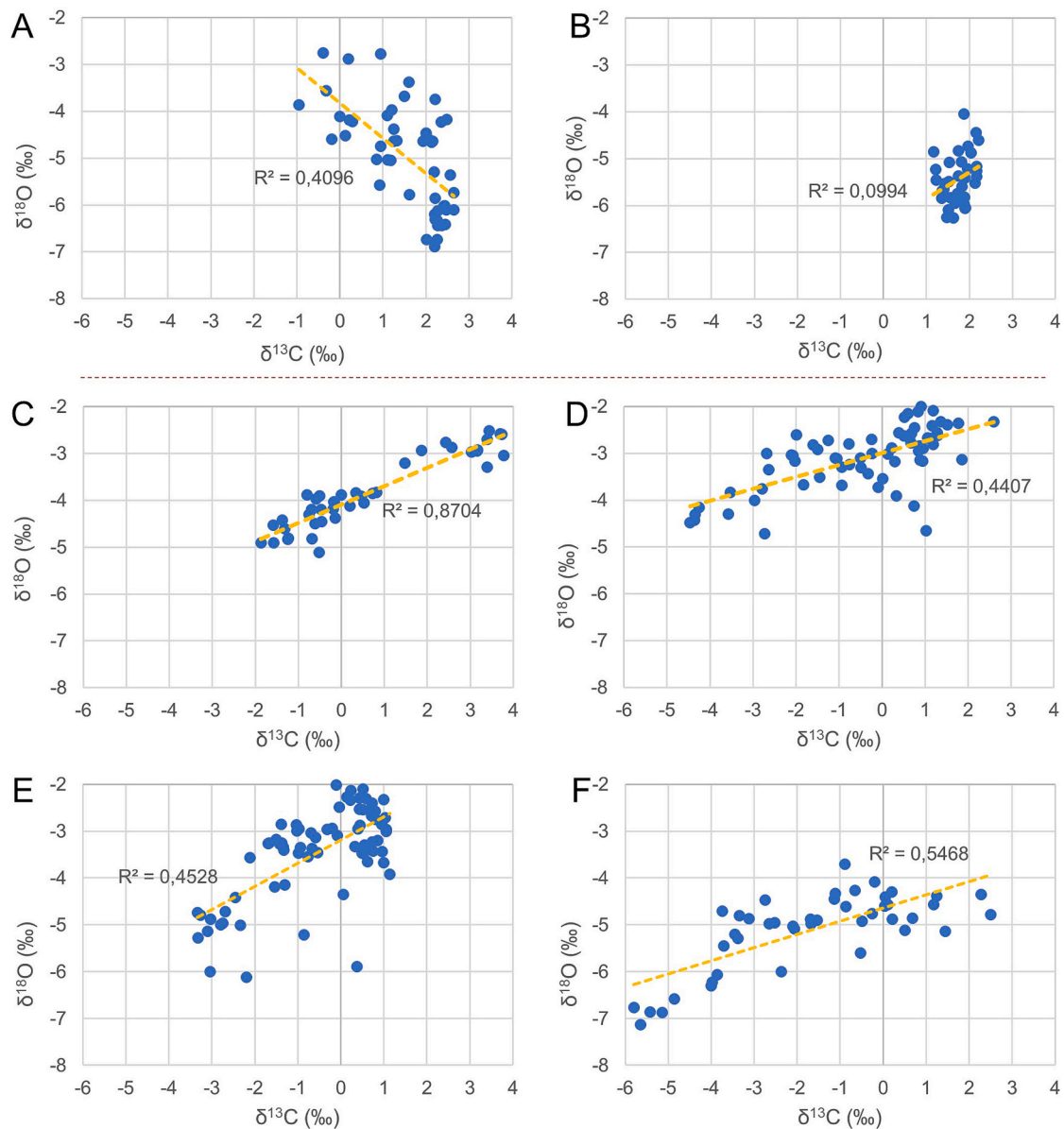
Fig. 13. Cross-plot diagrams of \delta^{18}\text{O} and \delta^{13}\text{C} with linear regression line and R^2 coefficient. A) Specimen MPUM13528, Poulsallagh, Burren; B) Specimen MPUM13529, Poulsallagh, Burren; C) Specimen MPUM13536, Black Fort, Inishmore; D) Specimen MPUM13535, Port Bhéal an Duin, Inishmore; E) Specimen MPUM13534, Port Bhéal an Duin, Inishmore; F) Specimen MPUM13532, Port Mainistir, Inishmore. The correlation is positive in except for A. It is statistically significant ( p < 0.05 ), in all except for B.
