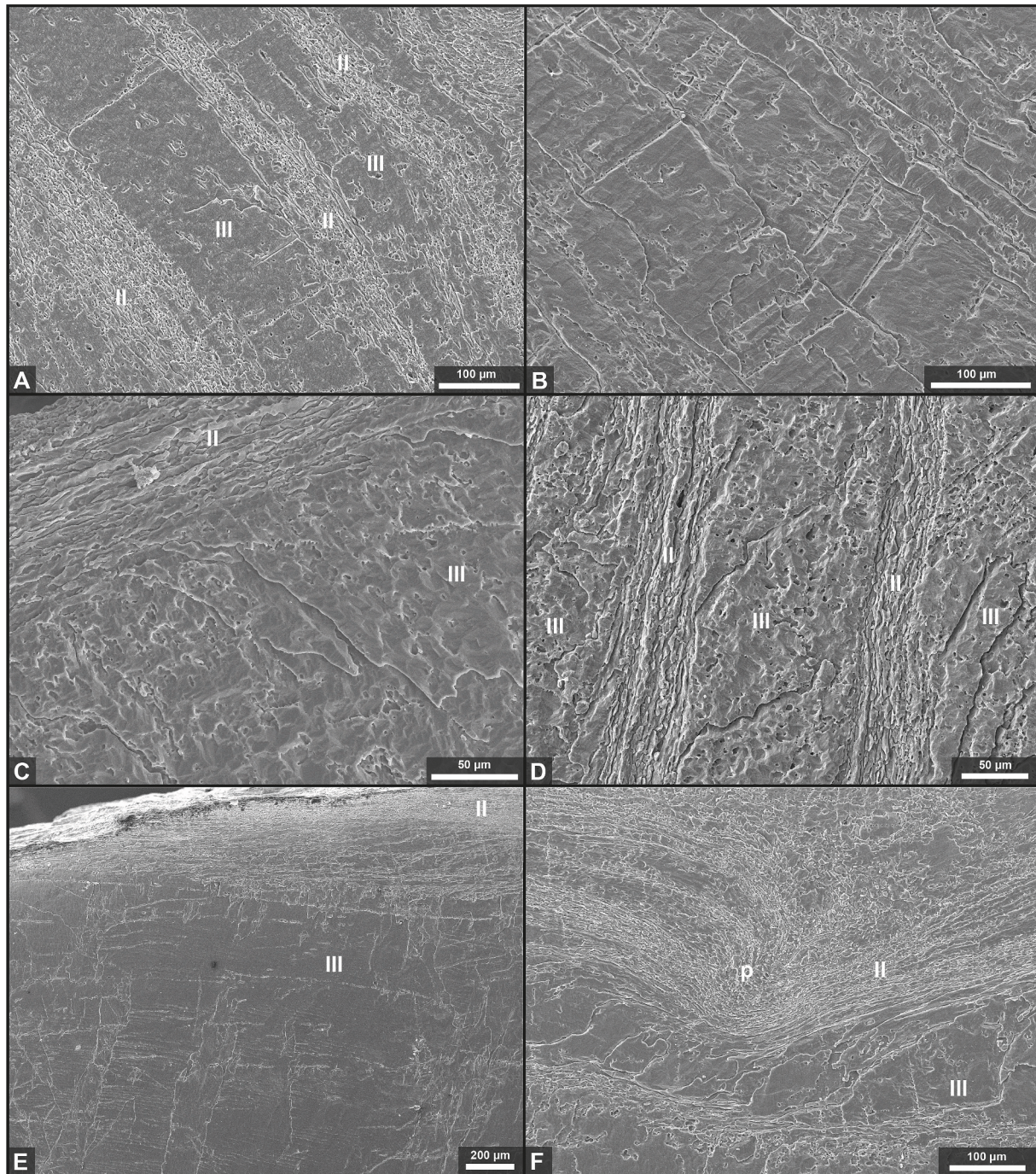
Fig. 8. SEM images showing the shell microstructure of Gigantoproductus semiglobosus (Part 1). A) MPUM13522, intercalations of laminar secondary layer (II) and columnar tertiary layer (III); B) MPUM13528, well-preserved columnar tertiary layer; C) MPUM13529, microstructural succession of the outermost part of the shell consisting of laminar secondary layer (II) with minor alteration in the form of laminae coalescence, and columnar tertiary layer (III); D) MPUM13530, intercalations of laminar secondary layer (II) and columnar tertiary layer (III); E) MPUM13532, microstructural succession of the shell consisting of laminar secondary layer (II) and columnar tertiary layer (III); F) MPUM13532, pseudopuncta (p) close to the transition between laminar secondary layer (II) and columnar tertiary layer (III).
