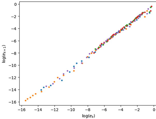
Fig. 1 Estimates for the order of convergence of \left| \frac{f(W)}{|W|^3} - \frac{\sqrt{6}}{4} \right| for n = 5 . Here, \log(e_k) = \log \left| \frac{f(W_k)}{|W_k|^3} - \frac{\sqrt{6}}{4} \right| , where W_k is the iteration at the k -th step. The scale of both axes are logarithmic
