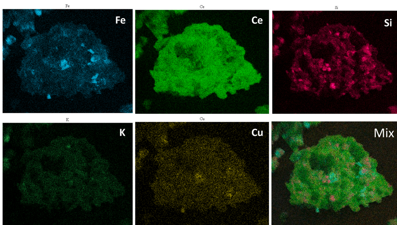
Fig. 1. Detailed SEM-EDX representation of Fe/Ce/SiO 2 -K,Cu and mix of all the elements, x750 magnification, 10 \mu m scale.
