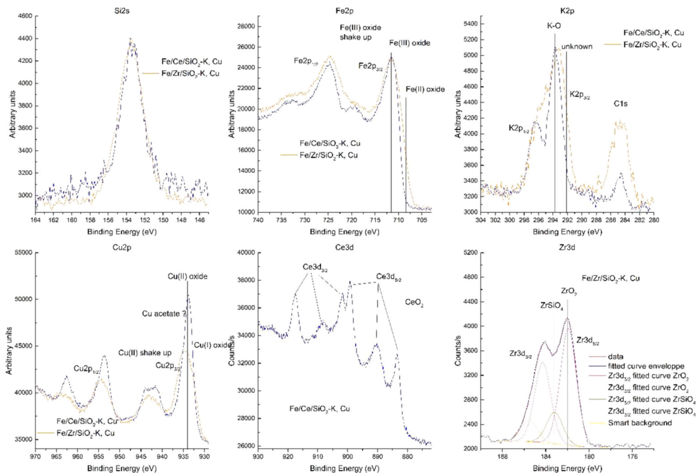
Fig. 17. High resolution spectra for catalysts a) Fe/Ce/SiO 2 -K,Cu (blue line) and b) Fe/Zr/SiO 2 -K,Cu (orange line). The intensity for spectra Si2s, Fe2p, K2p, and Cu2p was normalized to maximum intensity to ease comparison of spectral shape.
