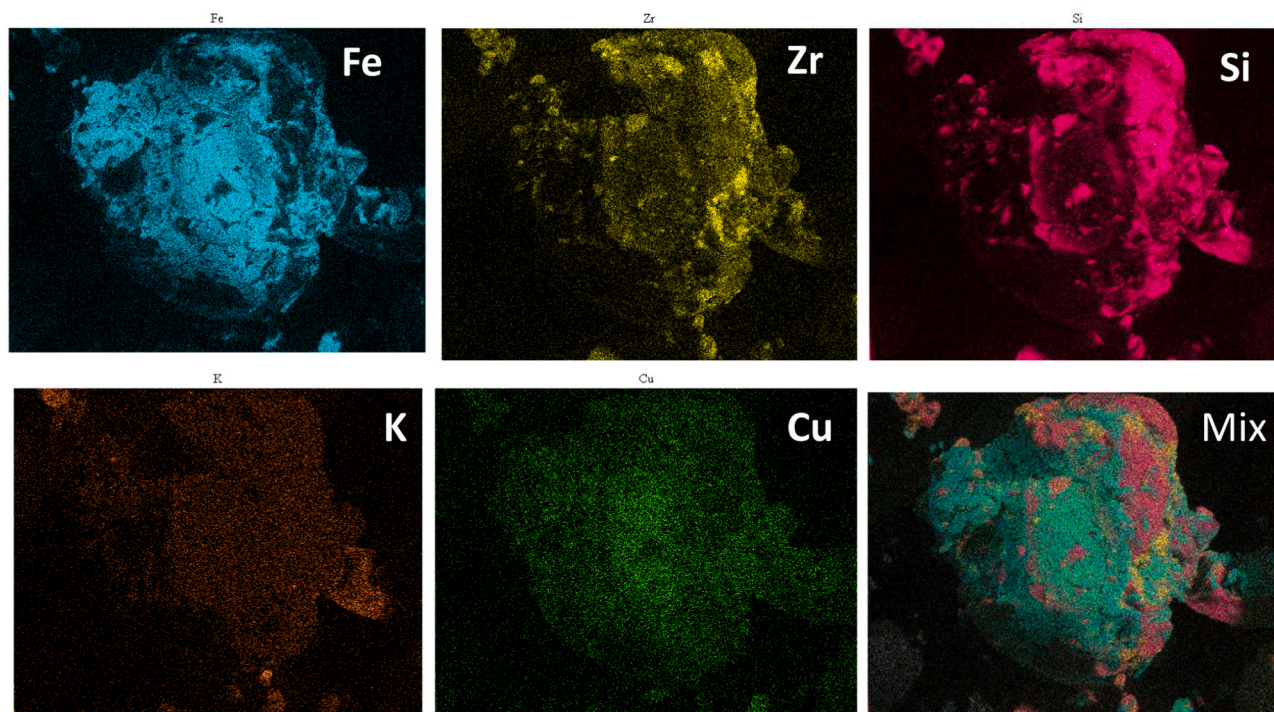
Fig. 2. Detailed SEM-EDX representation of Fe/Zr/SiO 2 -K,Cu and mix of all the elements, x270 magnification, 10 \mu m scale.
