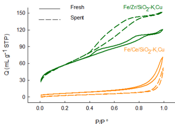
Fig. 6. BET adsorption-desorption isotherms of both Fe/Ce/ \text{SiO}_2 -K,Cu and Fe/Zr/ \text{SiO}_2 -K,Cu fresh and spent.
