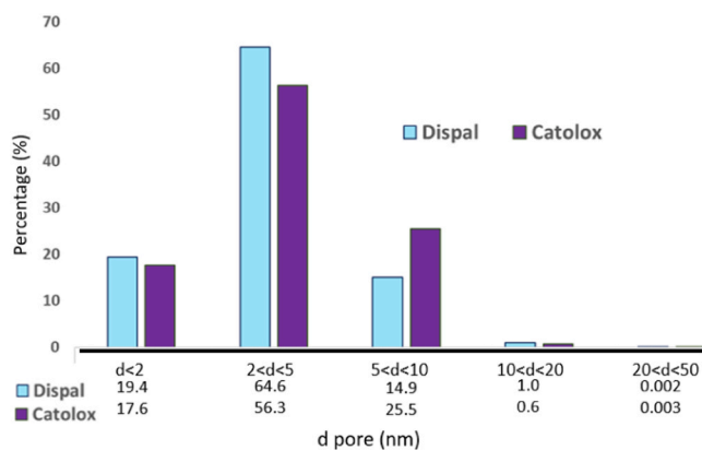
Fig. 8. The pore size distributions from d < 2 \text{ nm} and 100 \text{ nm} < d for Fe/Catalox-K,Cu-purple, Fe/Dispal-K,Cu-turquoise.
