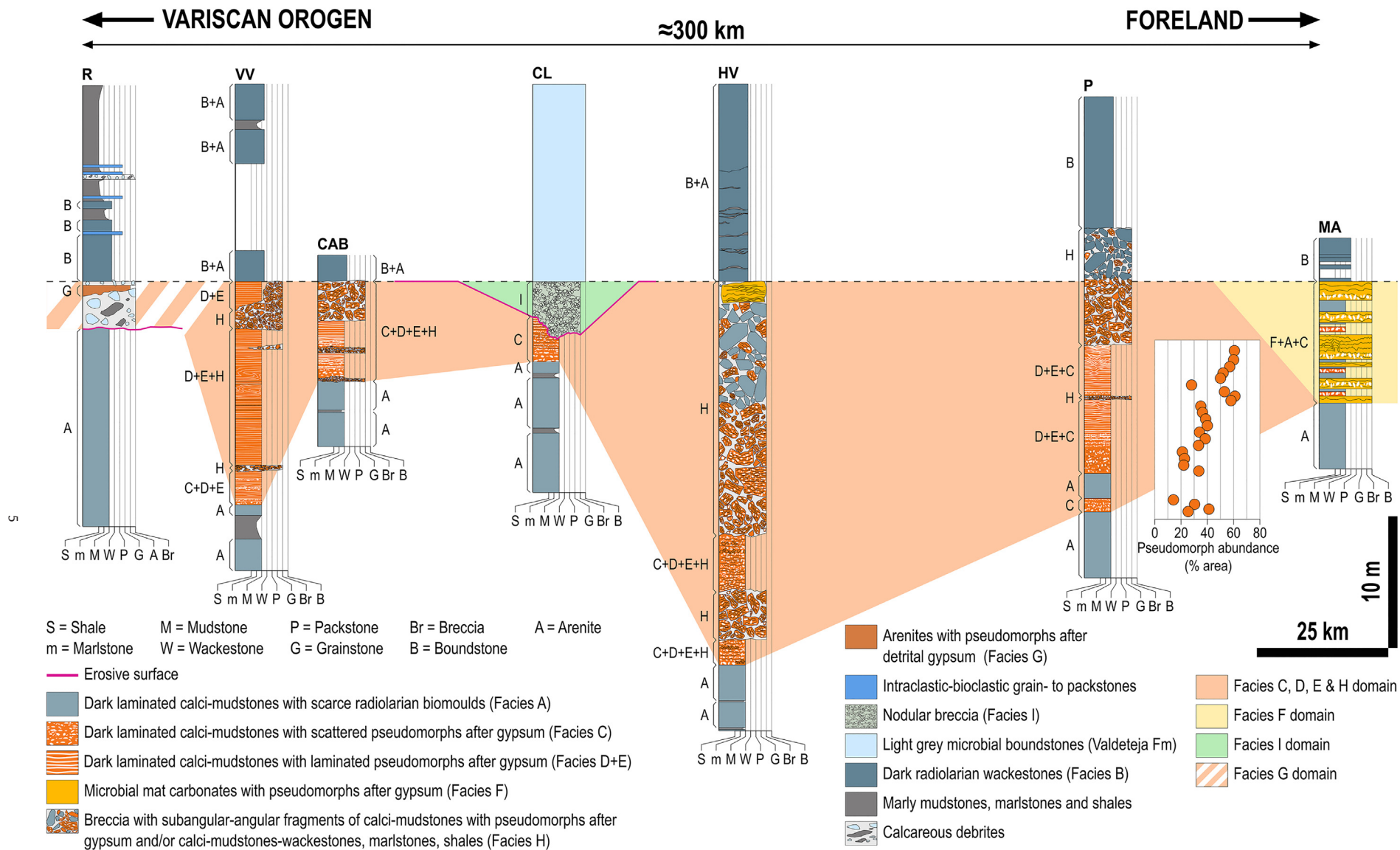
Fig. 4. Correlation of the sedimentary facies of the upper part of the Barcaliente Fm and the overlying deposits along the cross section shown in Fig. 3B. A log of the estimated abundance of calcite and quartz pseudomorphs after gypsum is shown for the Porma Reservoir section (P).
