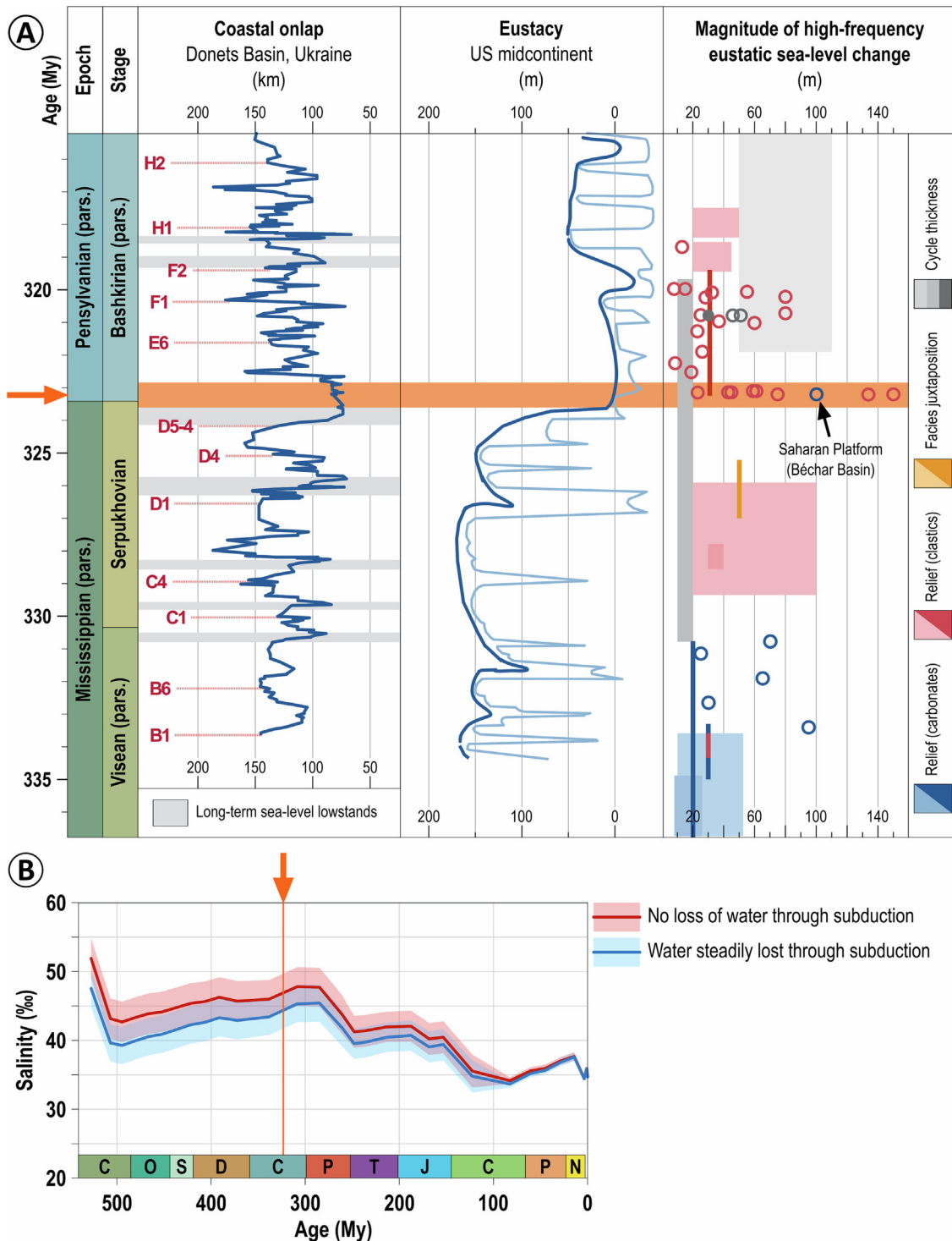
Fig. 16. A) Coastal onlap in the Donets Basin (Eros et al., 2012) and in the US Midcontinent (Ross and Ross, 1987), and amplitude of high-frequency sea-level glacio-eustasy from Middle Mississippian to Early Pennsylvanian times (Rygel et al., 2008). Redrawn from Montañez and Poulsen (2013). Gypsum deposits of Barcaliente Fm and equivalent stratigraphic units (orange arrow) are coeval with the major sea-level fall recorded in Donets Basin, US Midcontinent and other basins from around the world (orange area). B) Evolution of seawater salinities for the Phanerozoic Eon after Hay et al. (2006). Estimated mean seawater salinities for the mid-Carboniferous could have been as high as 45 ‰; the orange arrow indicates the inferred age of the studied evaporite interval.
