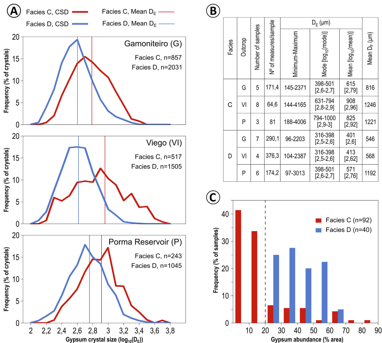
Fig. 9. A) Histograms of crystal size distribution (CSD) of the calcite and quartz pseudomorphs obtained by area counting procedure in samples of facies C and D from Gamoniteiro (G), Viego (VI) and Porma Reservoir (P) sections (see Fig. 4A for location). B) Synthetic table showing calculated area equivalent diameter ( D_E ; range, mode and mean values) and mean Feret diameter ( D_F , calliper or b axis) of the pseudomorphs calculated for samples of facies C and D of the aforementioned sections. C) Histogram showing pseudomorph abundance (% of area) and frequency (% of samples) in facies C and D (including samples from all the studied sections). Quantification was made by visual estimation and point and area counting procedures. Note that samples from facies C show generally pseudomorph abundances \leq 20\% , whereas abundances from facies D overcome 20\% .
