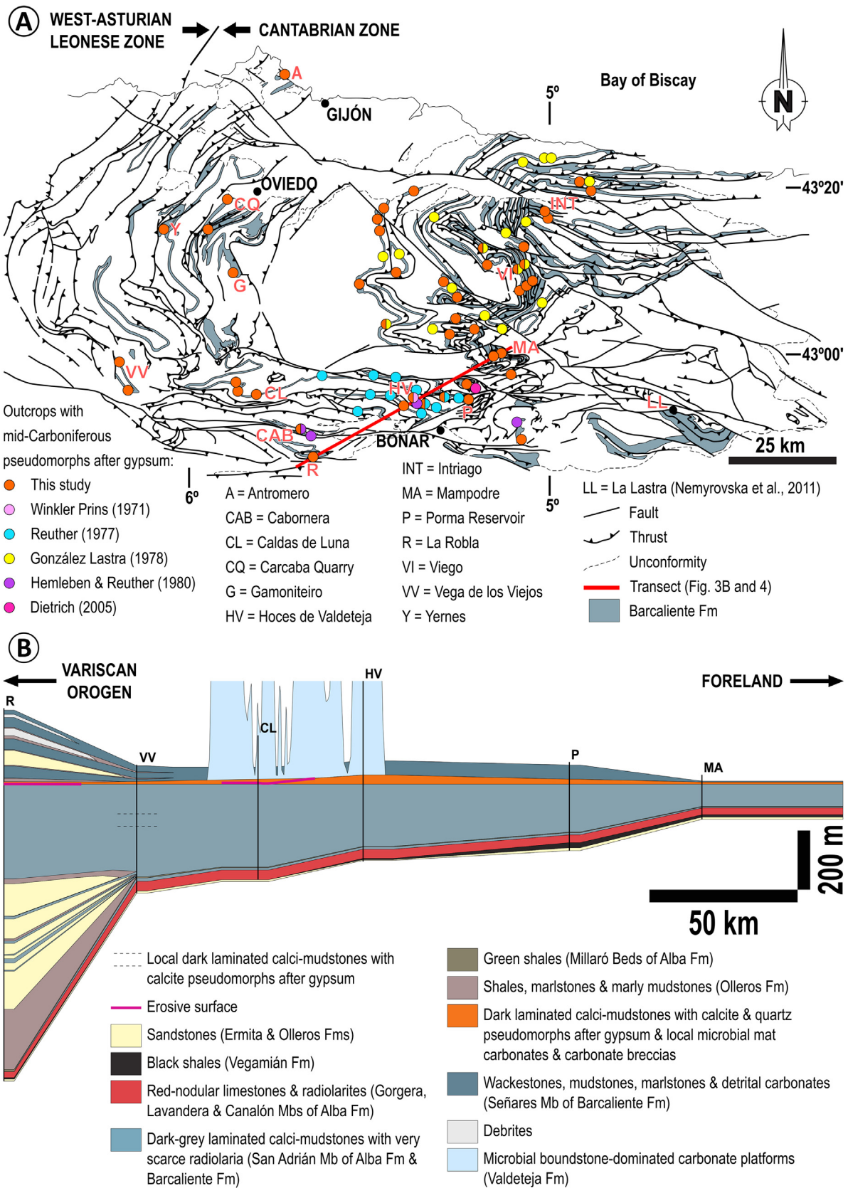
Fig. 3. A) Synthetic map of the CZ showing the areal distribution of the Barcaliente Formation and the localities in which calcite and quartz pseudomorphs after gypsum have been observed or reported in the literature (see Winkler Prins, 1971; Reuther, 1977; González Lastra, 1978; Hemleben and Reuther, 1980; Dietrich, 2005). B) Stratigraphic cross section showing the Mississippian and Early Pennsylvanian succession of the southern branch of the CZ (see location in A, red line).
