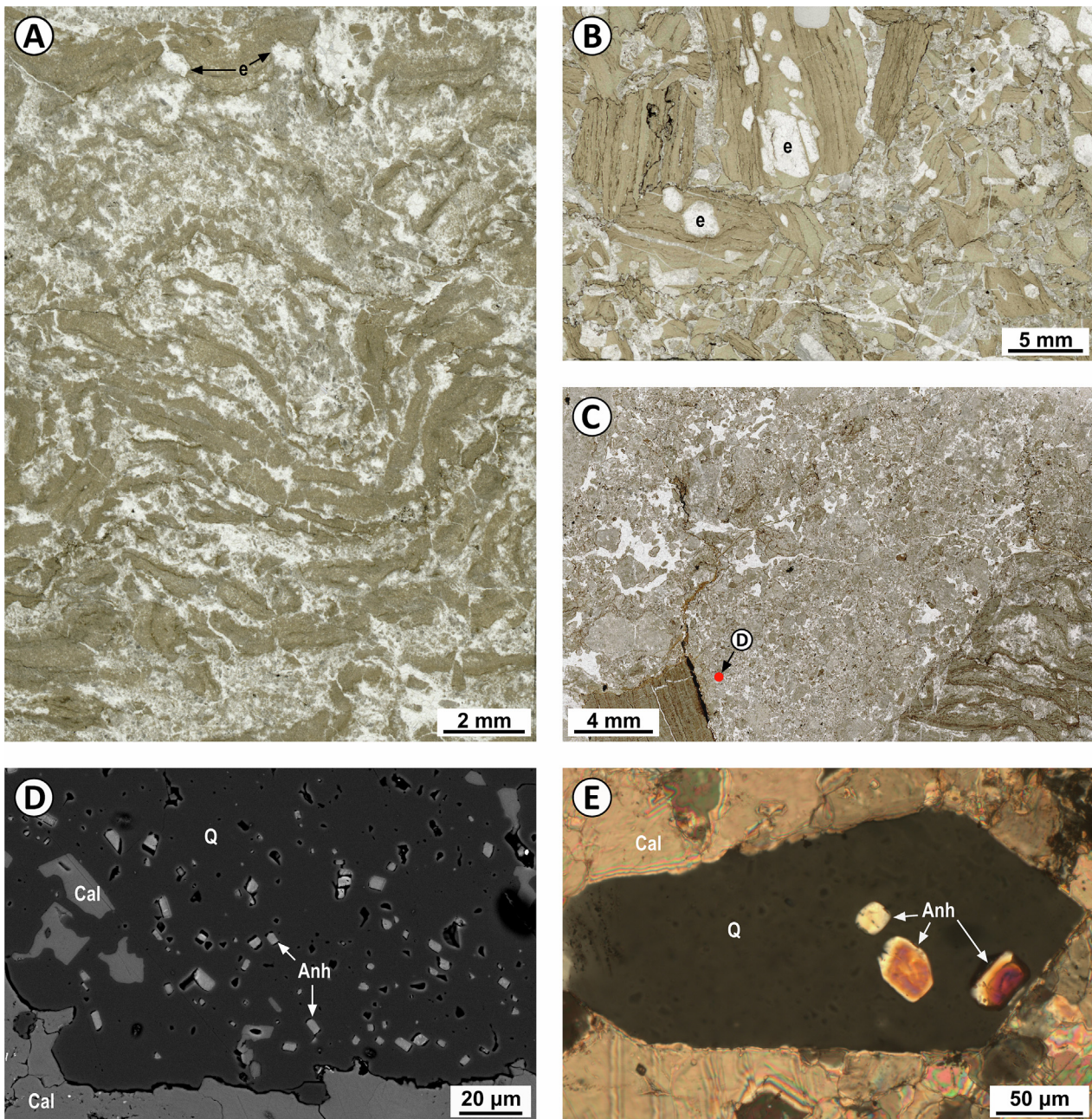
Fig. 13. A–C) Scanned thin sections of facies H consisting of breccia fragments composed of micritic limestone with calcite pseudomorphs after gypsum (e), embedded within a matrix composed of submillimetre-sized microsparitic limestone fragments and cloudy spar. D) SEM image (backscattered electrons) showing a detail of the matrix shown in image C with common quartz replacements (Q). Quartz contains numerous rectangular solid inclusions of anhydrite (Anh) and corroded calcite (Cal). Mineralogy was confirmed by EDS analyses. E) Transmitted light photomicrograph of a quartz replacement (Q) affecting the breccia matrix composed by calcite (Cal). Quartz shows solid inclusions of anhydrite (Anh).
