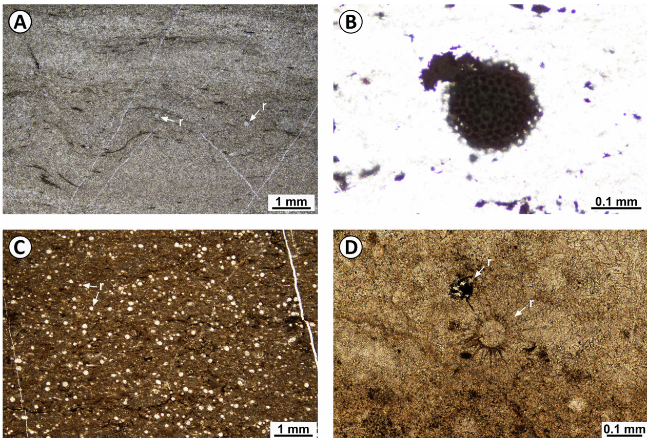
Fig. 7. Transmitted light photomicrographs of facies A and B. A) Burrowed calci-mudstone with disperse calcite biomoulds of radiolaria (r) (facies A). B) Pyritised radiolarian test preserving the internal structure (facies A). C) Dark-grey radiolarian wackestones (facies B) with abundant radiolarian biomoulds (r). D) Close-up view of radiolarian tests (r) preserving some of their spines in facies B.
