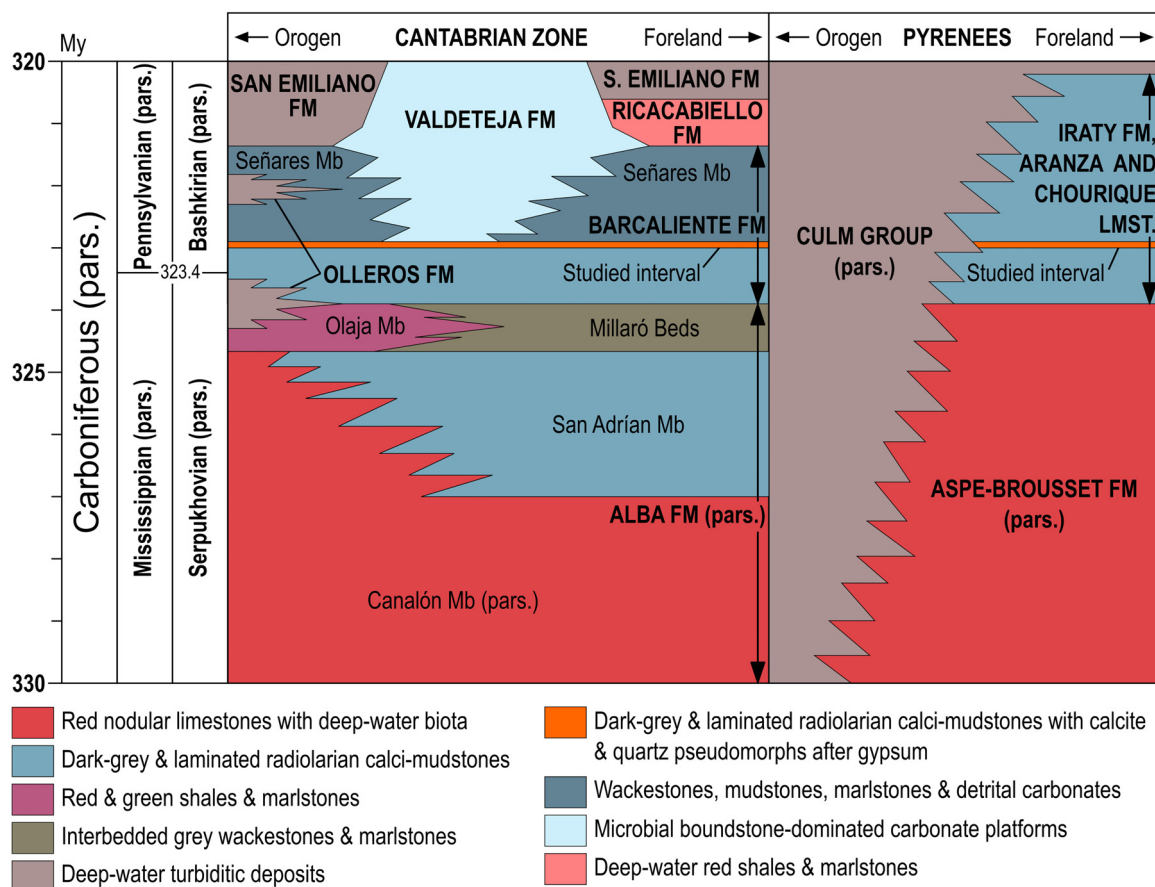
Fig. 2. Chronostratigraphic diagram for mid-Carboniferous strata of the CZ and Pyrenees. Modified from Sanz-López and Blanco-Ferrera (2012), Merino-Tomé et al. (2017, 2019), Cózar et al. (2018) and Sanz-López (2019).
