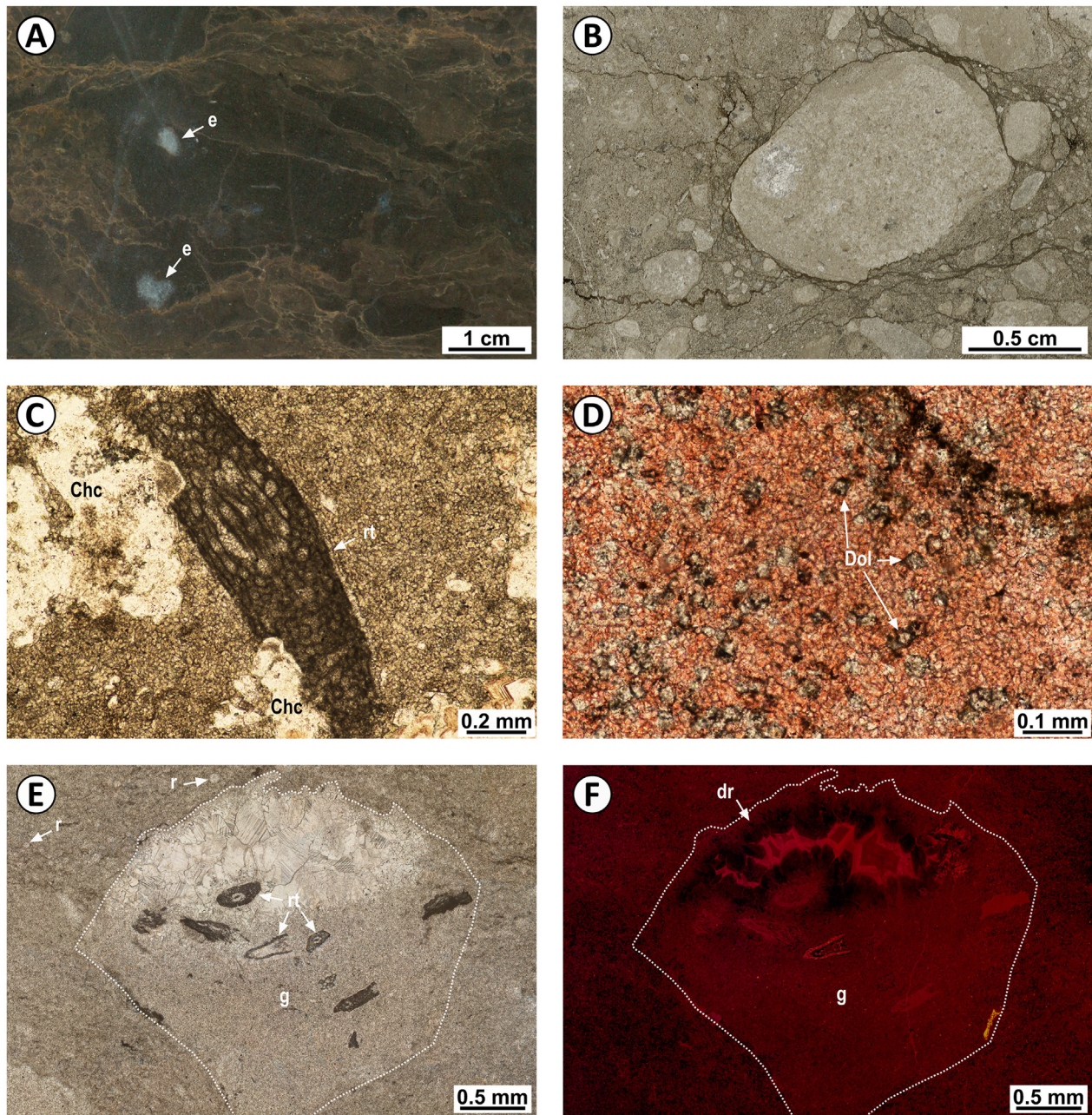
Fig. 14. A and B) Scanned polished slab (image A) and thin section (image B) of facies I, a nodular breccia with centimetre-sized carbonate intraclasts with scattered calcite pseudomorphs after gypsum (e). Note sutured contacts of intraclasts, abundant stylolitic surfaces and common gradual contacts between the clasts and the matrix, which are characteristic features of orthic nodules. C) Photomicrograph of the breccia matrix showing a root fragment (rt). Cell walls of the plant root tissues are replaced by micrite allowing the recognition of the xylem and the floem. Chalcedony (Chc) masses replace partially the matrix and the root fragment. D) Photomicrograph of microsparitic matrix from a stained thin section exhibiting dolomite crystals (Dol) within the calcite matrix. E and F) Transmitted light (image E) and cathodoluminescence (image F) photomicrographs from a stratum underlying facies I, which is composed by mudstone with scattered calcite pseudomorphs after evaporites (facies C). Note that the lower part of the evaporite mould shows microsparite geopetal infill (g) with numerous root fragments (rt) and the upper part of the mould is filled by a banded drusy calcite cement (dr). The surrounding microsparitic matrix, which shows few radiolarian biomoulds (r), is blotchy and poorly luminescent, whereas the microsparite of the geopetal infill shows brighter luminescence.
