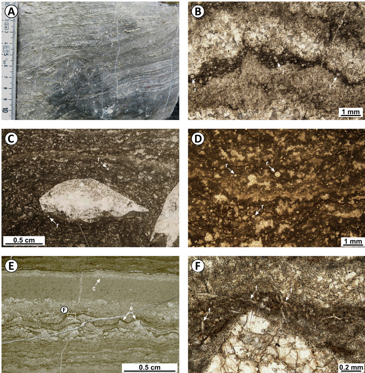
Fig. 11. A) Outcrop image of subfacies F1 showing crinkly lamination. B–D) Transmitted light photomicrographs of subfacies F1. B) Dark micritic–microsparitic laminae with abundant radiolarian biomoulds and pores cemented by blocky calcite. C) Laminated microsparite with common radiolarian biomoulds (r) showing small, elongated pores parallel to lamination and cm-sized calcite pseudomorphs after lenticular gypsum (e). D) Detail of the microsparitic matrix of subfacies F1 that shows irregular porosities sub-parallel to lamination and contains radiolarian biomoulds (r). E) Scanned thin section of facies F2 showing calcite pseudomorphs of bottom-grown gypsum crystals (e), which show subhedral habits at the top of the laminae. Note the potential pseudomorphs after cumulates (c) near the top of the image. F) Detail of image E showing a calcite pseudomorph (e) after a bottom-grown gypsum crystal overlain by a dark micrite–microspar lamina with filamentous structures (f) resembling microbe moulds.
