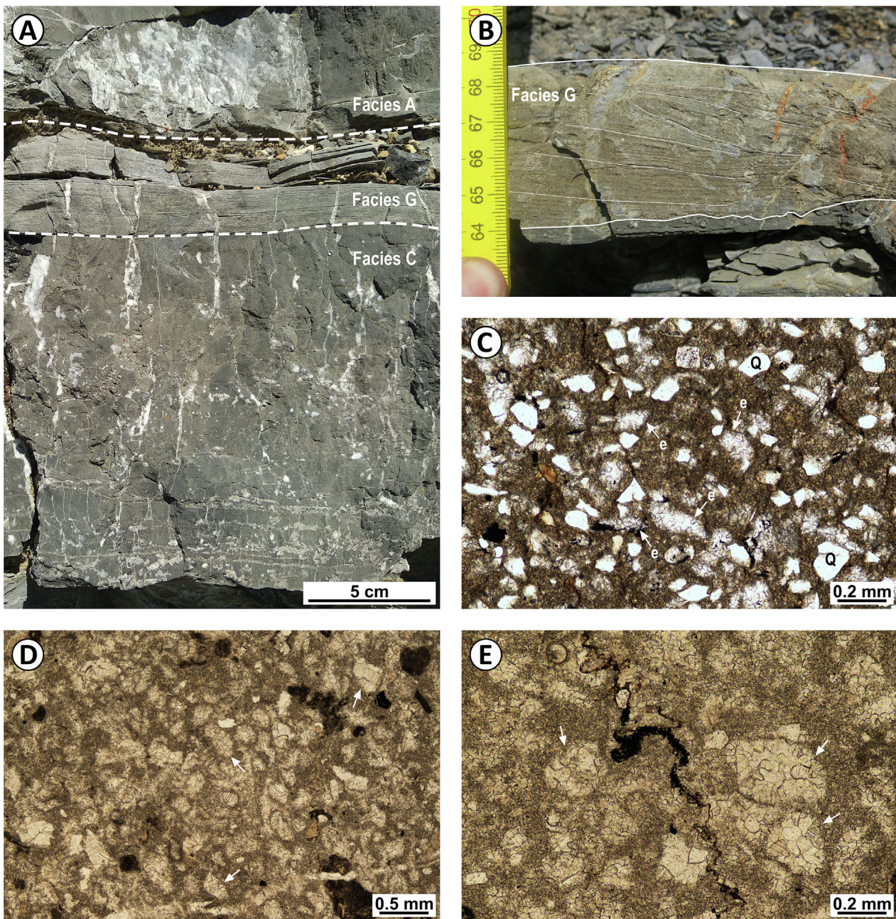
Fig. 12. A) Centimetre-thick, medium to fine sand-grained arenite layer (facies G), interbedded with dark-grey calciludstones (facies A) and calciludstones with scattered calcite pseudomorphs after intrasediment gypsum (facies C). B) Centimetre-thick arenite layer (facies G) with irregular erosive base and ripple cross-lamination. C–E) Transmitted-light photomicrographs of arenites with calcite pseudomorphs after detrital gypsum (facies G). C) Detail of the arenite shown in image A. Main components include sand-sized quartz grains (Q) and calcite pseudomorphs after detrital gypsum grains (e) showing abraded sub-euhedral monoclinic and lenticular habits. D and E) Arenites mainly composed of calcareous grains and calcite pseudomorphs after abraded grains with sub-euhedral and lenticular morphologies (white arrows), interpreted as being originally detrital gypsum grains.
