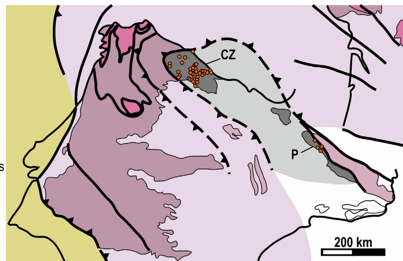
Fig. 1. A) Palaeogeographic reconstruction of the southern intertropical area of Pangea during mid-Carboniferous times (≈323 My) showing the location of the studied deposits with pseudomorphs after gypsum of the Variscan foreland basin (N Spain and S France), and potentially time equivalent gypsum strata of N Gondwana. Redrawn from Golonka et al. (1994), Scotese (2001) and Golonka (2002). B) Sketch showing the configuration of the Variscan massifs of Iberia prior to the opening of the Bay of Biscay (modified after Martínez Catalán et al., 2021) with location of the 67 studied outcrops. The boundary between the internal areas of the Variscan orogen and the foreland fold and thrust belt in the Pyrenees has been drawn according to García-Sansegundo et al. (2011).
