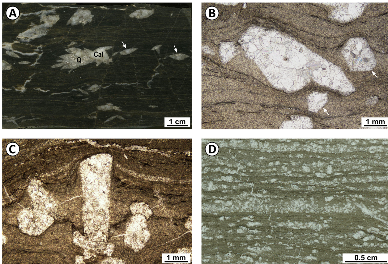
Fig. 8. A) Polished slab of facies C showing millimetre- to centimetre-sized lenticular calcite (Cal) and quartz (Q) pseudomorphs after gypsum (white arrows), locally forming centimetre-sized aggregates. B and C) Transmitted light microphotographs of facies C collected in the CZ (B) and Pyrenees (C). Pseudomorphs after gypsum show monoclinic prismatic and hexagonal sections (white arrows). D) Transmitted light photomicrograph of laminated calci-mudstones alternating with submillimetre-sized laminae of aggregates of calcite pseudomorphs after gypsum (facies D).
