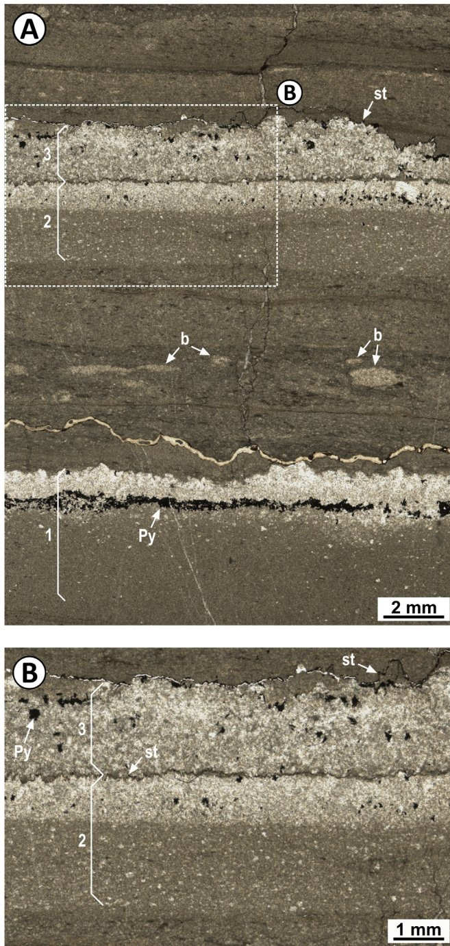
Fig. 10. A) Scanned thin section of facies E composed of laminae of calcite pseudomorphs after gypsum cumulates (1, 2, 3). Note the upward increase in the abundance of pseudomorphs within each pseudomorph-rich lamina. Pseudomorph lamina 1 shows a sharp upper contact and primary crystal terminations, which may have been formed by overgrowth of the cumulate crystals after their settling in the bottom. Py, pyrite replacements; st, stylolite; b, burrow. B) Photomicrograph showing cumulate cycles 2 and 3 from image A. The upper contact of the pseudomorph-rich lamina is stylolitized (st).
