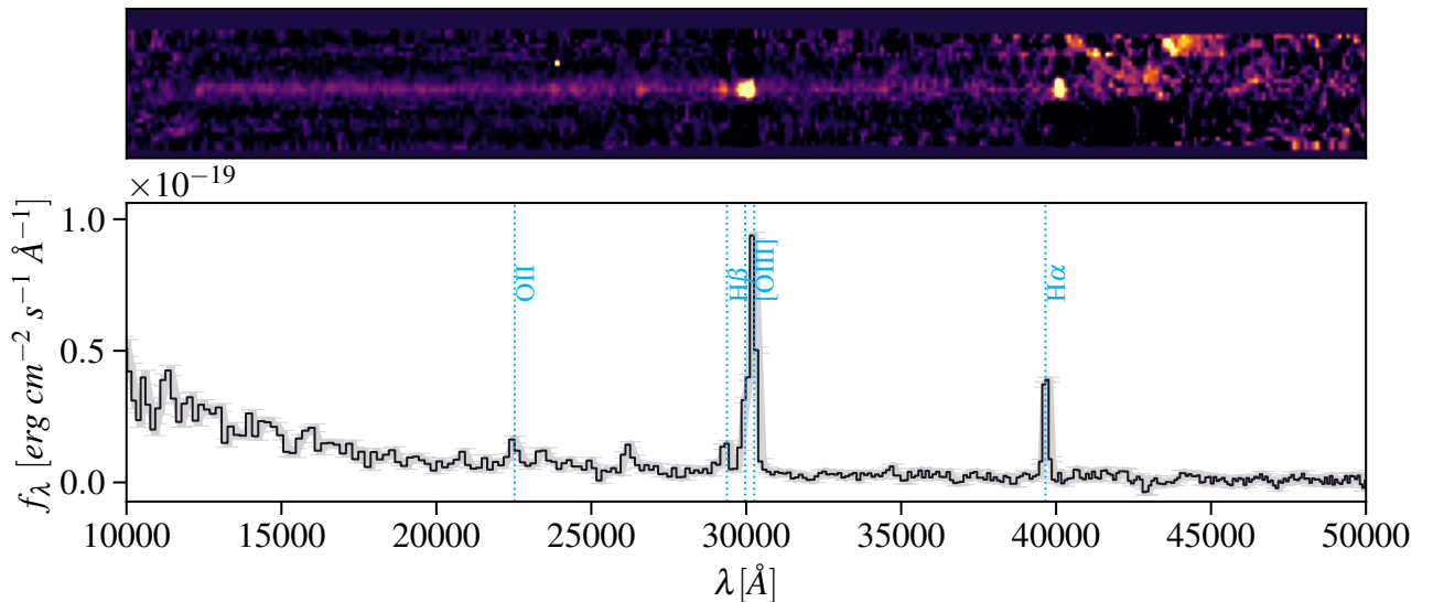
Fig. 2: Example 2D and 1D spectra of two representative galaxies in our sample. Top: 2D (top) and 1D (bottom) NIRSpect GLASS-JWST spectrum of 110000 at z = 5.765 (green for the G235H/F170LP and purple for the G395H/F290LP configuration) and 1\sigma uncertainty (gray). Bottom: 2D (top) and 1D (bottom) NIRSpect DDT spectrum of 150015 at z = 5.041 (black) and 1\sigma uncertainty (gray). Vertical dashed lines mark the position of well-detected rest-optical emission lines. The continuum emission is also detected as seen in the 2D spectrum. On the X-axis in the bottom panel, the observed wavelength ( \text{\AA} ) is reported.
