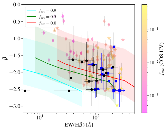
Fig. 6: \beta vs. rest-frame EW_0(\text{H}\beta) . Models are from Zackrisson et al. (2013) and simulate the expected trend for galaxies with an exponential declining SFR ( Z = 0.02 , solid lines) and various values of escape fractions. Symbols are as in Fig. 4.
