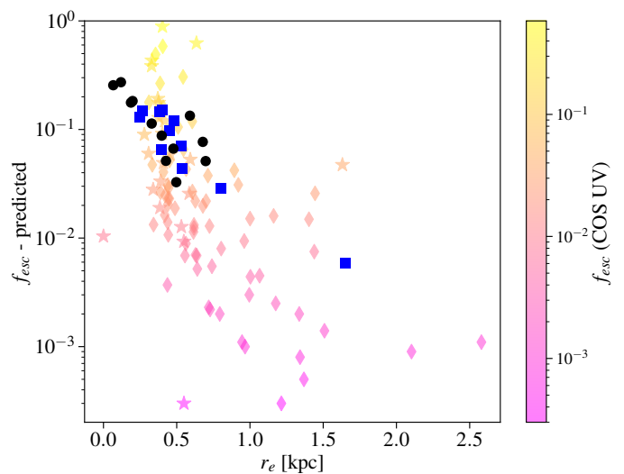
Fig. 8: Predicted f_{esc} vs. size r_e for our sample (blue and black symbols) and measured f_{esc} vs. size r_e from the literature. Symbols are as in Fig. 4.
