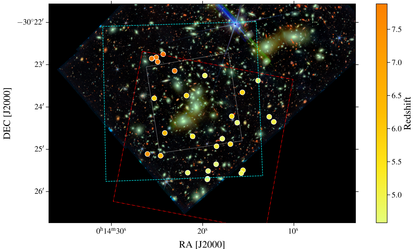
Fig. 1: Spatial location of the 29 selected sources, color coded by their spectroscopic redshift. They are superimposed on the RGB image of the UNCOVER program, made with NIRCam filters (blue = F115W + F150W, green = F200W + F277W, and red = F356W + F410M + F444W). The MUSE footprint is shown in white, the NIRSpec GLASS-JWST pointing is shown in cyan, and the NIRSpec DDT pointing is shown in red.
