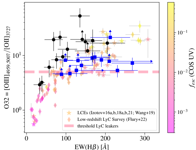
Fig. 4: O32 vs. rest-frame EW_0(H\beta) . Symbols are the same as in Figure 3. For reference, we also plot the galaxies at z = 0.3 - 0.4 from Flury et al. (2022) (diamonds) and the LCE from Izotov et al. (2016a,b, 2018a,b, 2021); Wang et al. (2019) (stars). Symbols are color coded as a function of their measured f_{esc} . The pink line ( O32 = 5 ) indicates the threshold for LCEs as predicted by Flury et al. (2022).
