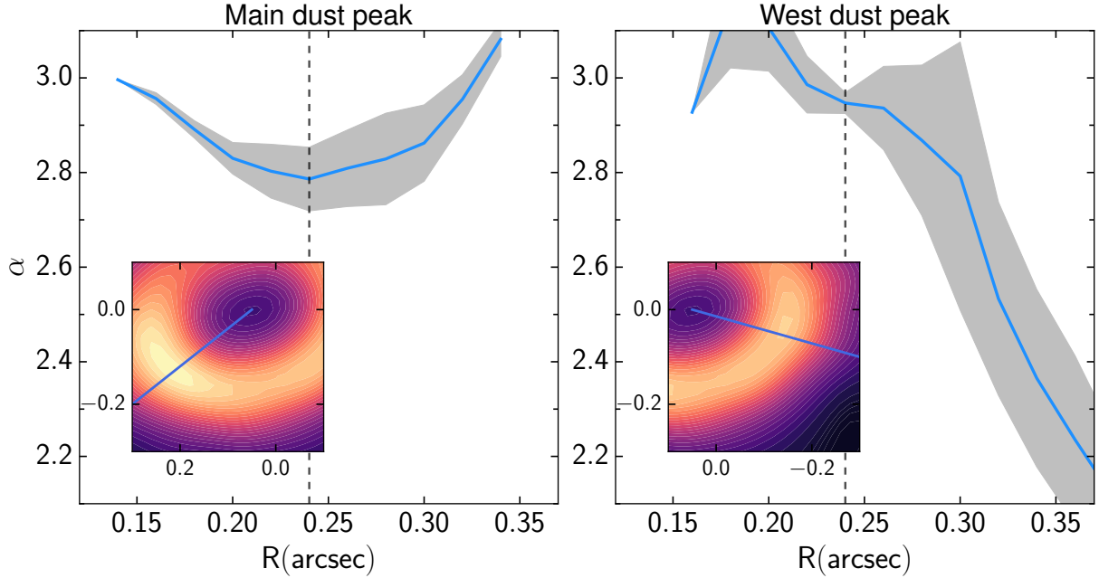
Figure 3. Dust spectral index profile of the dust emission peaks to the east (main, left ) and west ( right ). We plot the mean \alpha values within a beam as a function of distance from the center in arcseconds in blue while the gray-shaded regions indicate the dispersion around the mean. The vertical dash lines are placed at the rough locations of the peaks. Insets show the zoom-in view to the emission peak that is associated with each panel along with the radial cut that is shown by the blue line. The color scale in the insets is similar to Fig. 1.
