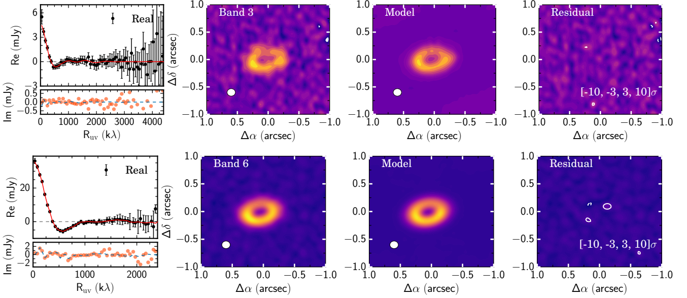
Figure 4. Best-fit symmetric Gaussian ring and two axisymmetric Gaussian ring model (GR2ARC) for both Bands 3 and 6. Top: The best-fit models for the Bands 3 data. Bottom: The best-fit model for the Bands 6 data. For each row, we show the binned visibilities, the original image, the model image, and the residual. For the residual image, the contours at -10, -3, 3, and 10 \sigma are indicated by the white lines.
