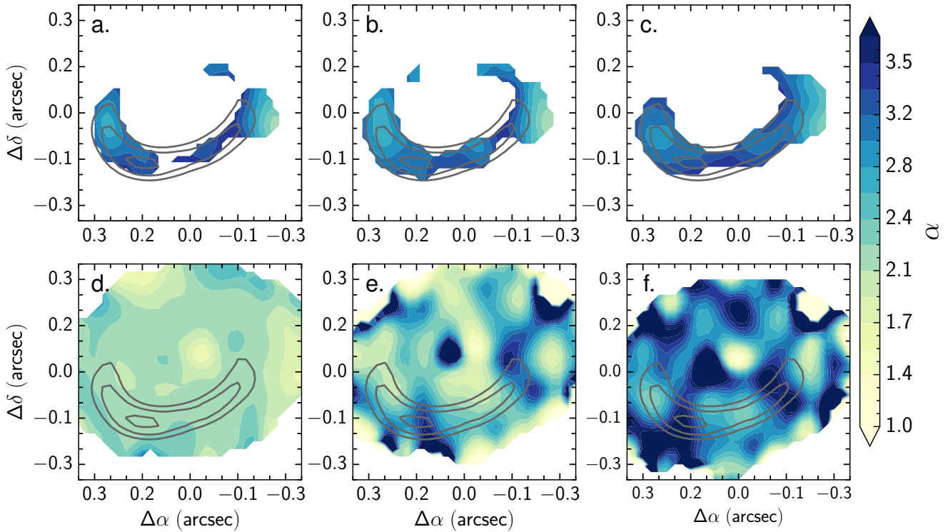
Figure 10. Spectral index maps of the primary disk. The top row (panels a, b, and c) shows the spectral index \alpha as derived in the image plane. Panel a is the spectral index map of the dust continuum images constructed with a tapering at 0''.09 with mfs and Hogbom deconvolver. Panel b shows the map using mtmfs and a taper while panel c shows the map in the case of the combination of tapering and a common beam of 0''.135 . The second row shows the spectral index map as produced by tclean mtmfs . Panels d, e, and f shows the \alpha map with increasing number of Taylor coefficients from 2 to 4. The gray contours indicate the dust continuum emission of the concatenated Bands 3 and 6 visibilities at 35, 40, and 45 \sigma .
