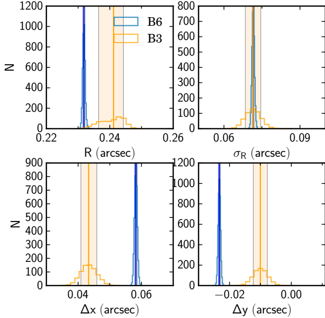
Figure 6. Similar to Fig. 5 but for the Gaussian Ring models.
