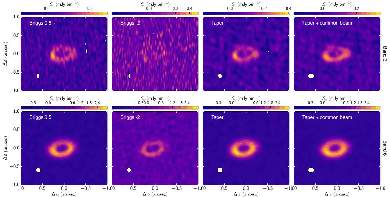
Figure 8. Dust continuum images of CIDA 9A. Top: Band 3 images. Bottom: Band 6 images. These images are cleaned with Briggs weighting. The tapered images (taper) are constructed with Briggs weighting of 0.5 and a tapering at 0''.08 . The panels that are indicated by 'Taper + common beam' are images that are restored with a common beam of 0''.135 .
