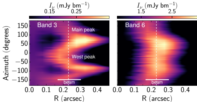
Figure 2. Profile of the dust emission in both Bands 3 (left) and 6 (right). The vertical dash line ( R = 0''.23 ) shows the location of the emission peaks in Band 6 that corresponds to the dust ring location of Long et al. (2018). The color scale is stretched differently with respect to Fig. 1 to highlight the dust emission peaks. The coordinates have been deprojected using the inclination and position angle obtained in Section 3.2.
