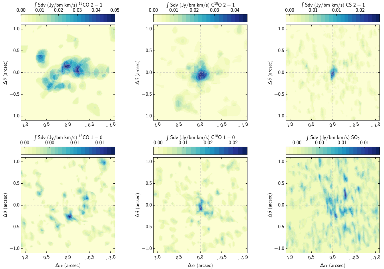
Figure 12. Similar to Fig. 11 with the addition of a velocity-based masking. We adopted the i = 47^\circ and a stellar mass of 0.7M_\odot .
