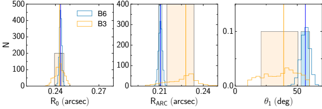
Figure 5. Comparison between the best-fit values of the GR2ARC model in Bands 3 and 6. The main parameters of the ring and the main arc are shown for simplicity. The mean and standard deviation for each of the parameters is plotted after taking into account the burn-in phase ( \sim 2000 ) and an acceptance rate of 15%. Band 6 results are shown in blue while Band 3 results are shown in orange.
