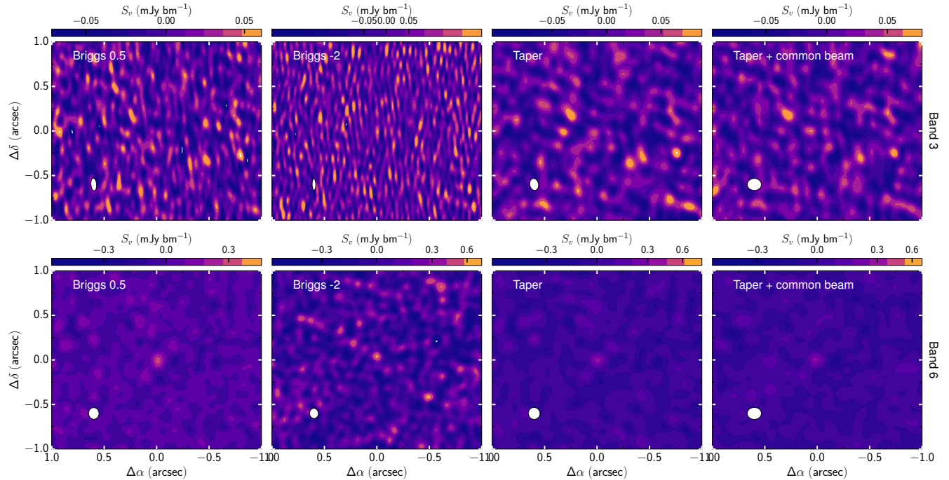
Figure 9. Similar to Fig. 8 for CIDA 9B.
