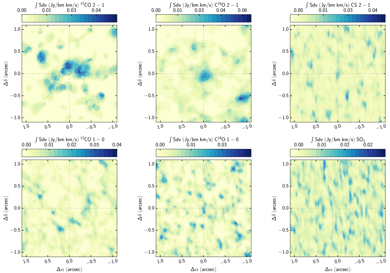
Figure 11. Integrated line maps (zeroth moment) of ^{13}\text{CO } J=2-1 , \text{C}^{18}\text{O } J=2-1 , \text{CS } J=2-1 , ^{13}\text{CO } J=1-0 , \text{C}^{18}\text{O } J=1-0 , and \text{SO}_2 \ 7_{3,5} - 8_{2,6} . The spectral cubes are integrated from 2 to 10 km/s. Only emissions above 2\sigma is considered.
