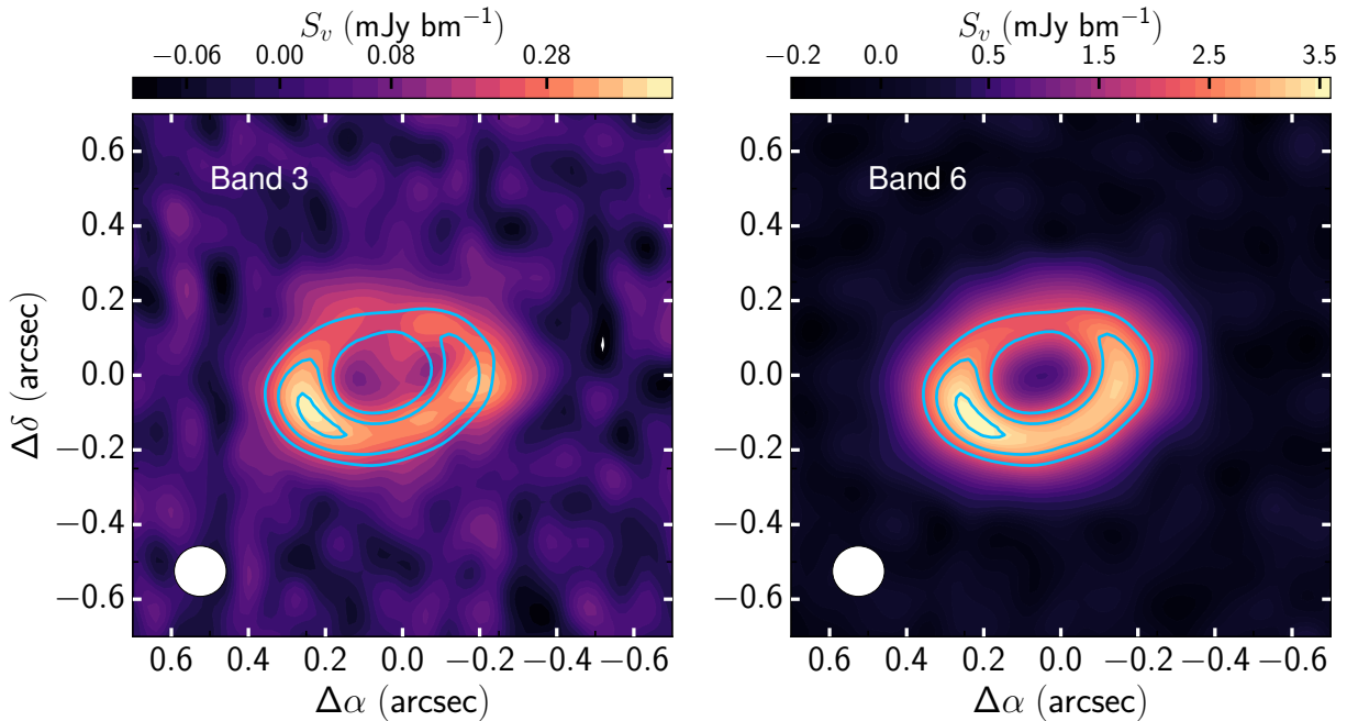
Figure 1. Dust continuum emission toward CIDA 9A in both Bands 3 ( Left ) and 6 ( Right ). The images are deconvolved using a tapering at 0''.09 and are restored with a 0''.135 \times 0''.135 beam. Blue contour lines indicate the 30 , 40 , and 50 \times \sigma levels of the Band 6 image to highlight the difference in the dust continuum peaks. The peak position in Band 3 is shifted clockwise with respect to the peaks that are seen in Band 6. The noise levels are tabulated in Table. 2.
