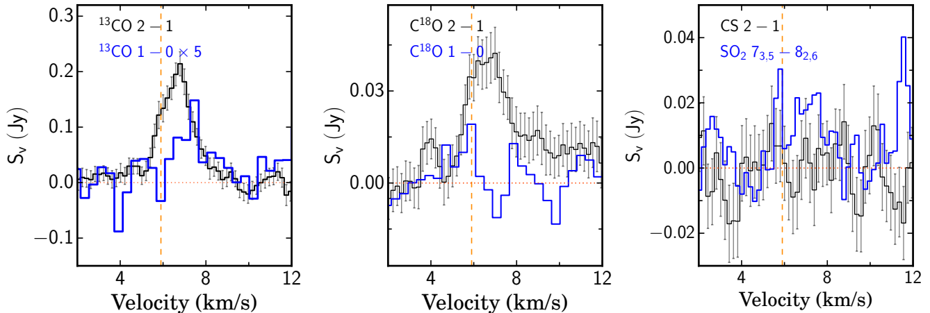
Figure 7. Molecular line profiles around CIDA 9A. As a reference, the ^{13}\text{CO} and \text{C}^{18}\text{O} J = 2 - 1 are shown in black lines in the left and middle panels. Their J = 1 - 0 counterparts are shown in blue. In addition, CS 2-1 and \text{SO}_2 7 3,5 - 8 2,6 are plotted in the right panel. These spectral lines are extracted with gofish adopting the stellar and disk parameters of Rota et al. (2022).
