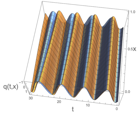
(a) Comparison of the numerical solution (orange) with the non-relativistic solution (blue) as the frequency and phase are set as constant. Adapted from Ref. [16] with permission of the Institute of Physics Publishing.
