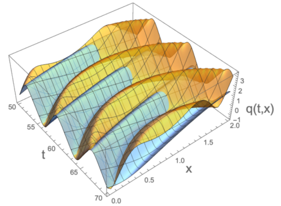
(b) A plot showing the variation from the numerical solution (orange) and the non-relativistic solution (blue) and highlighting the behavior of the system far from the origin
