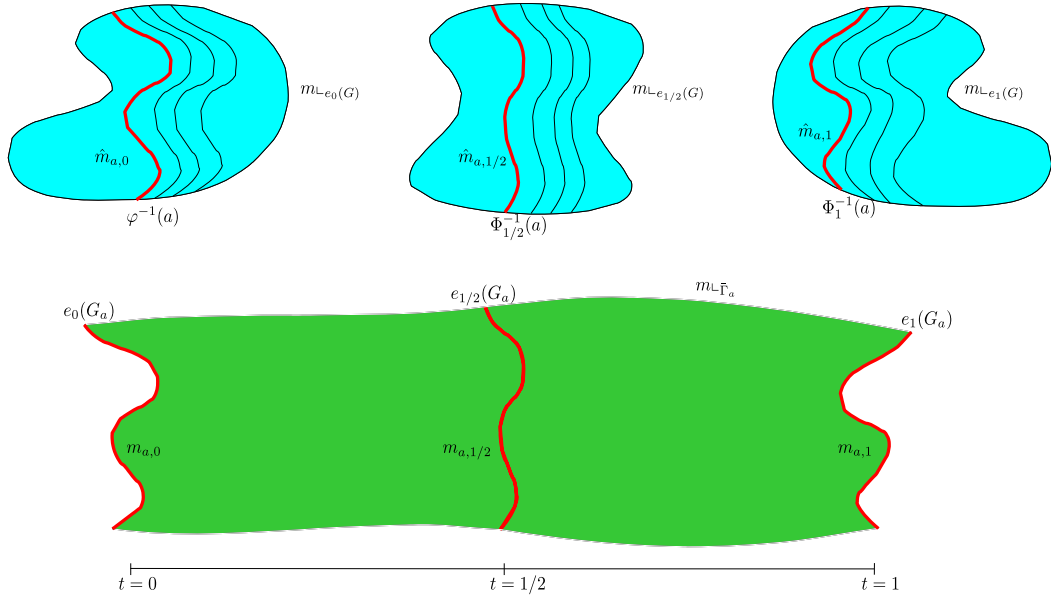
Figure 1: Above and below the disintegration with conditional \hat{m}_{a,t} and m_{a,t} , respectively
