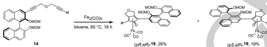
Scheme 5. Carbonylative cyclization/complexation of diynes 9-12 and 14 .
