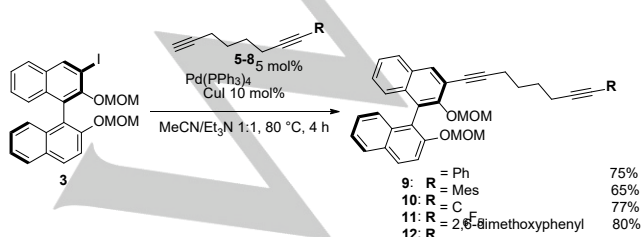
Scheme 3. A: Synthesis of mono-substituted 1,7-octadiyne derivatives 5-8 ; B: Synthesis of C 1 -symmetric diyne precursors 9-12 .
