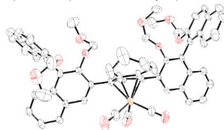
Figure 2. ORTEP representation of the molecular structure of complex 1a . Thermal ellipsoids are represented at the 50% probability level. Color code: C (black), O (red) and Fe (orange).
