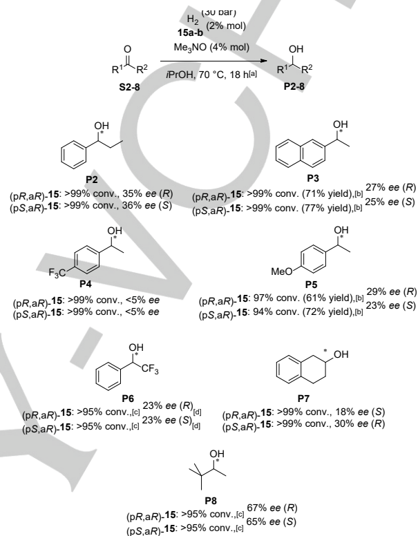
Scheme 7. Substrate screening for the AH of ketones catalyzed by CICs (p R ,a R )- 15 and (p S ,a R )- 15 . [a] Reaction conditions: Substrate/Pre-cat./Me 3 NO = 100:2:4, T = 70 °C, P H 2 = 30 bar, C 0,S1 = 1.43 M. Conversions were determined by chiral GC analysis. [b] Yield determined by 1 H-NMR analysis. [c] Conversion determined by 1 H-NMR analysis. ee's were determined by GC analysis with a chiral capillary column (see Supporting Information). [d] ee determined by chiral HPLC analysis.
