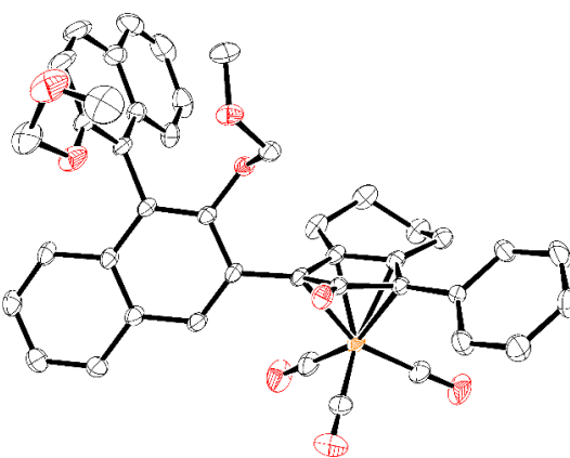
Figure 3. ORTEP representation of the molecular structure of complex (pS,aR)- 15 . Thermal ellipsoids are represented at the 50% probability level. Color code: C (black), O (red) and Fe (orange).
