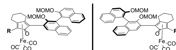
Figure 1. Cyclopentadienone complexes featuring a stereogenic plane. CIC = (cyclopentadienone)iron complex.
