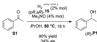
Scheme 6. Test of the AH of acetophenone ( S1 ) promoted by complex (p R ,a R )- 15 at 50 °C.
