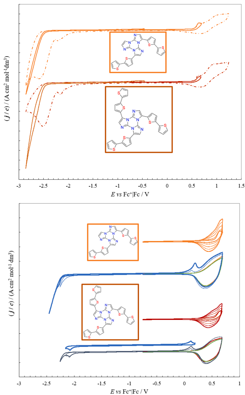
Fig. 8. Comparative synopses of normalized CV features on GC electrode for (2\text{-biTh})_2\text{TT} and (2\text{-biTh})_3\text{TT} with the same operating protocols, in \text{CH}_2\text{Cl}_2 with 0.1 M \text{TBAPF}_6 supporting electrolyte. Top: monomer CV features at 0.2 V/s. Bottom: potentiodynamic electrooligomerizations at 0.2 V/s scan rate (with I, III, VI, IX, XII cycles reported), followed by stability cycles in monomer-free solution (V cycle reported in green over the last deposition cycle) and by potential cycle widening towards more negative potentials enabling to highlight charge trapping effects (reported in blue).
